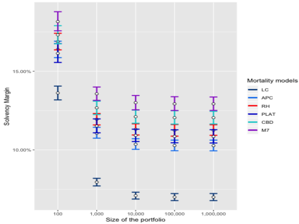
Figure 3.4.8: Solvency margins for different stochastic mortality models for d = 5 and T = n with 95% confidence intervals
