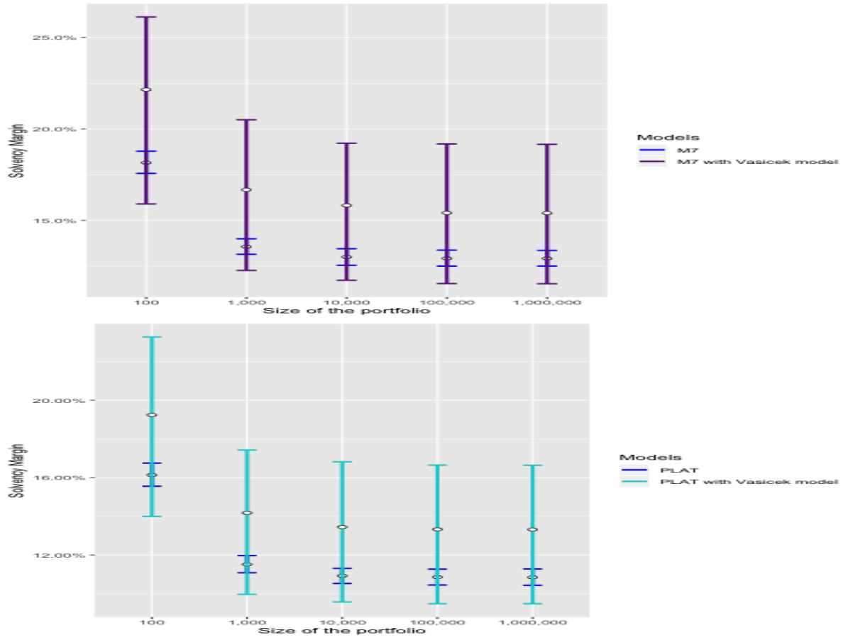
Figure 3.5.3: Solvency margins for different stochastic mortality models combined with Vasicek stochastic interest rate model with \sigma = 0.2 for d = 5 and T = n with 95% confidence intervals.
