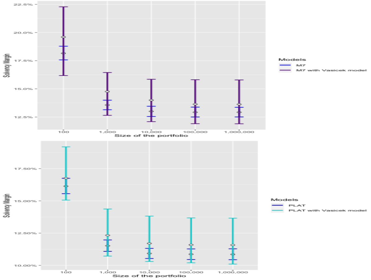
Figure 3.5.1: Solvency margins for different stochastic mortality models combined with Vasicek stochastic interest rate model with \sigma = 0.05 for d = 5 and T = n with 95% confidence intervals.
