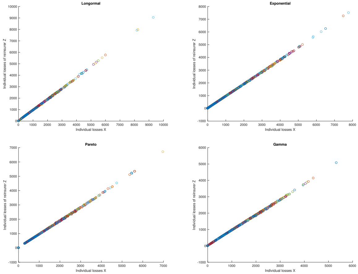
Figure 2.4.1: Empirical solutions of z_{kr} , 1 \leq k \leq m for proposition 2.3.1 for different distributions.
