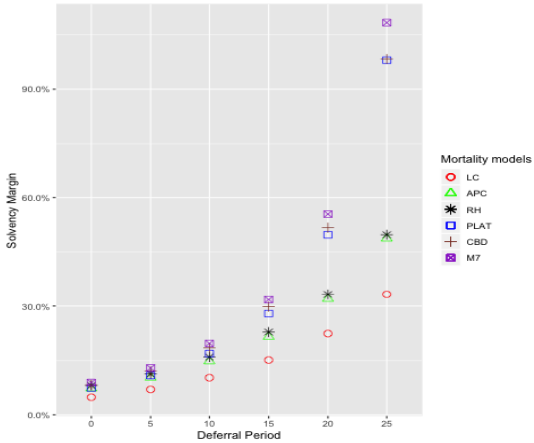
Figure 3.4.9: Solvency margins for different stochastic mortality models and different deferred periods when T = n
