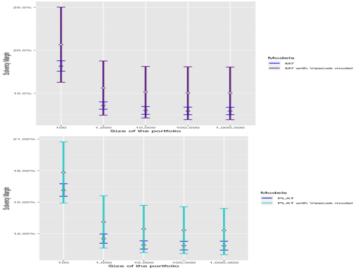
Figure 3.5.2: Solvency margins for different stochastic mortality models combined with Vasicek stochastic interest rate model with \sigma = 0.1 for d = 5 and T = n with 95% confidence intervals.
