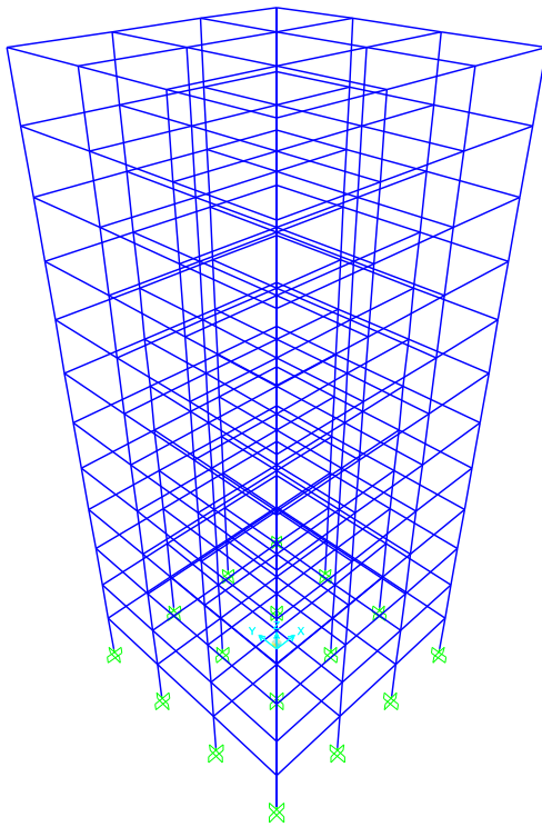
Fig. 7. 3D view of the 12-storey concrete frame.
