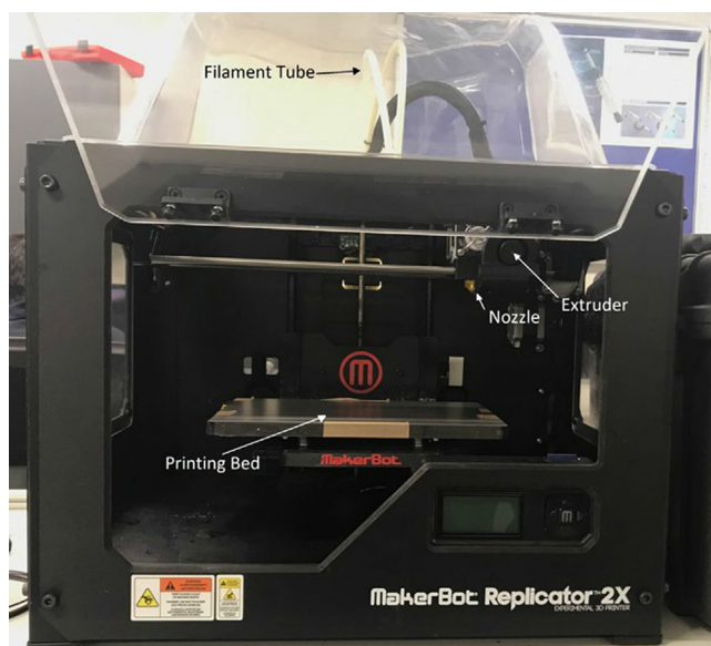
Fig. 3. Labelled MakerBot Replicator 2 machine used for 3D printing.
