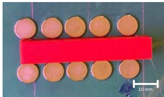
Fig. 4. PLA printed cuboid with five N52 magnets of opposite polarity on each side of the cuboid.
