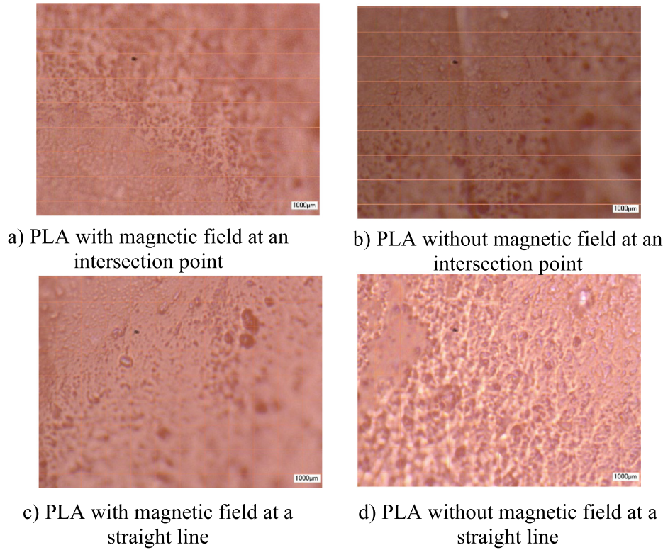
Fig. 10. PLA samples with x5000 magnification.
