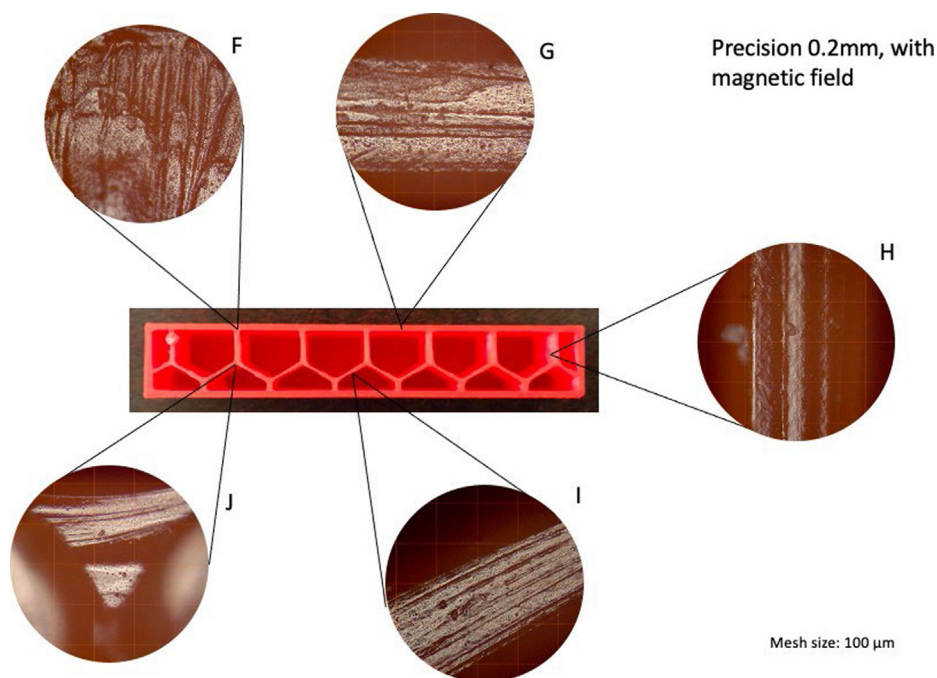
Fig. 9. Printed PLA sample with microscopy - F: Side and boundary, G: Side and hole, H: Straight line, I: Tilted line and J: Intersection.
