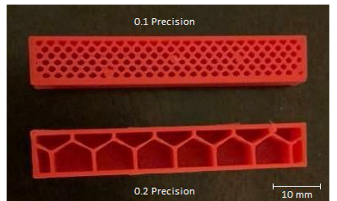
Fig. 2. PLA samples of different precisions: The top with high precision 0.1 mm and the bottom with standard precision 0.2 mm.
