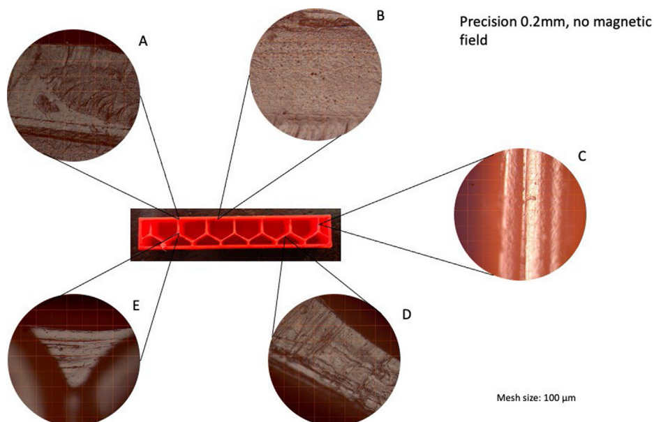
Fig. 8. Printed PLA sample with microscopy - A: Side and boundary, B: Side and hole, C: Straight line, D: Tilted line and E: Intersection.
