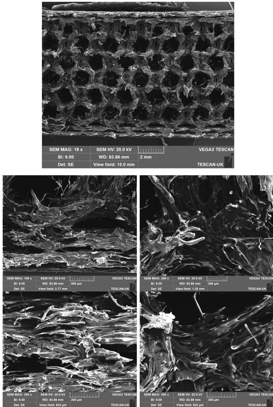
Fig. 11. Typical SEM images of carbon composite Onyx subjected to in-situ magnetic field during 3D printing.
