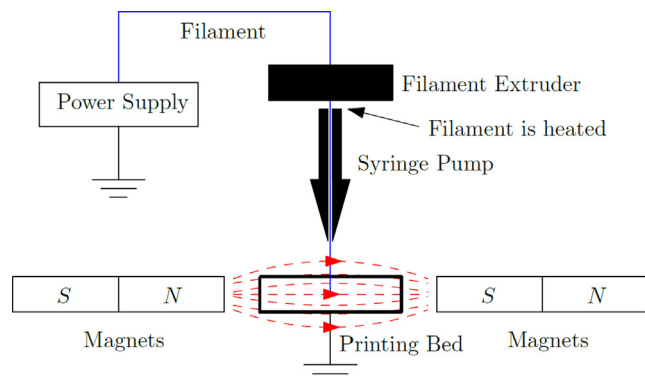
Fig. 1. Diagram of the front view of FDM technique with magnets on either side of the printing bed, where the red dashed line represents the magnetic field going from the north to south pole. (For interpretation of the references to colour in this figure legend, the reader is referred to the web version of this article.)
