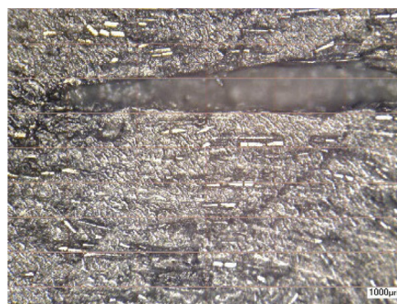
b) Polished onyx subjected to two rows of magnets through magnification of X500
