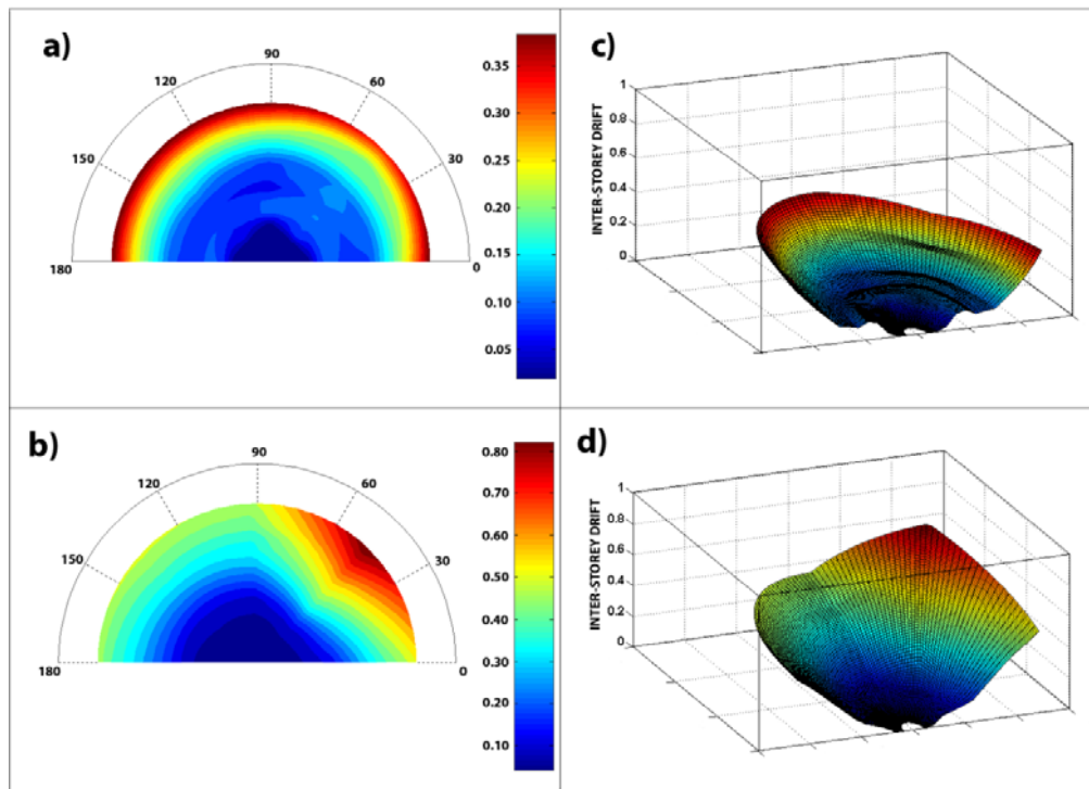
Figure 13. IM-incident angle- EDP plots. a) Contour EDP plot for the fault-parallel component b) Contour EDP plot for the fault-normal component c) EDP response surface for the fault-parallel component d) EDP response surface for the fault-normal component.
