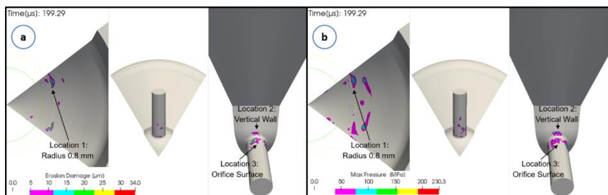
Figure 6. 8. Spatial distribution of potential cavitation damage. (a) Erosion damage prediction [ \mu\text{m} ]. (b) Maximum wall collapse pressures recorded at the walls [MPa].
