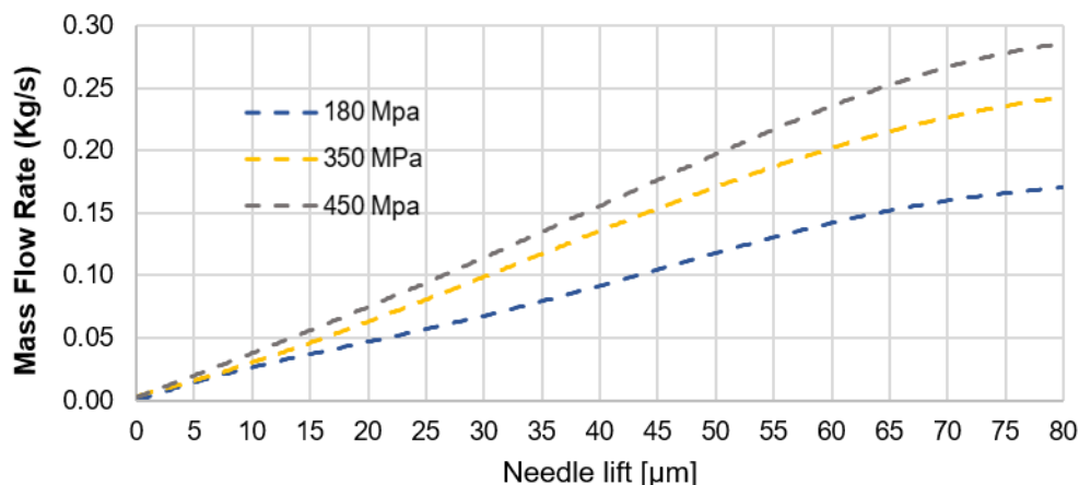
Figure 4. 3. Mass flow rate at the orifice exit for all cases.
