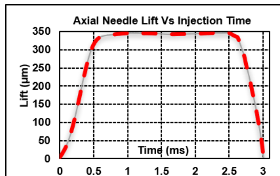
Figure 6. 2. Needle motion of the injector.
