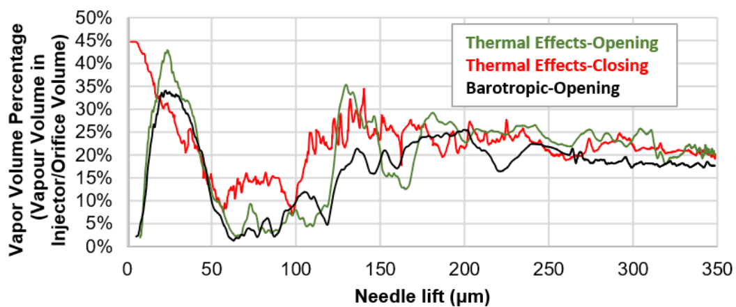
19 20 Figure 3. 10. Vapor volume fraction in the injector volume during the opening and closing 21 phase of the needle valve. Before 150\mu\text{s} ( 60\mu\text{m} ) and after 2950\mu\text{s} ( 63\mu\text{m} ) the vapor volume 22 is normalised with the total injector's sac and orifice volumes. During these times,
