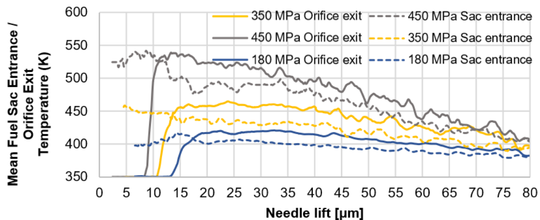
Figure 4. 8. Temporal evolution of fuel temperature at the exit of the injector's orifice (solid lines) and at the sac entrance (dashed lines); lift increase from 0 \mu\text{m} to 80 \mu\text{m} during the plotted time.
