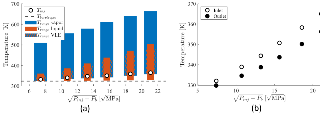
Figure 5. 7. (a) Variation in temperature for the liquid, vapor and vapor-liquid equilibrium (VLE) phases versus the square root of pressure drop. As a reference, both the injection temperature and the reference temperature used in the barotropic approach are included. (b) Average temperatures at the orifice inlet and outlet slices.
