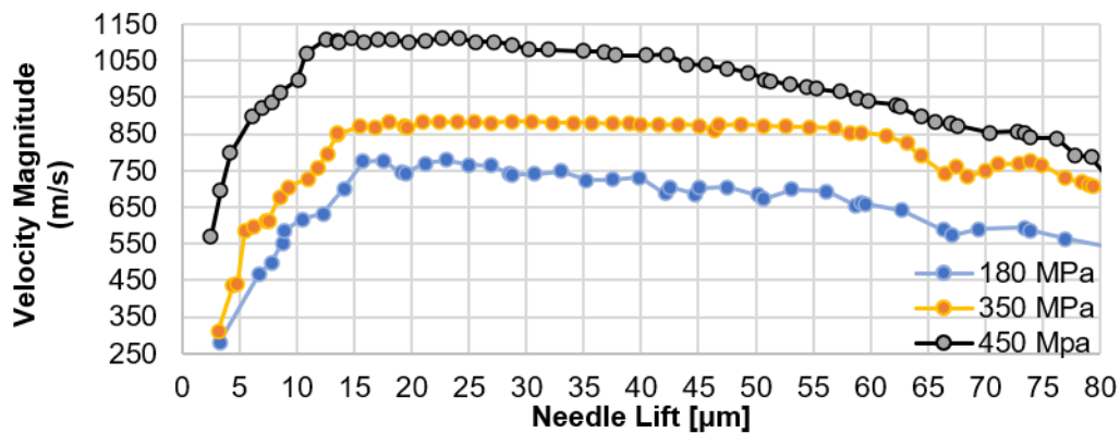
Figure 4. 4. Temporal evolution of maximum velocity magnitude at the narrowest point at the needle seat passage; lift increase from 0 \mu\text{m} to 80 \mu\text{m} during the simulated time.
