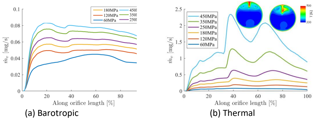
Figure 5. 14. Time-averaged vapor mass flow rate along the orifice length for both (a) barotropic and (b) thermal cases, for all injection pressures simulated. Two insets of the temperature distribution are added to the thermal case, corresponding to locations of high
