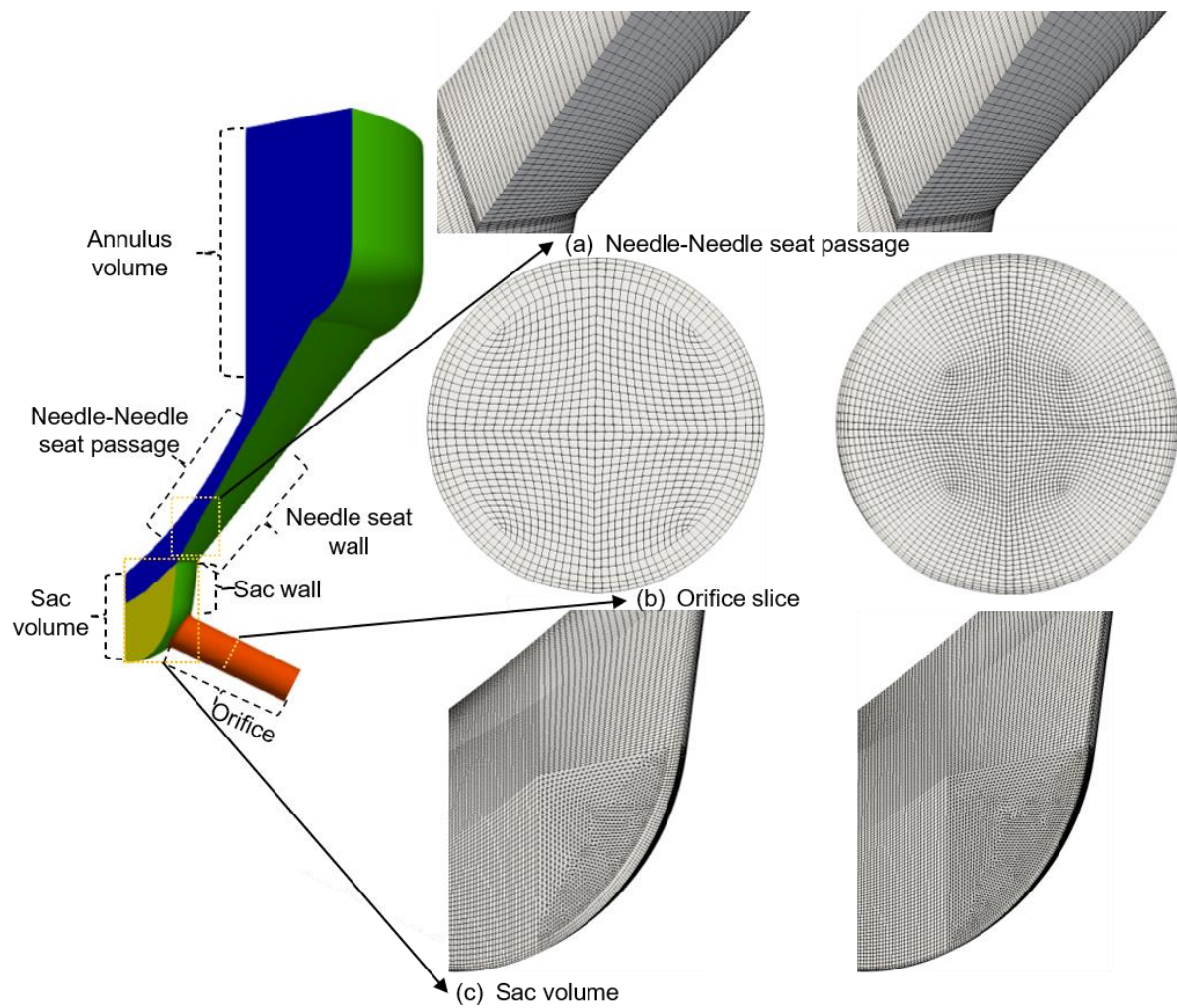
2 Figure 4. 1. Naming convention of injector surfaces and 3D view of the computational 3 domains at 70 \mu\text{m} needle lift for different injection pressures.
