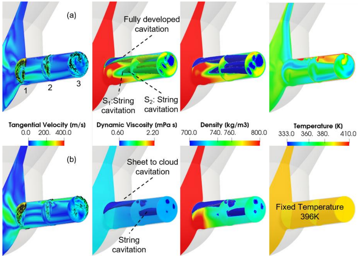
Figure 3. 20. Instantaneous tangential velocity, dynamic viscosity, density and temperature distribution on slices normal to the orifice and at the midplane of the injector, at time instant 248\mu\text{s} ( 132\mu\text{m} needle lift) using (a) full thermodynamic model and (b) barotropic model. Instantaneous tangential velocity, dynamic viscosity, density and temperature distribution on slices normal to the orifice and at the midplane of the injector, at time instant 248\mu\text{s} ( 132\mu\text{m} needle lift). The vapor volume fraction \alpha = 0.01-1.0 is coloured by the dynamic viscosity and by the density.
