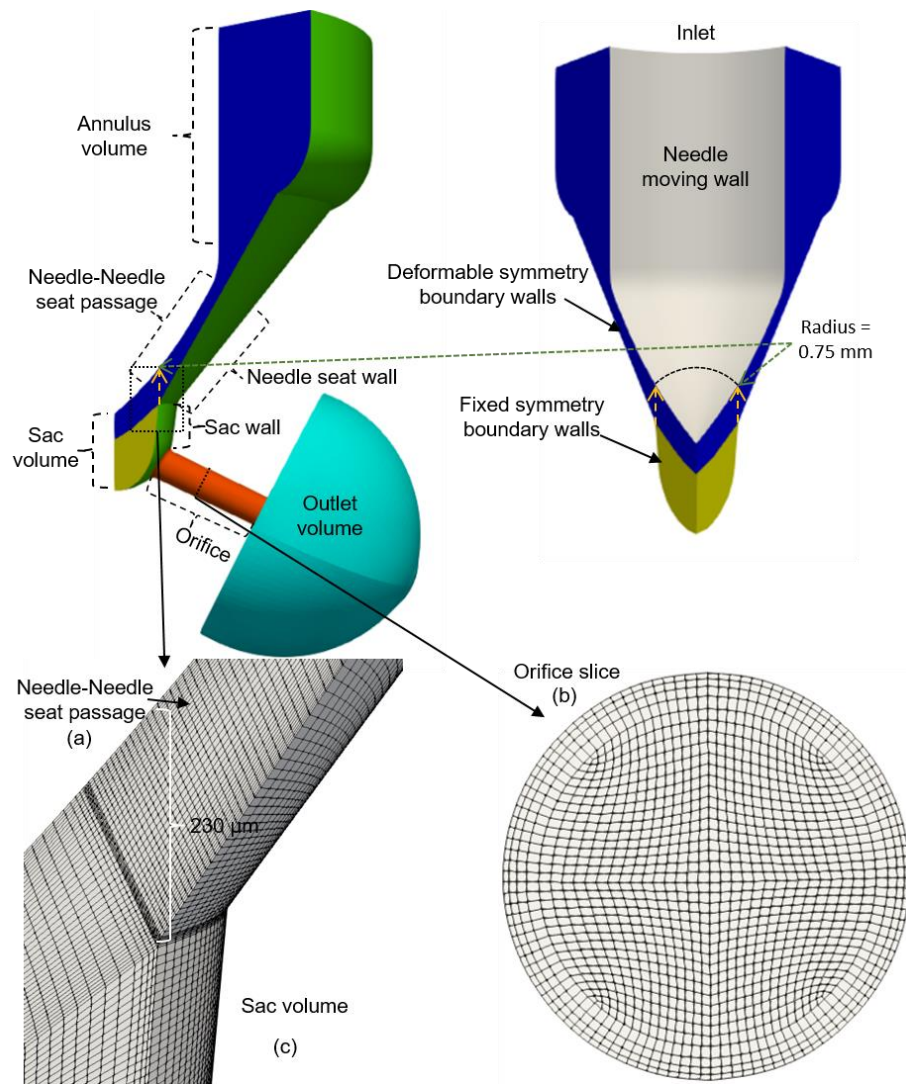
Figure 3. 5. Naming convention of injector surfaces (top) and 3D view of the computational domain at 70 \mu\text{m} needle lift (bottom).
