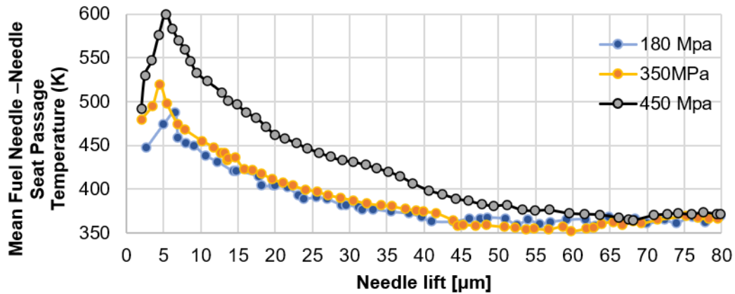
Figure 4. 13. Temporal evolution of fuel temperature at the needle- needle seat passage; lift increase from 0 \mu\text{m} to 80 \mu\text{m} during the plotted time.
