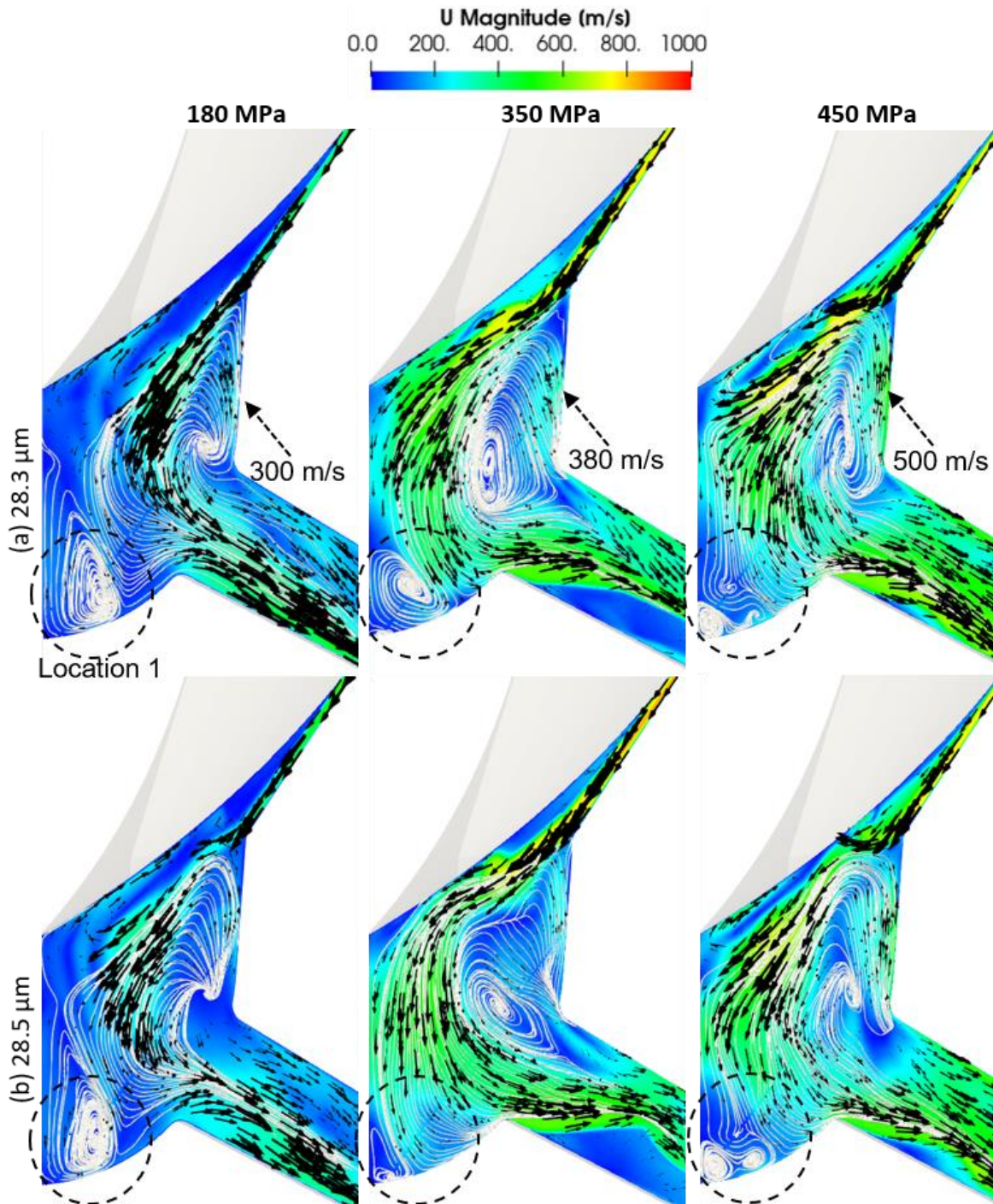
Figure 4. 11. Snapshots of the predicted flow field and flow streamlines at selected time instants (a) and (b).
