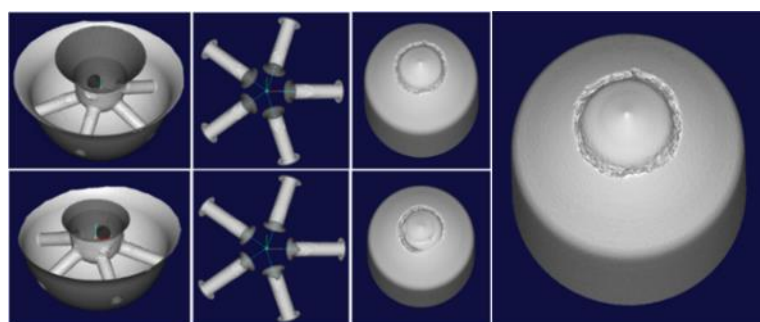
Figure 6. 5. From left to right. Erosion details at various locations. Analysis of the needle surface erosion pattern using image processing tool.
