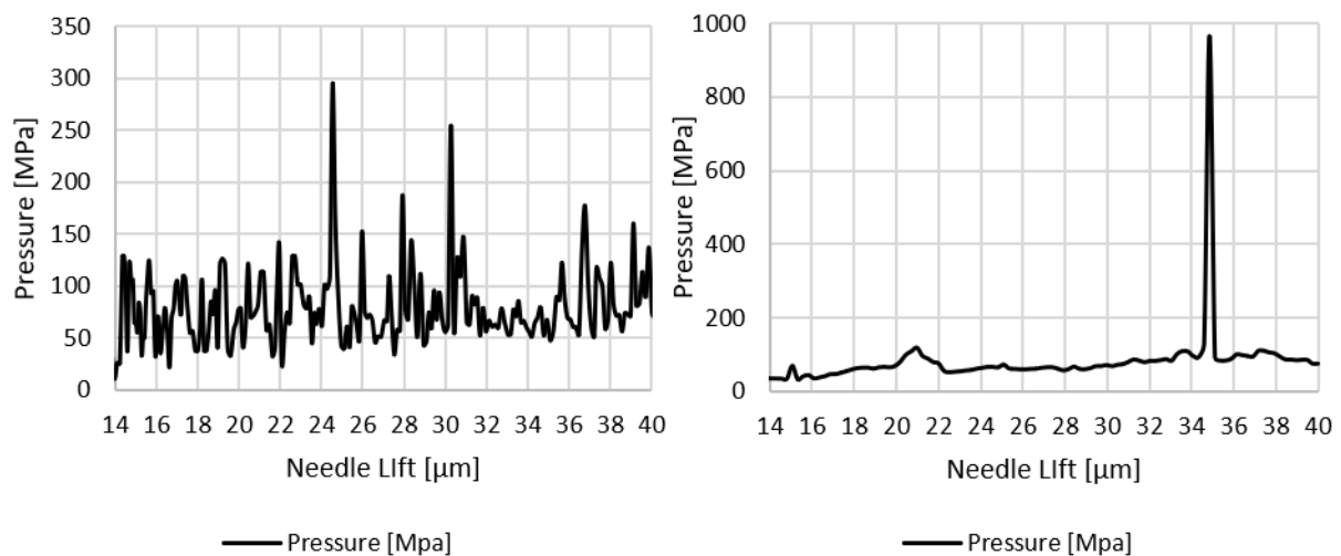
Figure 3. 18. Peak collapse detector pressures during the needle opening phase (right) and during the needle closing phase (left), recorded during the period when the needle lift moves between 14 \mu\text{m} to 40.
