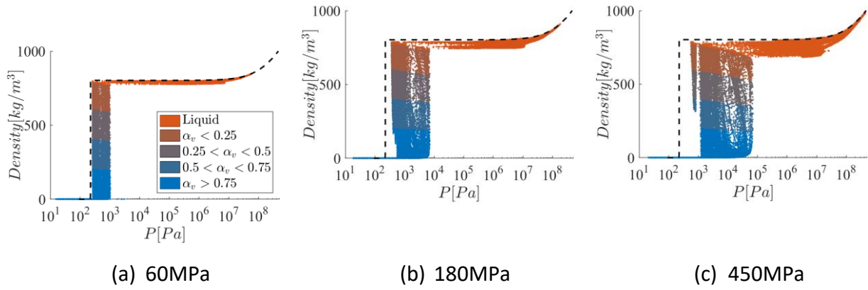
Figure 5. 9. Predicted single-time instance of logarithm of pressure versus density values over the whole computational domain for three injection pressures; the curve for the barotropic evolution (dashed line) is indicated. The colour of the symbols shows their value of the vapor volume fraction within different ranges.
