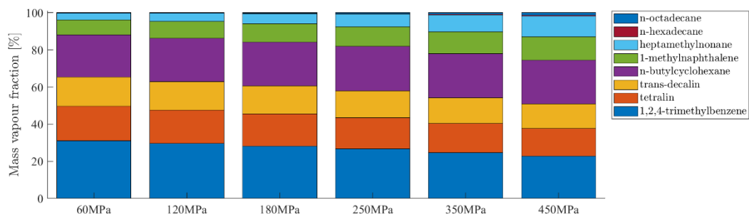
Figure 5. 19. Time-averaged predictions for the vaporised mass composition of the vapor cloud, in a stacked fashion, for all injection pressures.
