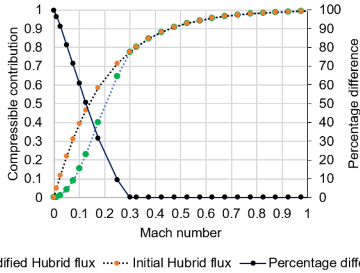
Figure 3. 2: Illustration of the contribution of the weighted term \beta (Eq(25) [185] ) on the interface pressure as described in Eq(22).
