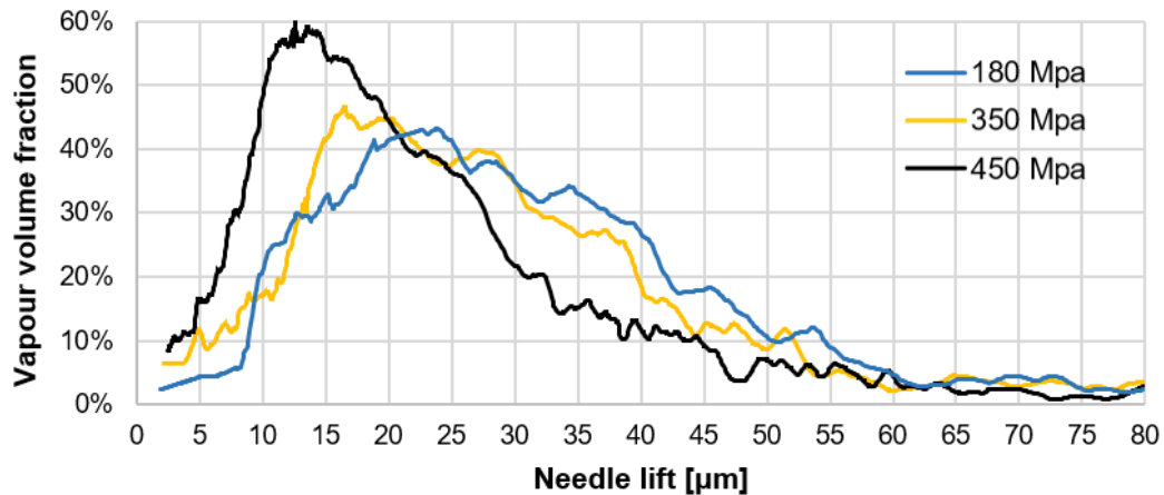
Figure 4. 5. Vapor volume fraction in the injector volume during the early opening phase of the needle valve. The vapor volume is normalised with the sum of the needle seat passage volume below the narrowest point, the injector's sac and orifice volumes. It is noted that at zero needle lift the sac volume is 3.1 times larger than the volume of the orifice.
