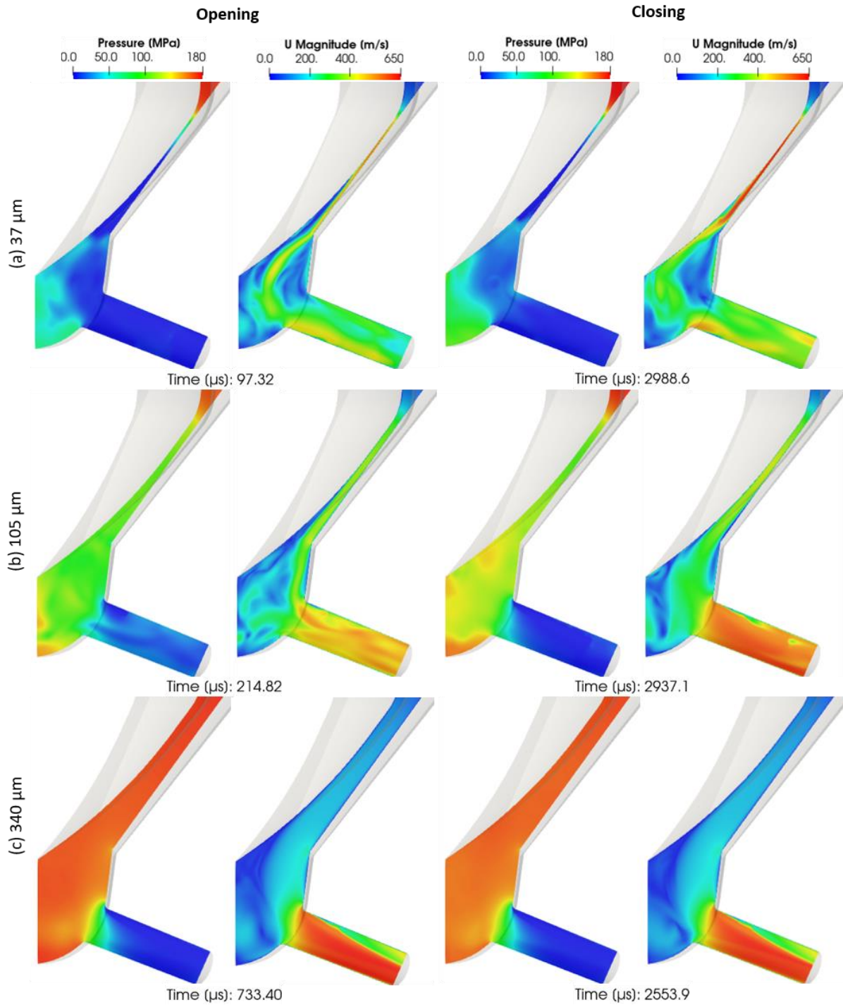
Figure 3. 14. Snapshots of instantaneous pressure and velocity magnitude at time instances corresponding to (a) 37 \mu\text{m} , (b) 105 \mu\text{m} and (c) 340 \mu\text{m} .
