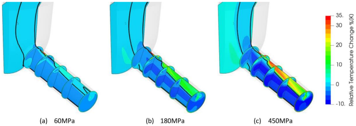
Figure 5.7. Predicted time-averaged temperature change with respect to the injection temperature, defined as (T - T_{inj})/T_{inj} * 100 , when thermal effects are considered. The injection temperature for each case is shown in Table 3. A solid thick black line is plotted in the longitudinal slice where T = T_{inj} , thus all points inside this iso-line show cooling and those outside show heating. Results are shown on different slices at the sac volume and orifice for three injection pressures.
