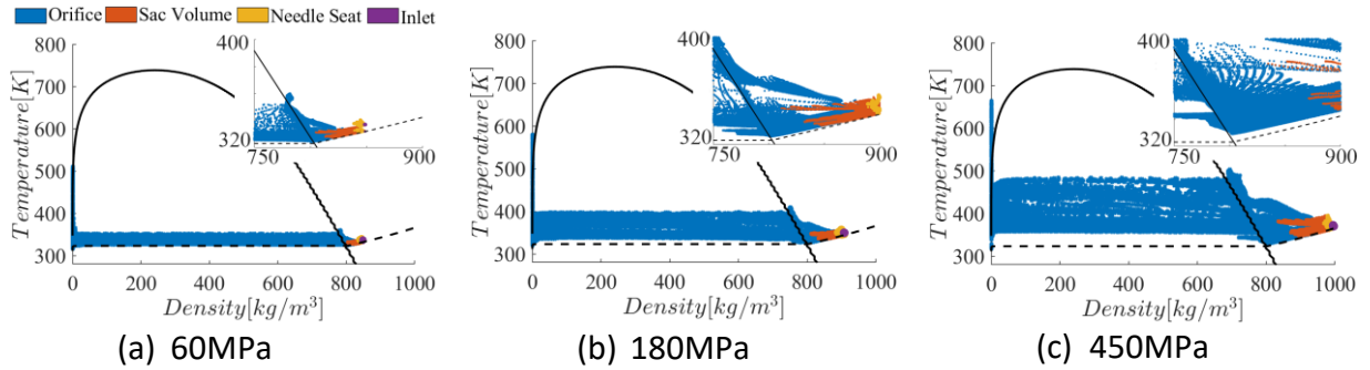
Figure 5. 8. Predicted time-averaged density-temperature values over the whole computational domain for three injection pressures. The saturation curve for the multicomponent Diesel surrogate (solid line) and the isentropic approach (dashed line) are indicated. The colour of the symbols distinguishes the zone in the injector they correspond to. As an inset, the distribution of point close to the saturation curve is added.
