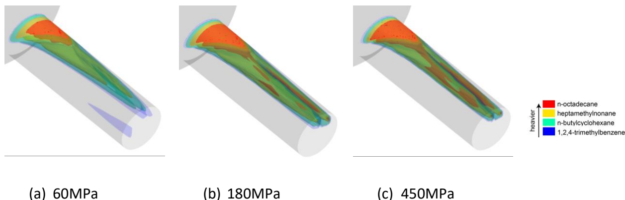
Figure 5. 18. Effect of the injection pressure on partial vaporisation of selected components of the Diesel surrogate simulated. Results are time-averaged and thermal effects are considered.
