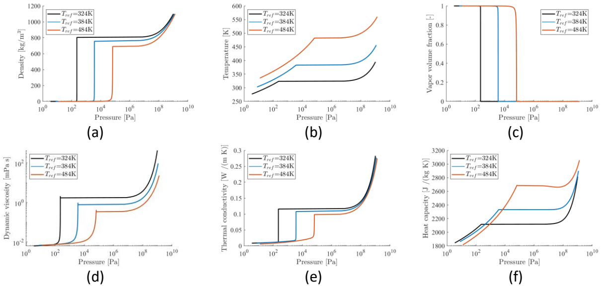
Figure 5. 2. Thermodynamic data following an isentropic expansion of the Diesel surrogate.
