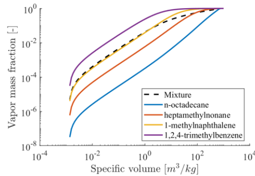
Figure 5. 17. Vapor mass fraction of representative components of the fuel surrogate (the heaviest, lightest and two intermediate) as a function of specific volume for a OD expansion of the fuel at 350K.
