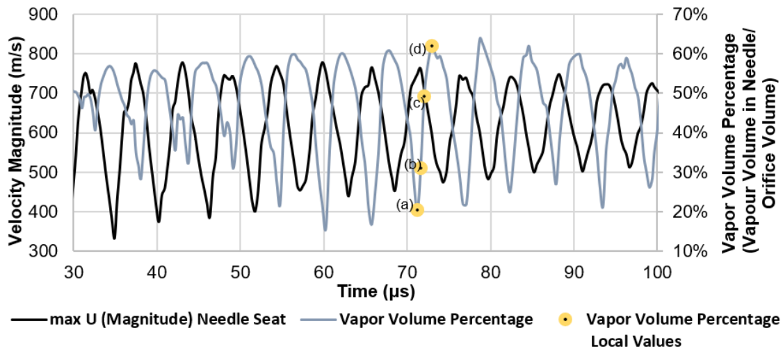
Figure 3. 8. Temporal evolution of maximum velocity magnitude and vapor volume percentage at the narrowest point at the needle seat passage; lift increase from 12 \mu\text{m} to 35 \mu\text{m} during the plotted time. The points (a) to (d) are indicated as a reference to following figures.
