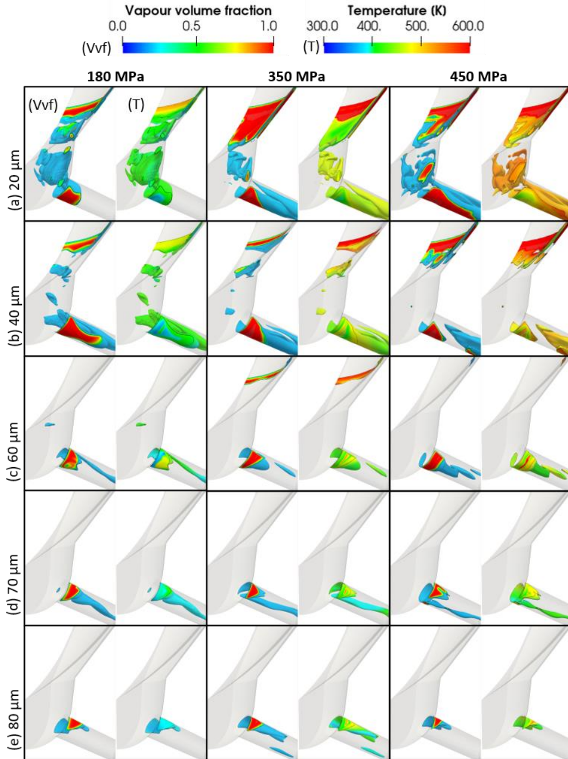
Figure 4. 6. Snapshots of cavitation formation coloured by both the vapor volume fraction and temperature during the opening of the needle valve. The time instants correspond to needle lifts of: (a) 20 \mu\text{m} , (b) 40 \mu\text{m} , (c) 60 \mu\text{m} , (d) 70 \mu\text{m} and (e) 80 \mu\text{m} .
