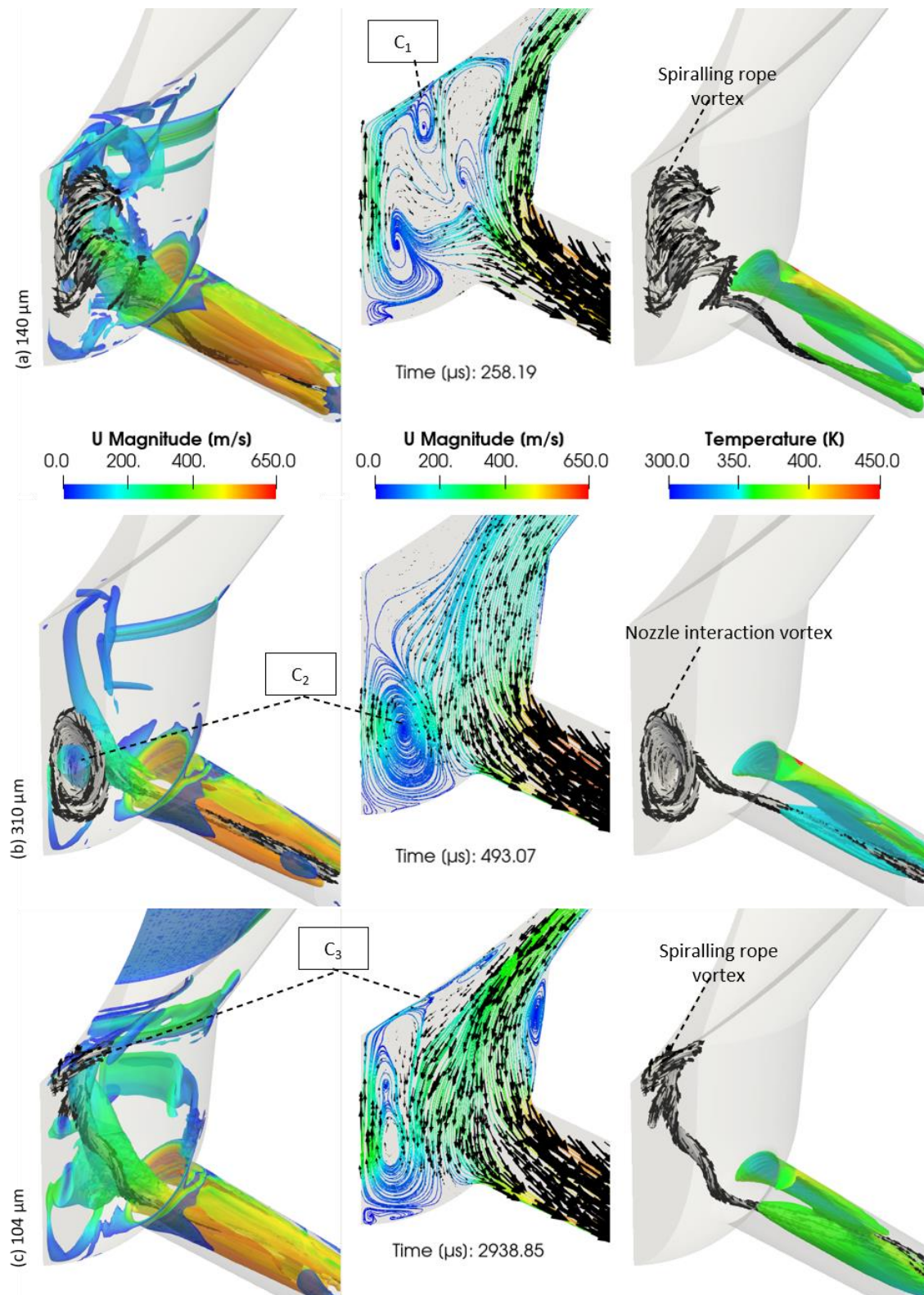
Figure 3. 13. 3D visualization of a representative vapor and vortex shedding cycle at time instances correspond to (a) 140 \mu\text{m} opening phase, (b) 310 \mu\text{m} opening phase and (c) 104 \mu\text{m} closing. First column: The iso-surfaces of q criterion with q = 2.2 \times 10^{12} are colored by the velocity magnitude; Second column: flow streamlines at the midplane of the injector coloured by the velocity magnitude; Third column: vapor volume fraction coloured by fuel temperature and flow streamlines.
