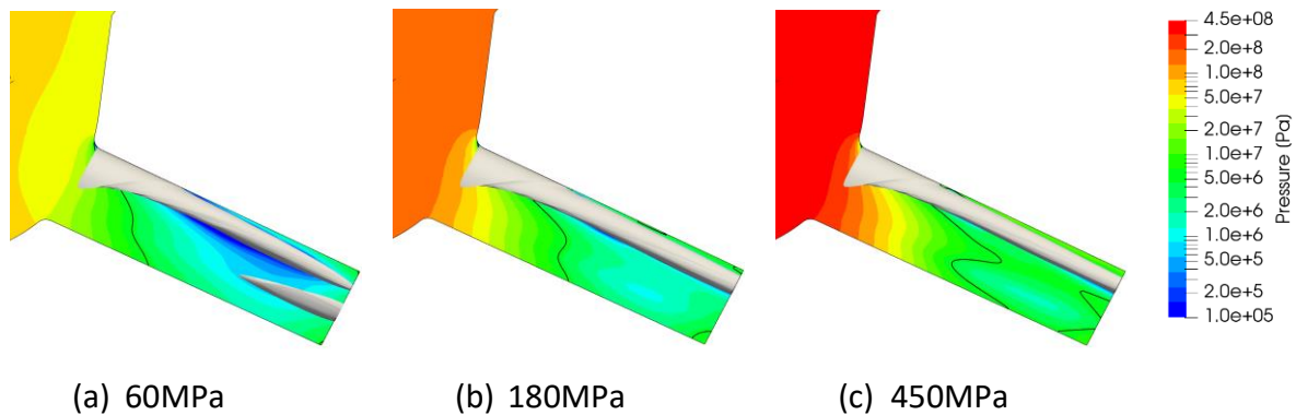
Figure 5. 11. Predicted time-averaged pressure on a longitudinal slice of the injector. A solid black iso-line at 5MPa, the back pressure, and the iso-surface for 50% vapor volume fraction have been included. The colour map is in logarithmic scale and thermal effects are considered.
