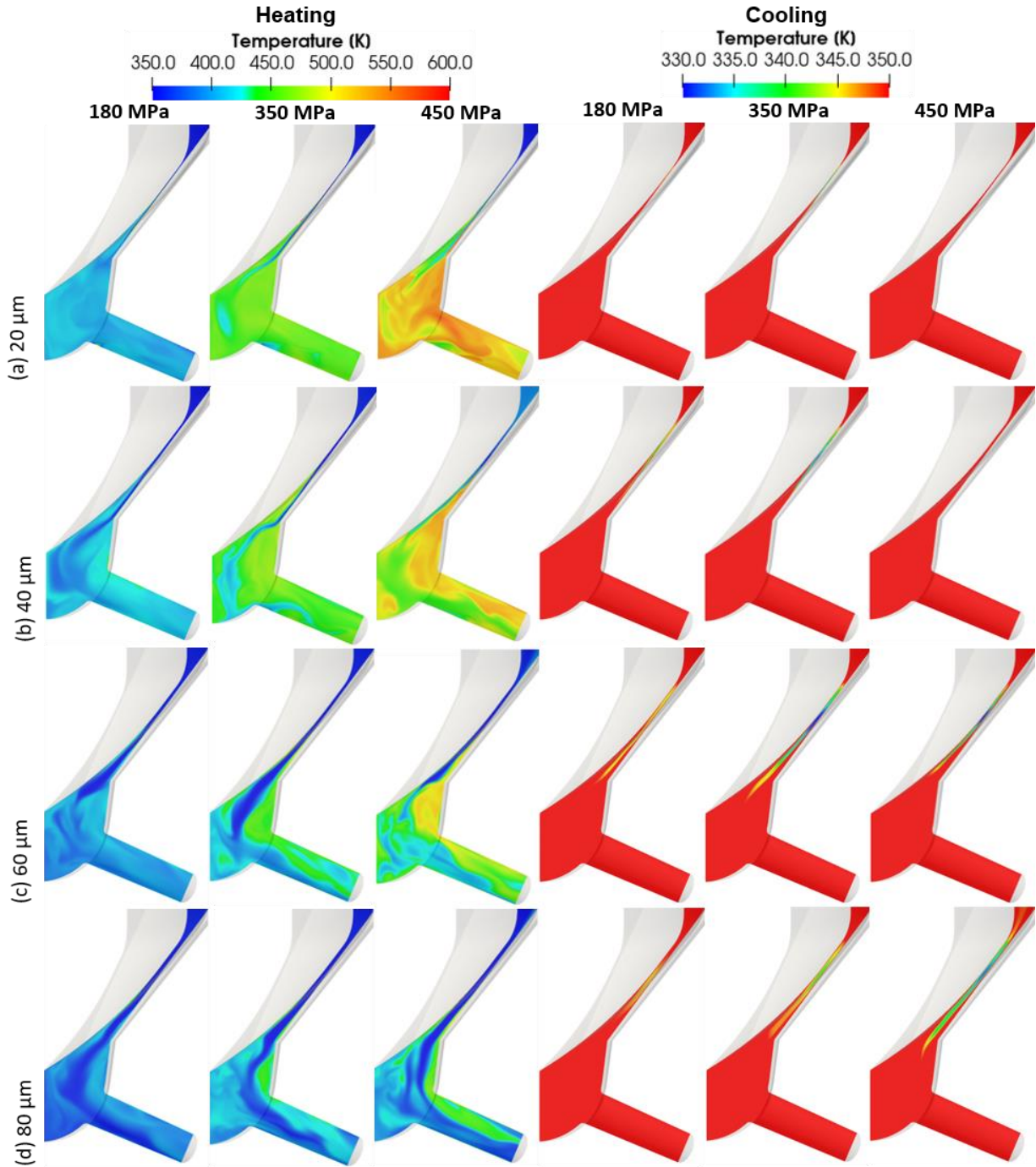
Figure 4. 9. Snapshots of instantaneous temperature field on the mid-plane of the injector. The time instants correspond to needle lifts of: (a) 20 \mu\text{m} , (b) 40 \mu\text{m} , (c) 60 \mu\text{m} and (d) 80 \mu\text{m} .
