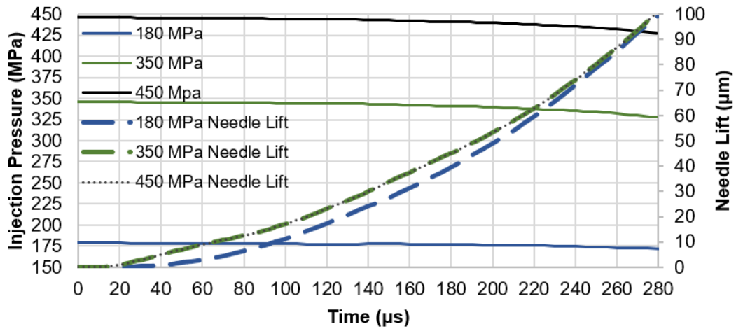
Figure 4. 2. Injection pressure and needle lift profile utilised as boundary conditions until 100 \mu m needle lift.
