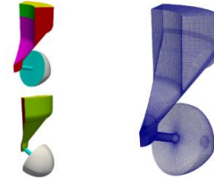
Figure 6. 4. Computational Volume of the 1/5th of injector.
