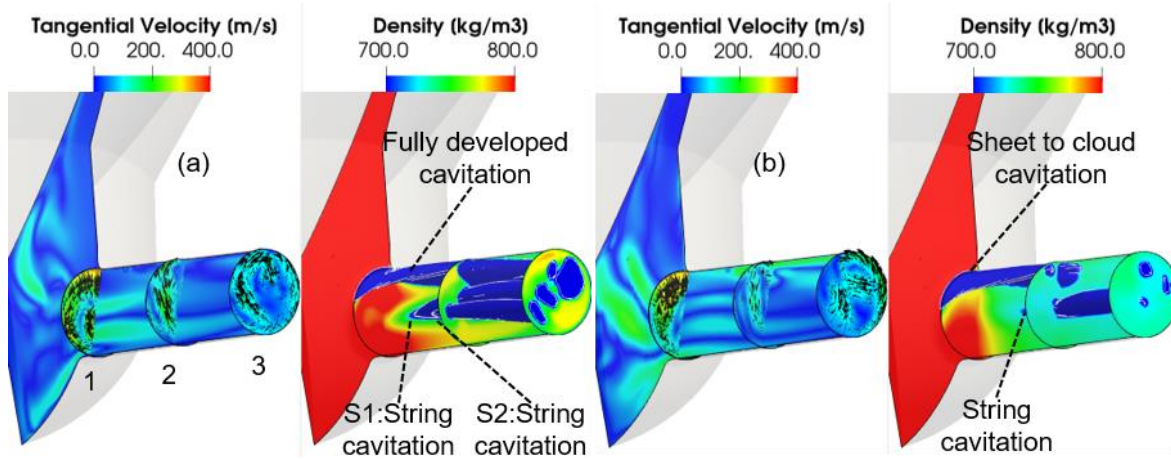
Figure 3. 11. Instantaneous tangential velocity and density distribution on slices normal to the orifice and at the midplane of the injector, at time instant 248 \mu s (132 \mu m needle lift) using (a) full thermodynamic model and (b) barotropic model.
