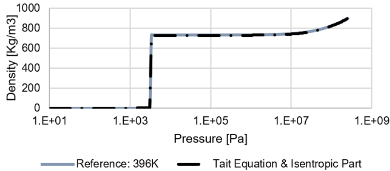
Figure 3. 4. Utilised density variation with pressure, as predicted by the relevant barotropic fluid EoS.
