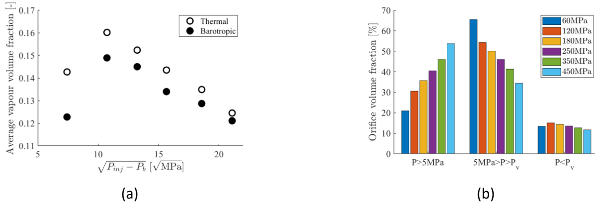
Figure 5. 12. (a) Time-averaged vapor volume fraction inside the injector orifice versus the square root of the pressure drop estimated utilising both the barotropic and thermal models. (b) Orifice volume fraction histogram for different pressure ranges inside the orifice volume when thermal effects are considered.
