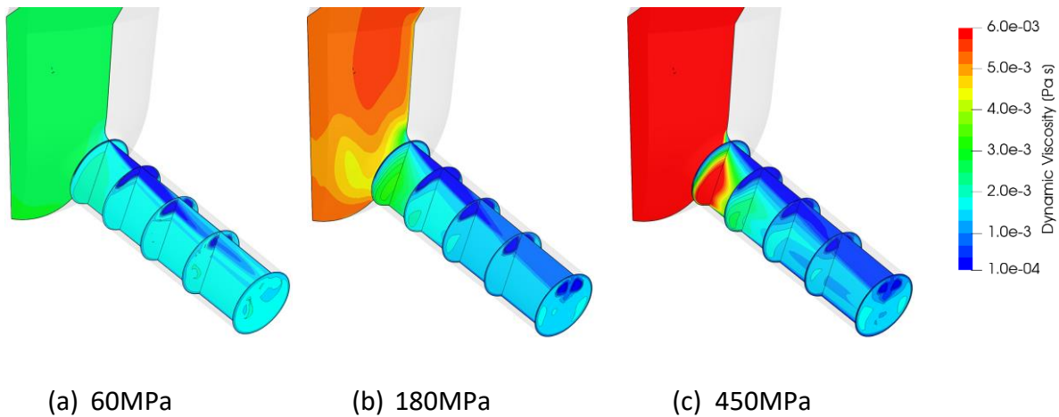
Figure 5. 5. Predicted time-averaged dynamic viscosity on different slices at the sac volume and orifice for three injection pressures. Thermal effects are considered.
