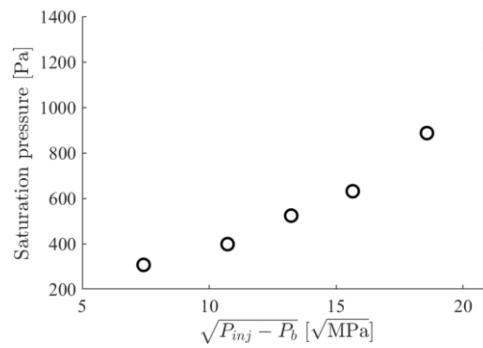
Figure 5. 10. Predicted saturation pressure versus the square root of the pressure difference when thermal effects are considered.
