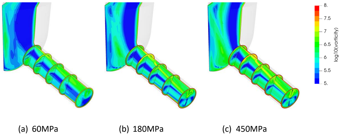
Figure 5. 3. Predicted time-averaged vorticity, in logarithmic scale, on different slices at the sac volume and orifice for three injection pressures. Thermal effects are considered.
