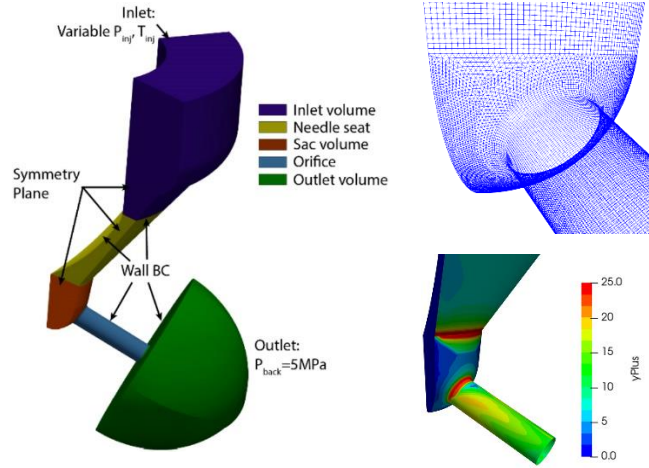
Figure 5. 1 Simulated geometry (one fifth of the complete injector nozzle). Characteristic volumes are colourised and the boundary conditions are indicated. The transition between the two distinct topologies at the orifice and the contour plot at P_{inj}=450\text{MPa} for the estimated y^+ values are also added.
