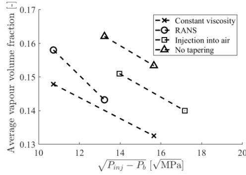
Figure 5. 13. Effect of boundary conditions and simulation parameters on calculated vapor volume fraction as function of pressure drop.
