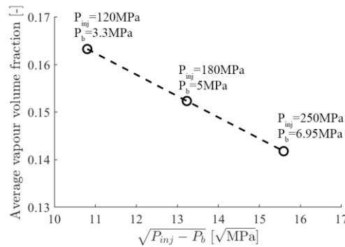
Figure 5. 16. Time-averaged vapor volume fraction inside the injector orifice versus the square root of the pressure drop, considering thermal effects. All cases have the same cavitation number, CN=35 .
