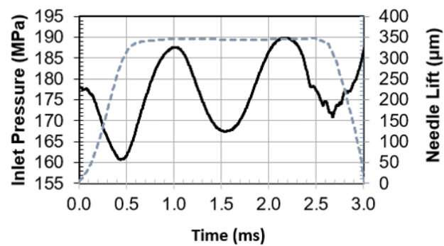
Figure 3. 6. Injection pressure and needle lift utilised as boundary conditions.
