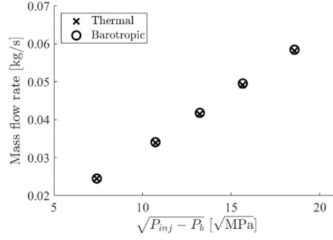
Figure 5. 6. Mass flow rate at the orifice exit for both the barotropic and thermal cases.
