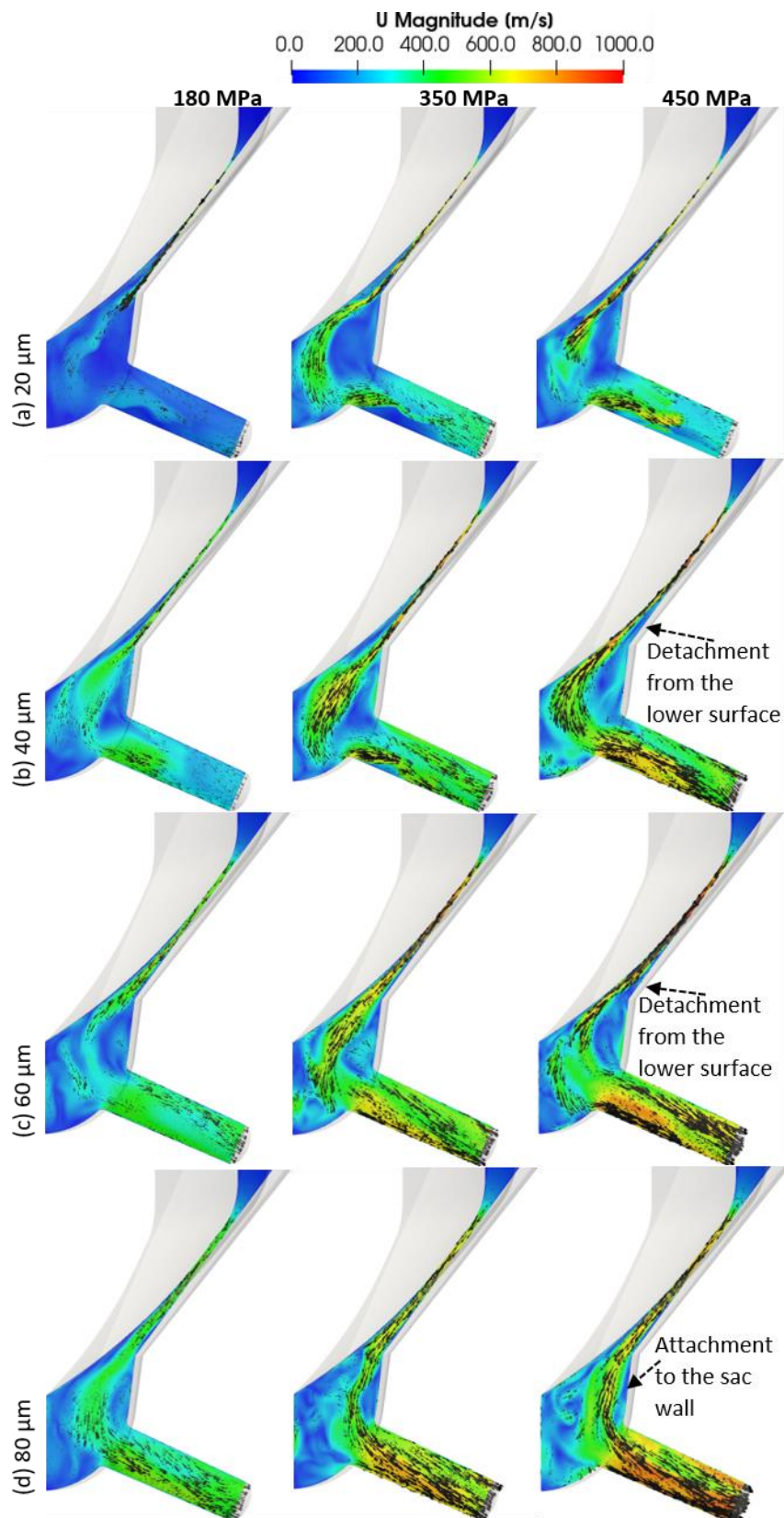
Figure 4. 10. Snapshots of instantaneous velocity magnitude and flow field vectors plotted at time instances corresponding to (a) 20 \mu\text{m} , (b) 40 \mu\text{m} , (c) 60 \mu\text{m} and (d) 80 \mu\text{m} .
