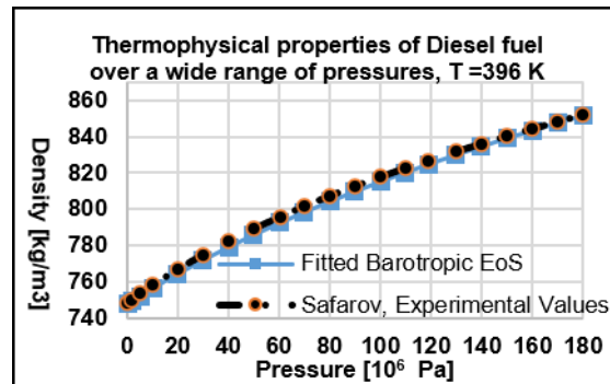
Figure 6. 1. EoS with reference data of Safarov et al. [278]
