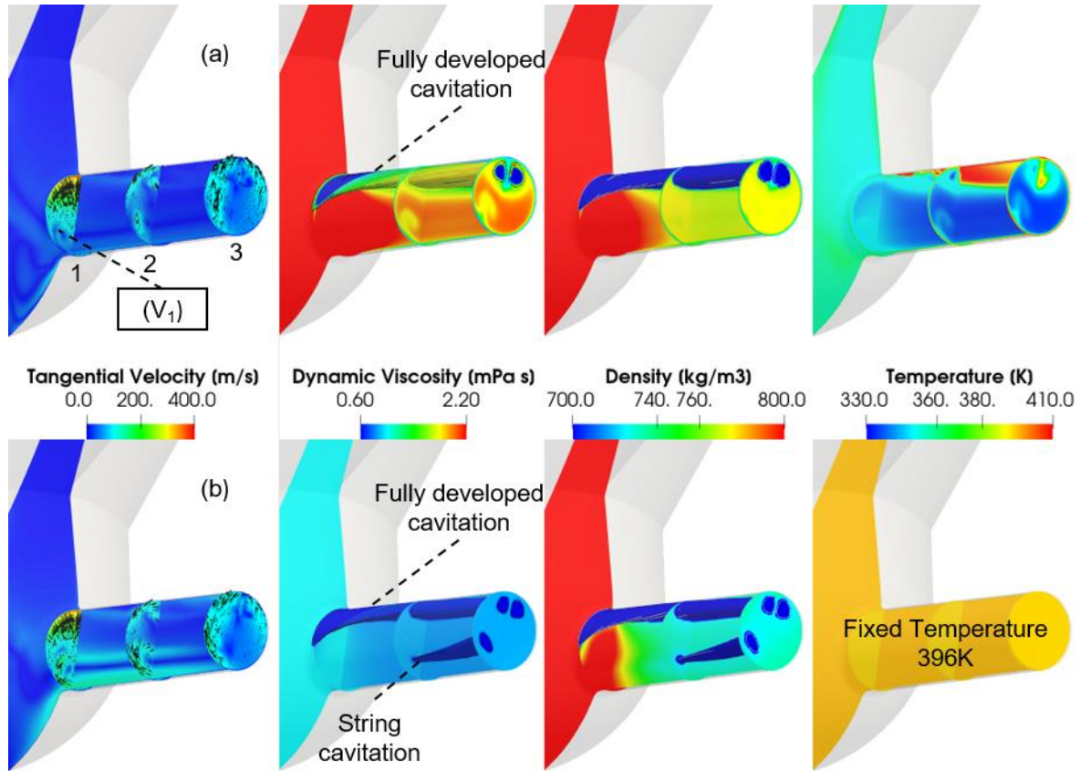
Figure 3. 21. Instantaneous tangential velocity, dynamic viscosity, density and temperature distribution on slices normal to the orifice and at the midplane of the injector, at 989 \mu s (350 \mu m needle lift) after start of injection, (SOI) using (a) full thermodynamic model and (b) barotropic model. The vapor volume fraction \alpha = 0.01-1.0 is coloured by the dynamic viscosity and density.
