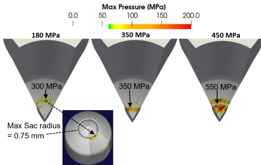
Figure 4. 12. Spatial distribution of accumulated pressure peaks on the surfaces of the needle valve. Strongest collapse events are located on the needle surface, reaching up to 550MPa for the 450MPa case.
