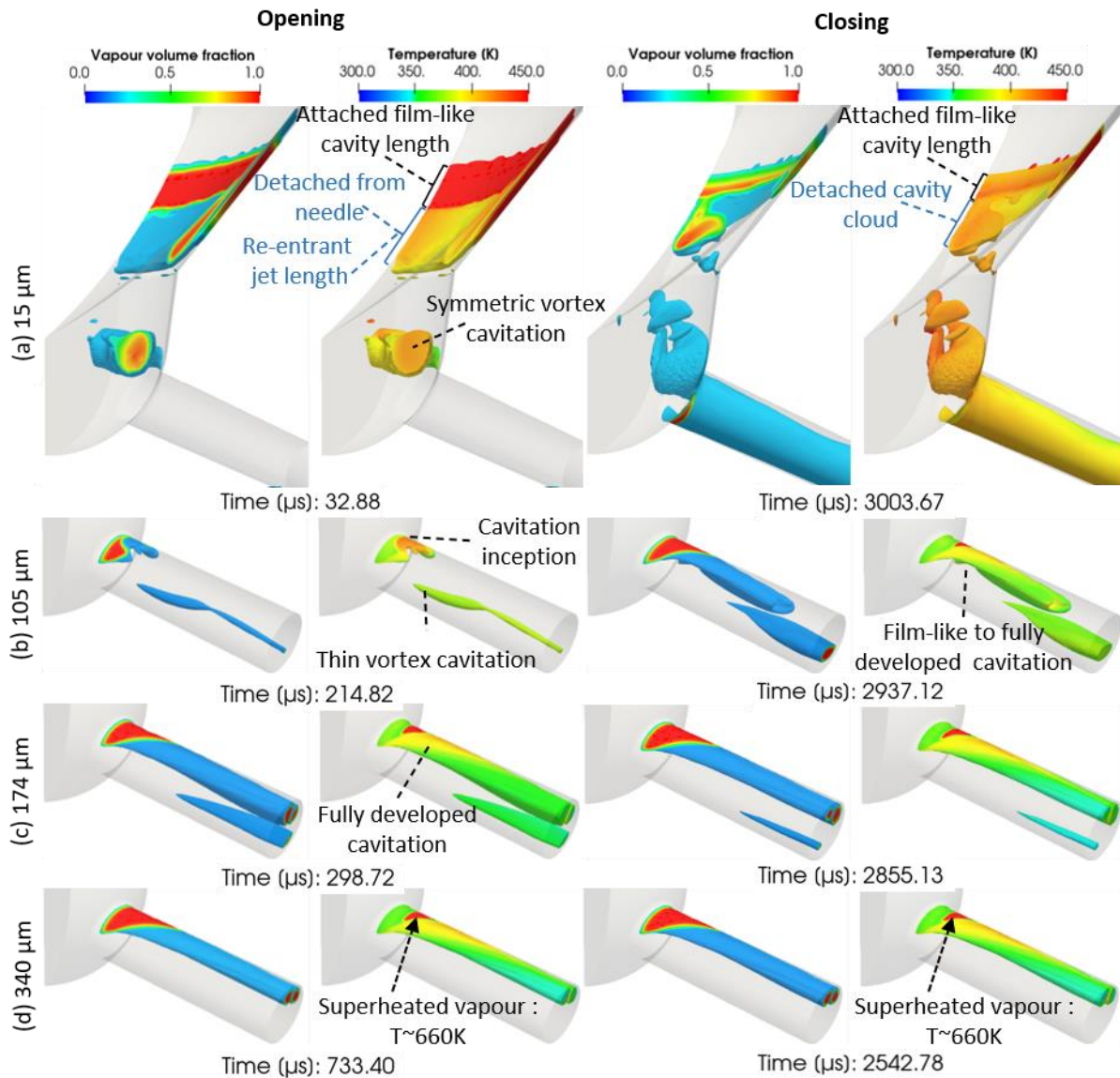
Figure 3. 16. Snapshots of cavitation formation coloured by the temperature and vapor volume fraction during the opening and closing of the needle valve. The time instants correspond to needle lifts (a) 15 \mu\text{m} , (b)105 \mu\text{m} , (c)174 \mu\text{m} and (d)340 \mu\text{m} .
