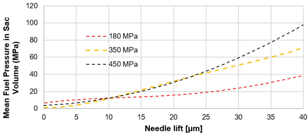
Figure 4. 7. Temporal evolution of fuel pressure in the injector's sac volume; lift increase from 0 \mu\text{m} to 40 \mu\text{m} during the plotted time.
