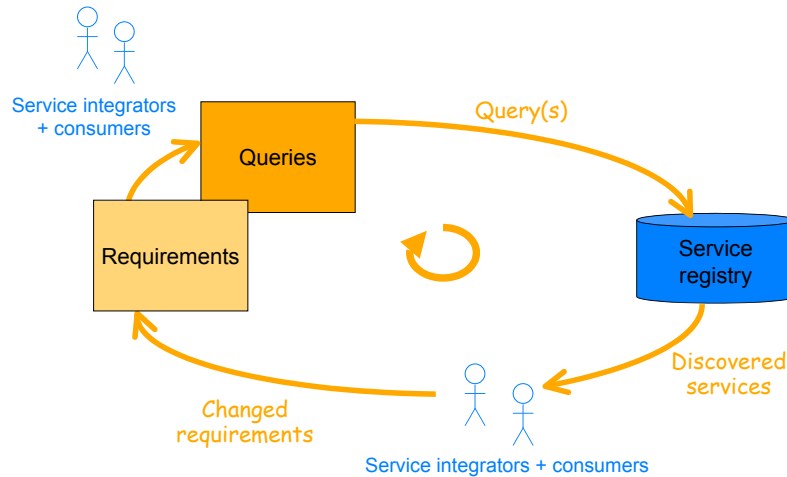
Figure 1. SeCSE's iterative and incremental requirements process.
