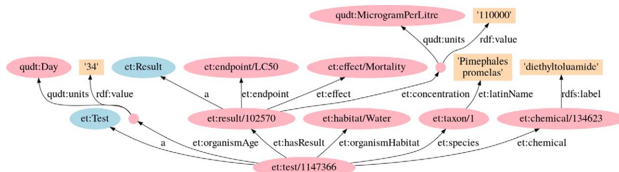
Fig. 3. Example of an ECOTOX test and related triples.
