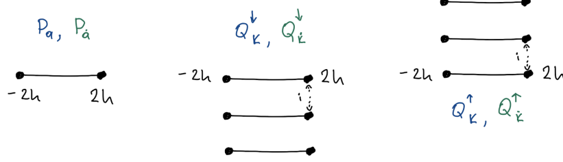
Figure 2. Standard analytic structure of \mathbf{P} 's with one branch cut. As a consequence of this, \mathbf{Q} functions will have an infinite ladder of cuts separated by i in the lower or upper half of the analytic plane.
