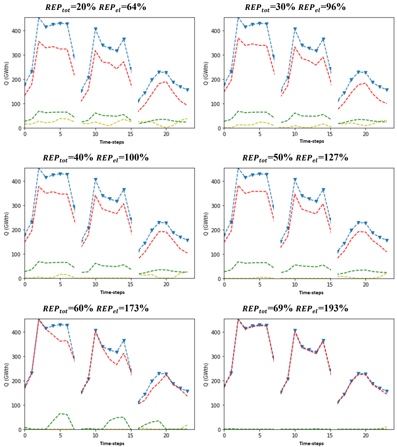
Fig. 8 – Thermal energy consumptions and mix of power systems that satisfy the demand for increasing shares of RESs resulting from the optimizations.
