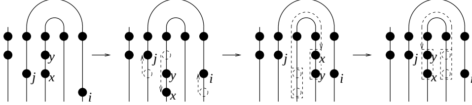
Figure 12: An example of move (M3)
