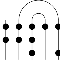
Figure 7: The partition (5, 4) on the new abacus
