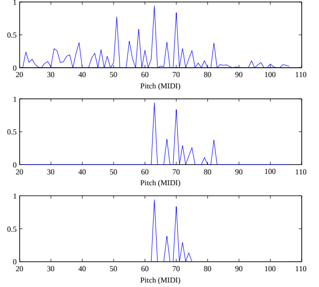
Figure 2: Saliency function stages for an Eb4-G4-Bb4-C5-D5 piano chord. From top to bottom, the figures represent (i) The raw saliency function (ii) The saliency function after the spectral structure rules have been applied (iii) The saliency function after the temporal evolution tests have been applied.
