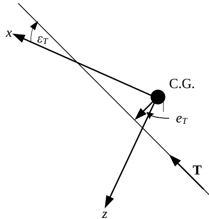
Figure 3-9 Thrust Configuration
