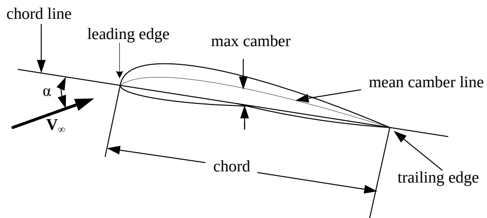
Figure 3-3 Airfoil Cross-Section
