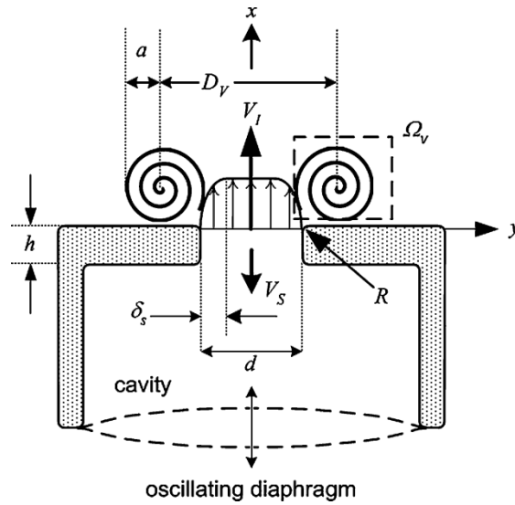
Figure 2-11 synthetic jet actuator (Holman et al., 2005)
