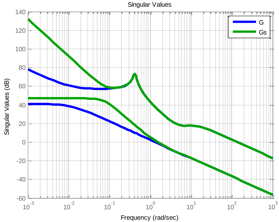
Figure 5-6 Controller effect on the open loop system G
