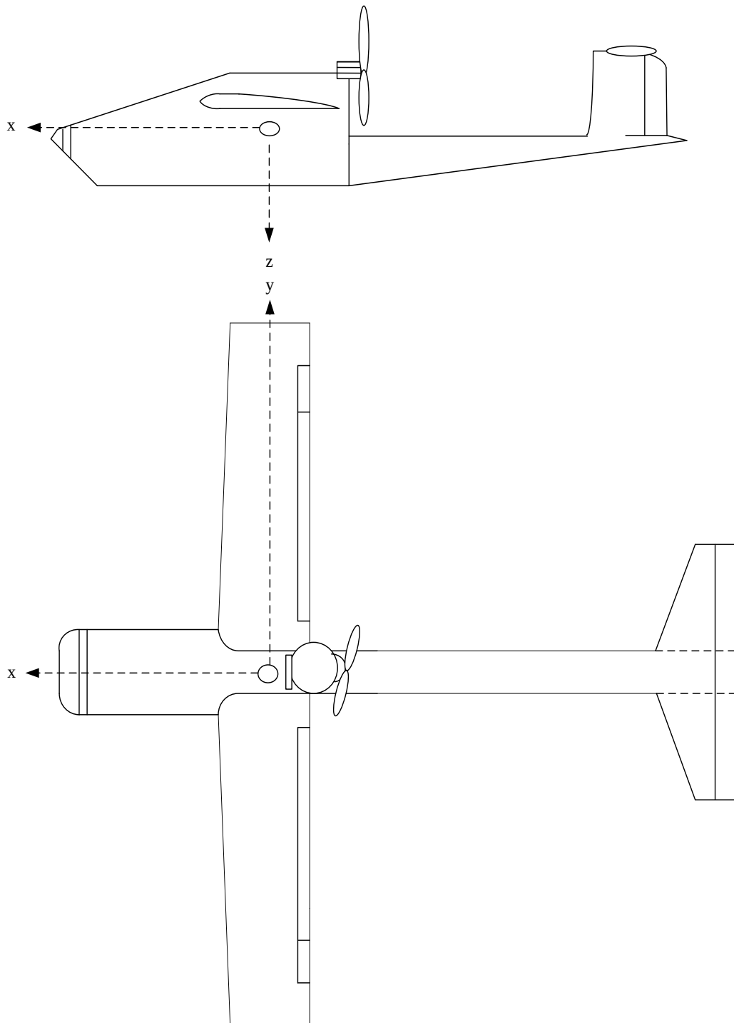
Figure 4-1 X-RAE1 Layout
