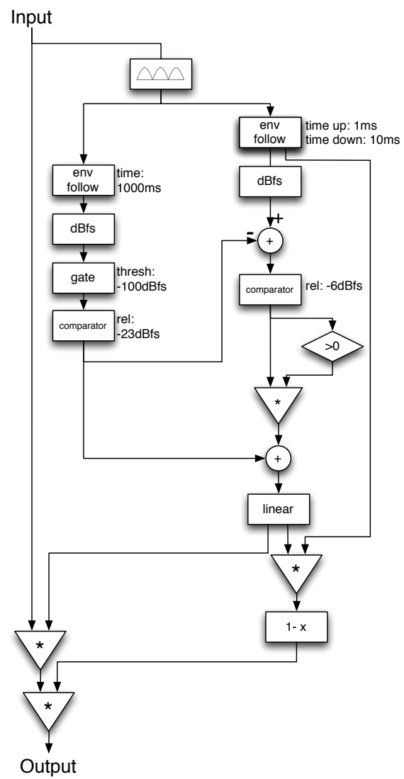
Figure A.4: Dynamic Range Squasher
