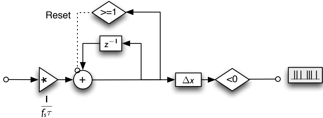
Figure 8.2: Accumulator design
