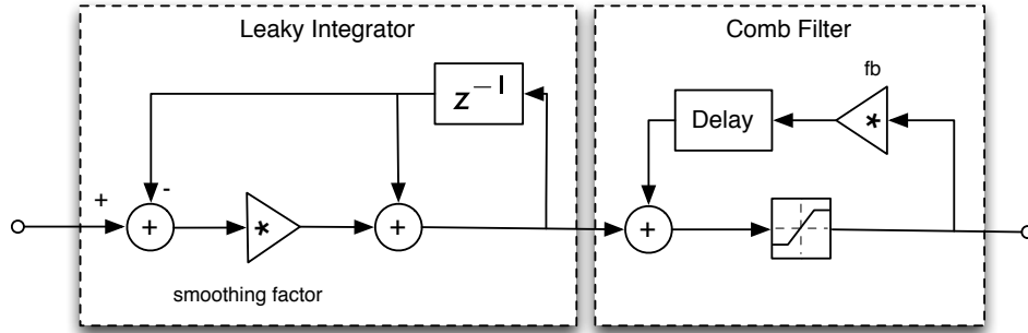
Figure A.1: Envelope follower with integrator and comb filter
