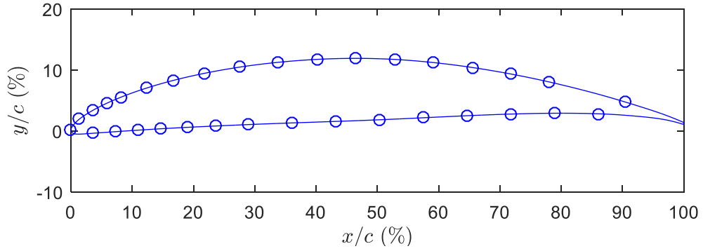
Fig. 2 Positions of the pressure taps on the aerofoil model.
