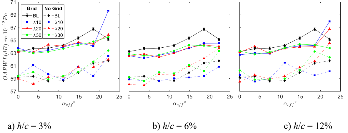
Fig. 14 Variations of overall sound power level with an angle of attack: (a) h/c = 3\% ; (b) h/c = 6\% ; (c) h/c = 12\% .
