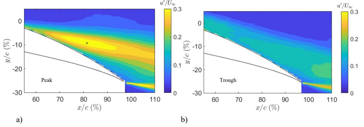
Fig. 17 Colour contours of the turbulence intensity u'/U_\infty downstream of the LEU peak (a) and the trough (b) of an optimized LEU profile (230h6) at \alpha = 15.3^\circ with grid.
