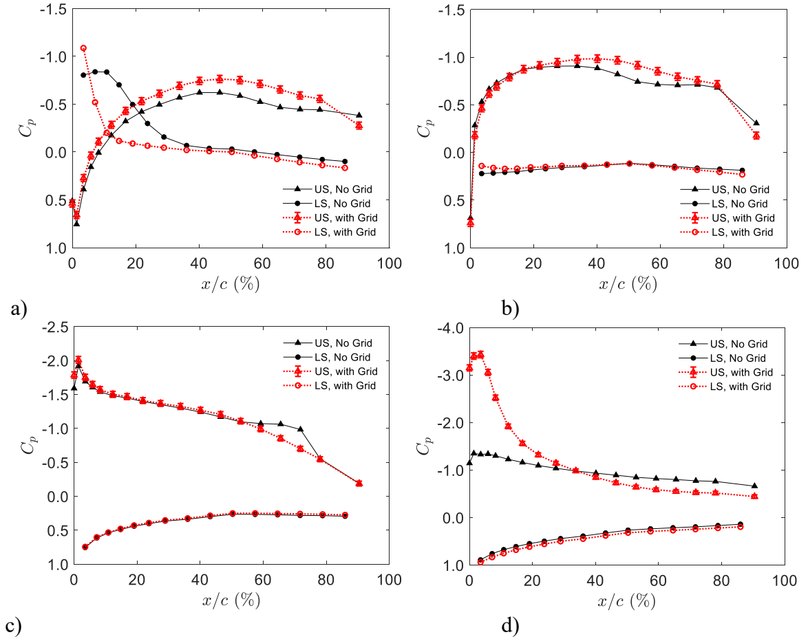
Fig. 5 C_p distributions on the upper surface (US) and the lower surface (LS) at \alpha equal to (a) -1.8^\circ , (b) 5.4^\circ , (c) 9.9^\circ and (d) 19.8^\circ . Error bars to indicate experimental uncertainties are shown in (a).
