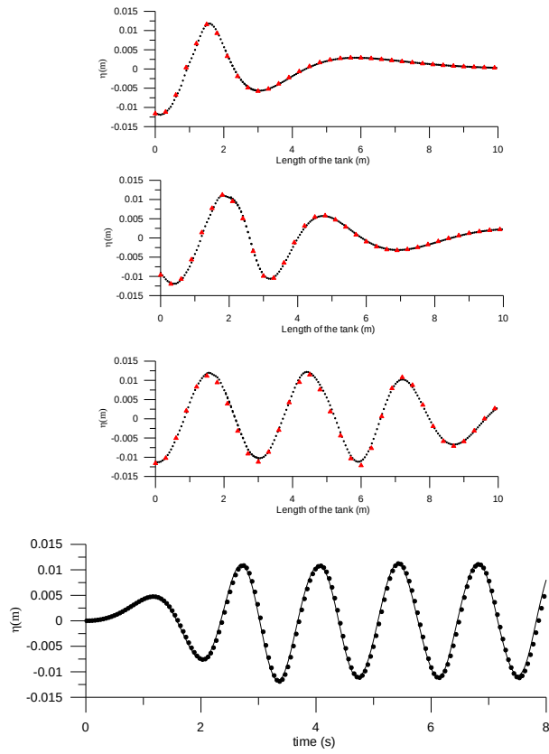
Fig. 12. Comparison between analytical (dot/triangle) and numerical (lines) spatial wave profiles (obtained by using MLPG_R method) at different time instants a) t = 2\text{ s} b) t = 4\text{ s} and c) t = 8\text{ s} (d) time history at x = 4\text{ m} .
