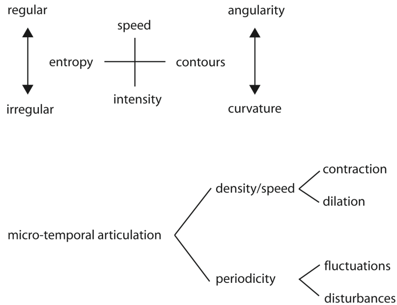
Figure 13: Perturbation.
