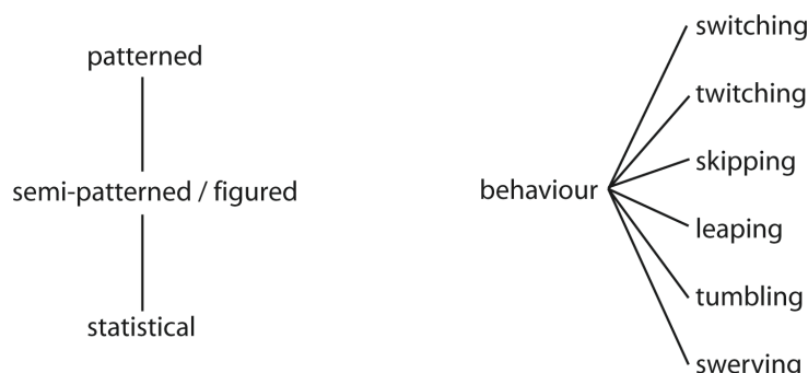
Figure 14: Fractional motion.
