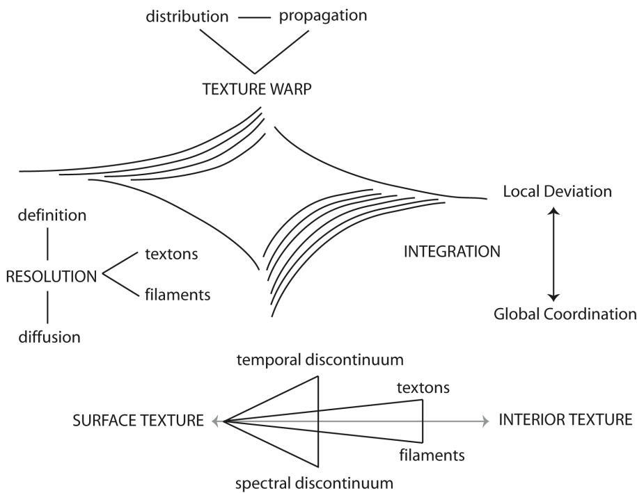
Figure 7: Low-level topology.
