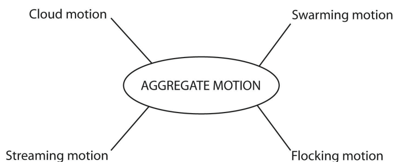
Figure 15: Aggregate motion.
