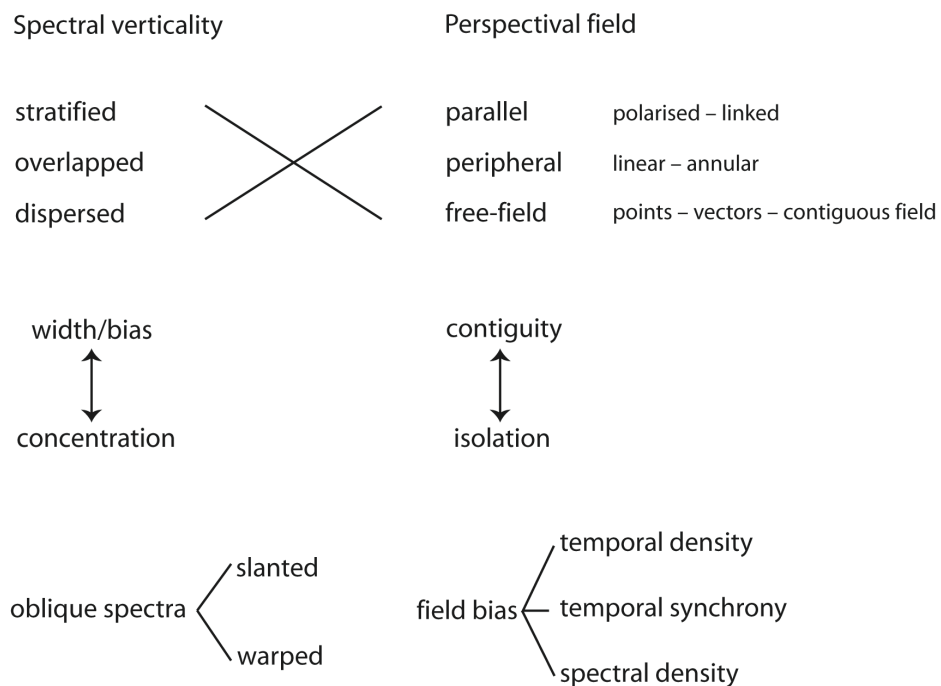
Figure 6: Distributions.
