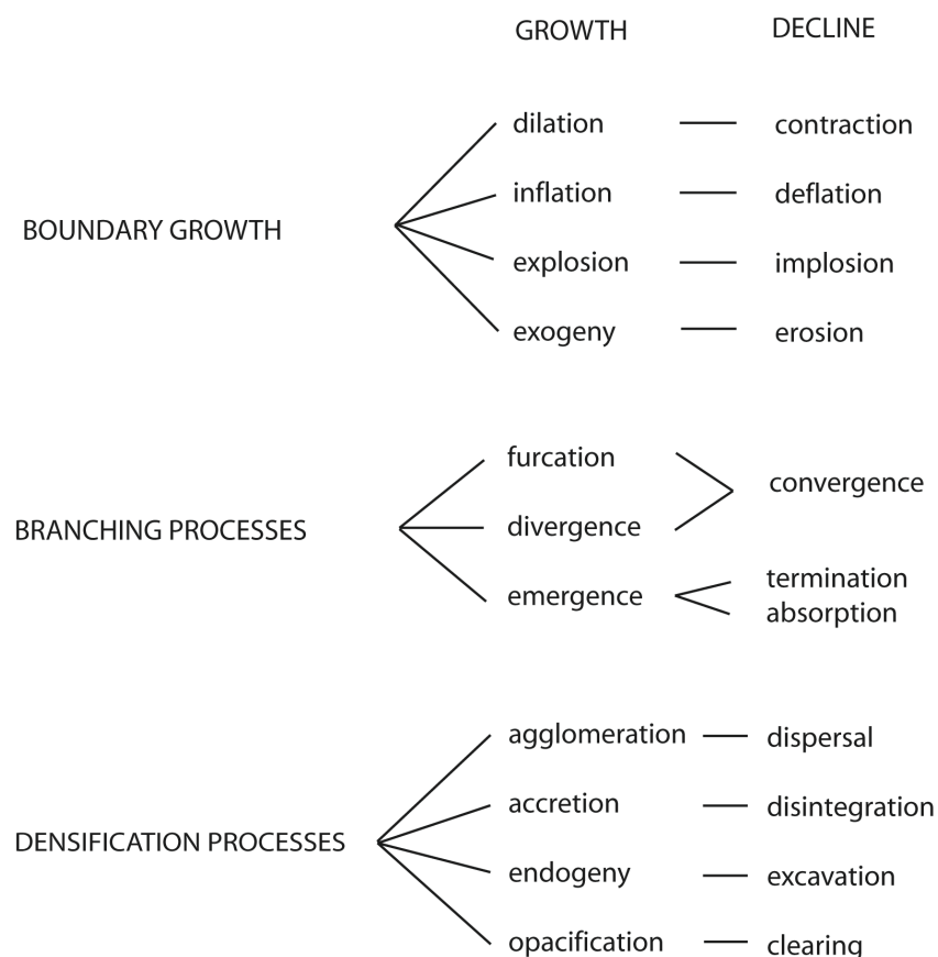
Figure 12: Growth processes.
