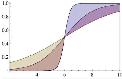
Fig. 5: Sigmoid-function \sigma(\frac{x-a}{\tau}) for a=6 and \tau = 0.2, 1.0 , and 2.0
