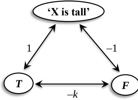
Fig. 4: Simple neural network with one input node (representing ‘X is tall’) and two output nodes ( T and F ).
