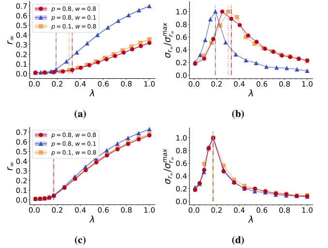
FIG. 2: In panel a) we display the final epidemic size ( r_\infty = R_\infty / N ) with 95% confidence intervals and in panel b) the normalized relative variance \sigma_{r_\infty} / \sigma_{r_\infty}^{\max} for different values of \lambda in the case of non-perfect random adoption. Vertical dashed lines indicate the analytical threshold derived from Eq. 6 for the different values of p and w considered. In panel c) and d) we repeat the analysis in the case of non-perfect adoption dependent from nodes' activity for different values of p and w . In all figures, we represent median and 95% confidence intervals obtained from 10^2 stochastic simulations for each point with the following parameters \mu = 10^{-2} , N = 10^6 , m = 2 , \epsilon = 10^{-3} , \alpha = 2.1 , i_0 = I_0 / N = 0.01 (initial fraction of infected seeds), \gamma = 0.8 , \psi = 0.1 .
