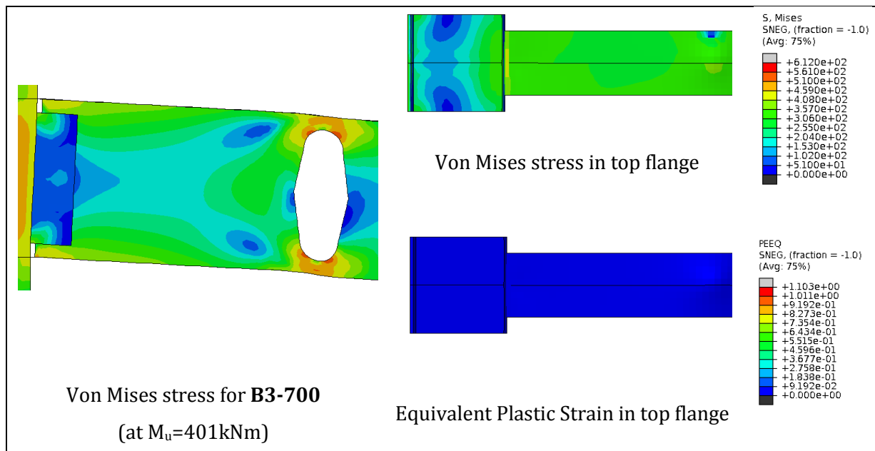
Figure 13: Stress and strain distribution for opening B3-700
