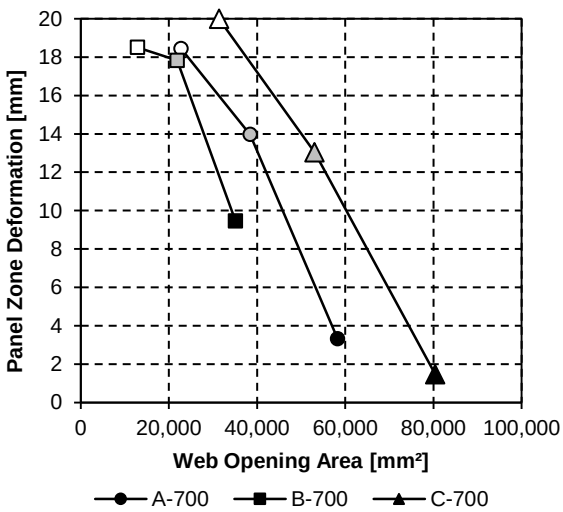
Figure 20c: Panel-zone shear deformation when S=700\text{mm}
