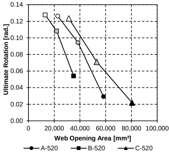
Figure 17b: Ultimate rotation of openings for S=520mm
