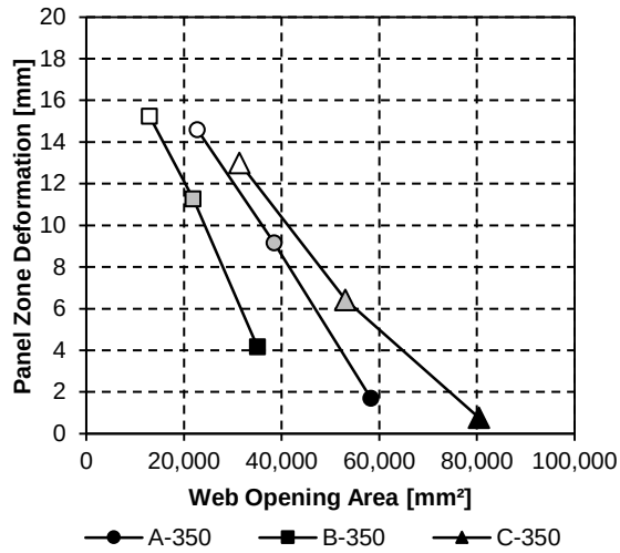
Figure 20a: Panel-zone shear deformation when S=350\text{mm}
