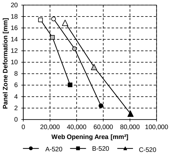
Figure 20b: Panel-zone shear deformation when S=520\text{mm}
