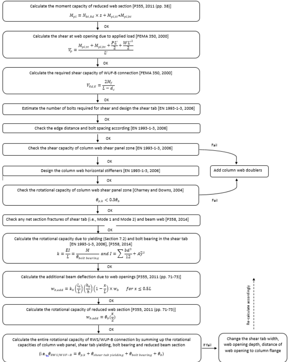
Figure 21: Design process of RWS/WUF-B connections
