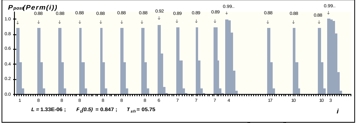
Figure 6. P_{post}(Perm) for Example 2 ( \theta t = 2 \cdot 10^{-6} , \beta 1 = 10^{-6} )
