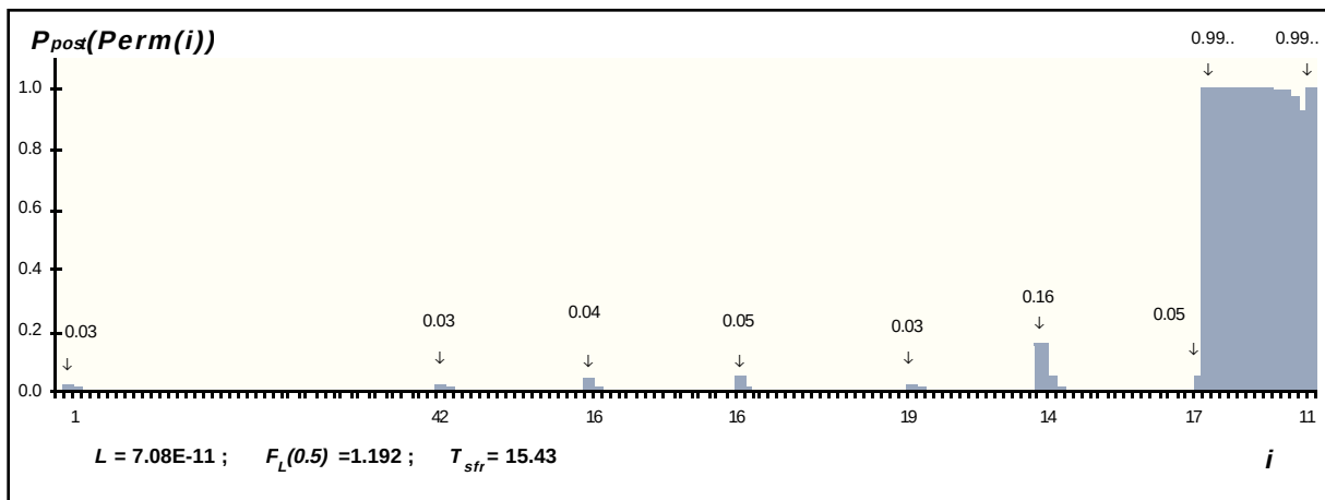
Figure 4. P_{post}(Perm) for Scenario C (as in Figure 3, but with \theta t = 100 \cdot \theta p )
