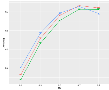
(c) n = 200
