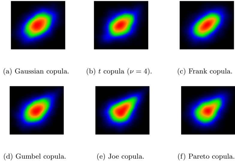
Figure 1: Examples of heatmap images of smoothed bivariate densities for different copula models ( n = 2000, \tau = 0.3 ).
