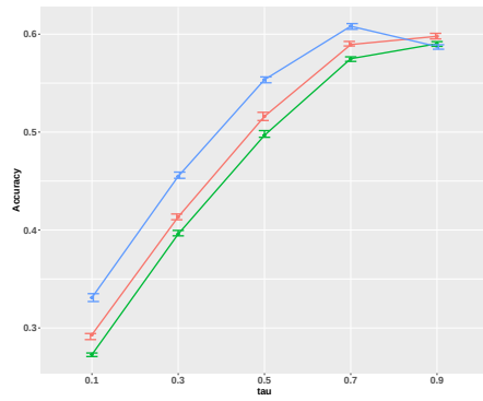
(a) n = 100
