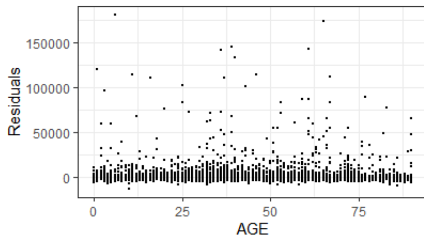
Figure 3.11: Scatter plot of residuals vs. AGE of the two-part model.
