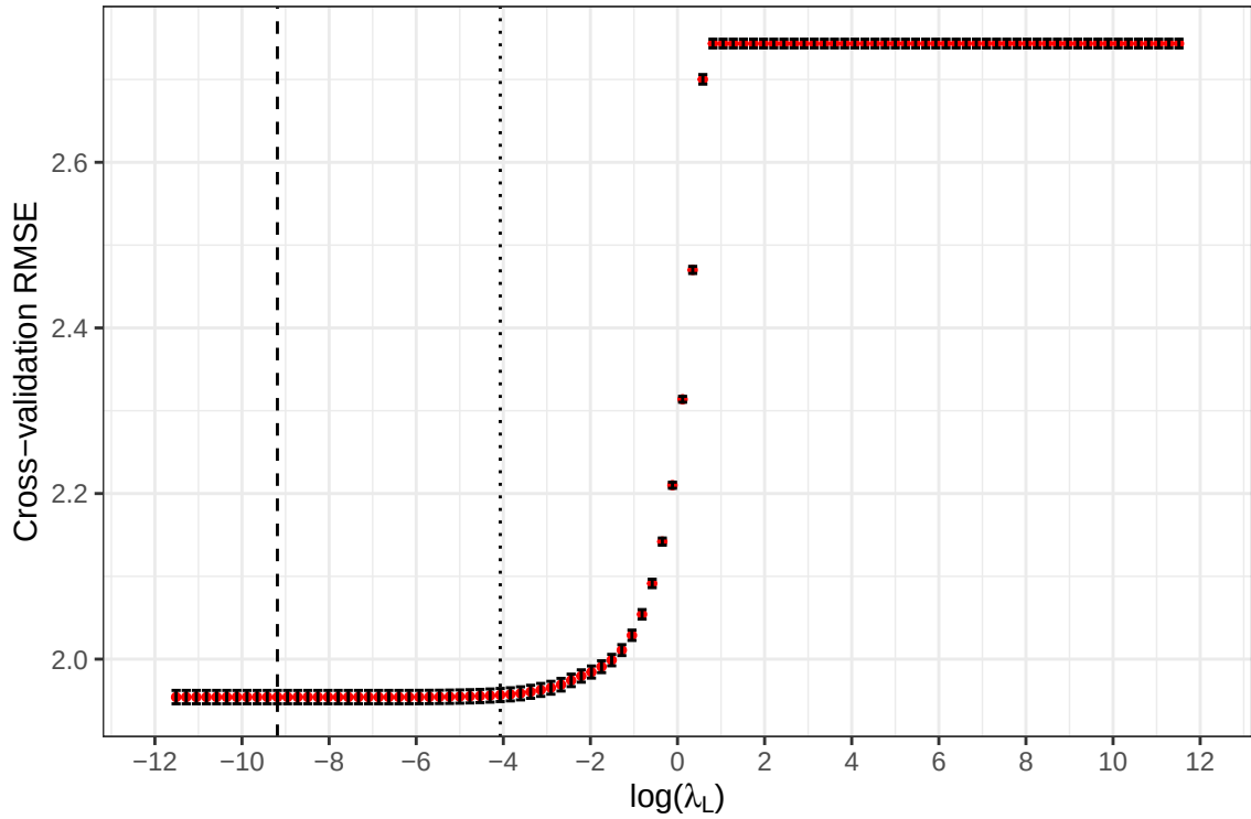
Figure 5.7: Change in the cross-validated RMSE with the increase of shrinkage factor - GBD.
