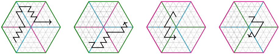
Fig. 17 We let h = 3 , \ell = 1 , e = 5 and \alpha = \varepsilon_3 - \varepsilon_1 and \beta = \varepsilon_1 - \varepsilon_2 and \gamma = \varepsilon_2 - \varepsilon_3 . The paths P_{\alpha\beta\alpha} , P_{\beta\alpha\beta} , P_{\gamma\beta\gamma} and P_{\beta\gamma\beta} are pictured
