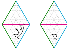
Fig. 21 We let h = 3 , \ell = 1 , e = 5 and \alpha = \varepsilon_3 - \varepsilon_1 and we depict the paths P_\alpha^b and P_\emptyset (we actually only depict P_\emptyset which is a third of the path P_\alpha ). We have already constructed the corresponding element \text{spot}_\alpha^\emptyset in great detail over the course of Examples 3.6, 3.8 and 3.10 and Fig. 13
