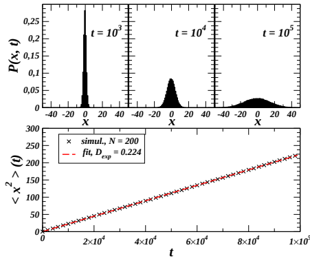
FIG. 5: Evolution of the position of an interface \dots AAABBB \dots . Top: evolution of the distribution \mathcal{P}(x, t) . Bottom: evolution of the mean square displacement, showing a clear diffusive behavior \langle x^2 \rangle = 2D_{exp}t/N with a coefficient D_{exp} \approx 0.224 in agreement with the theoretical prediction.
