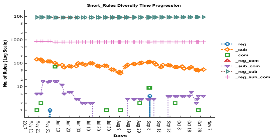
Fig. 8 Time progression of diversity in snort rules
