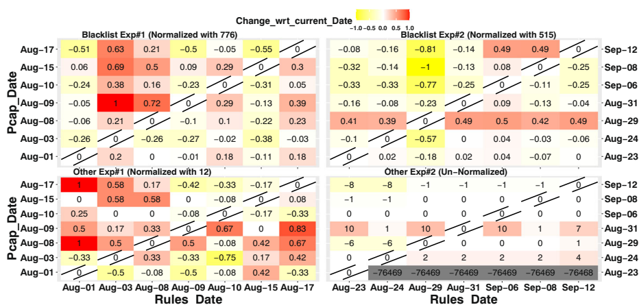
Fig. 13 Evolution of the Suricata alerting behaviour
