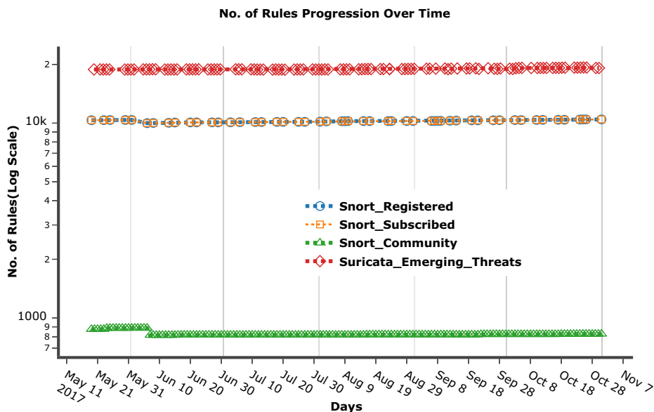
Fig. 7 Snort and Suricata rule counts over the duration of the experiment
