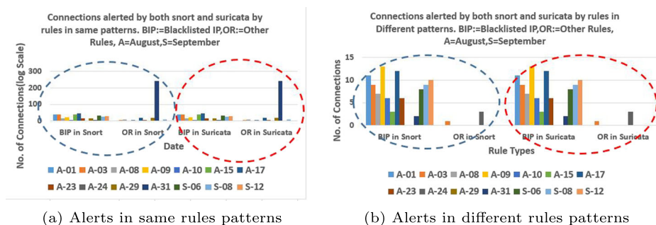
Fig. 16 Analysis of connections alerted by both snort and Suricata
