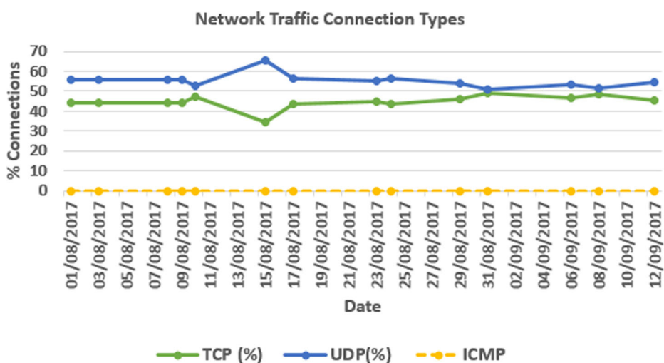
Fig. 11 Pcap Traffic Connections type breakdown
