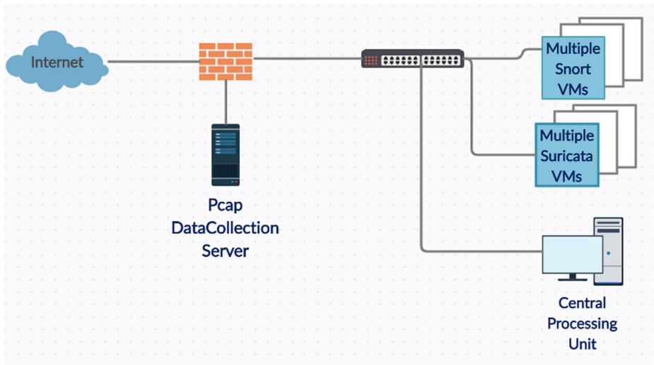
Fig. 2 Data collection infrastructure
