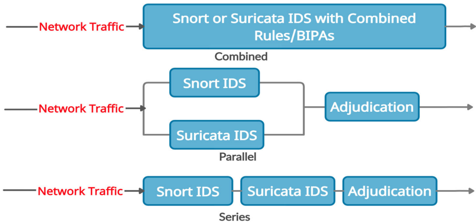
Fig. 17 IDS Deployment strategies
