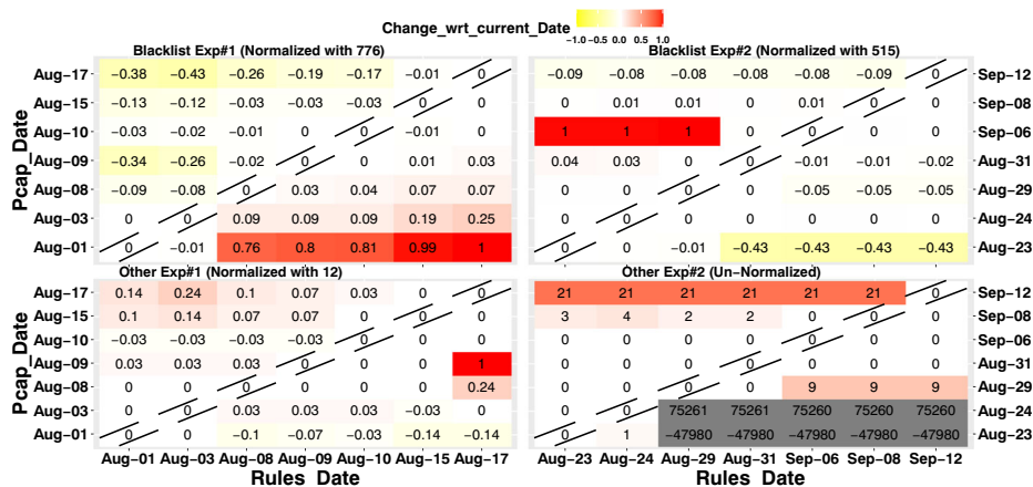
Fig. 12 Evolution of the snort alerting behaviour
