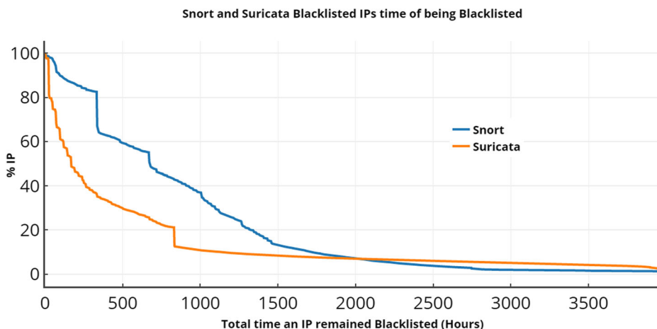
Fig. 4 Total time (Hours) an IP remained blacklisted
