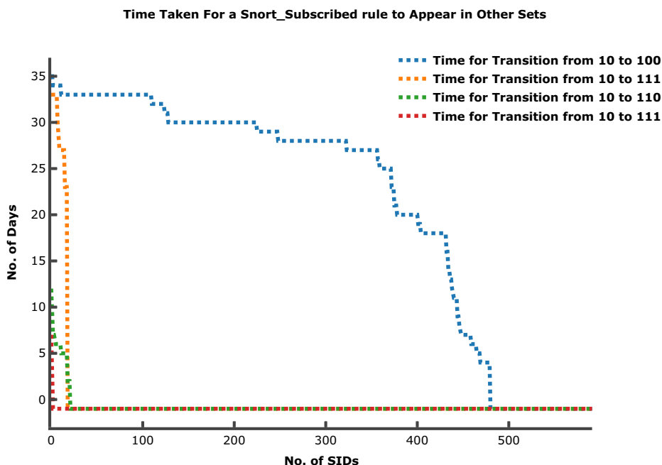
Fig. 9 The time lag for Subscribed rules to appear in the other Snort Rulesets
