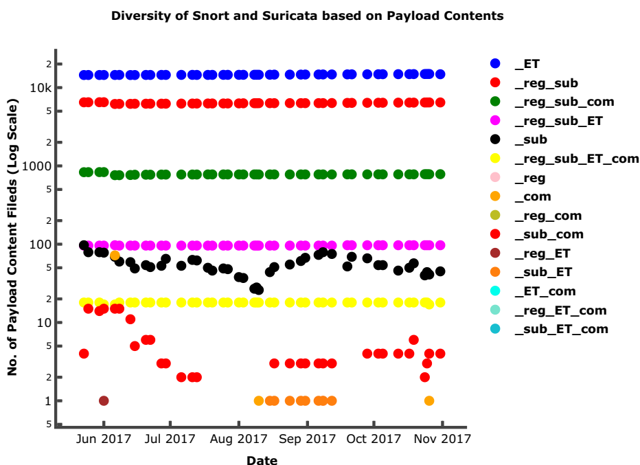
Fig. 10 Evolution of Configurational Diversity of the Snort and Suricata rulesets
