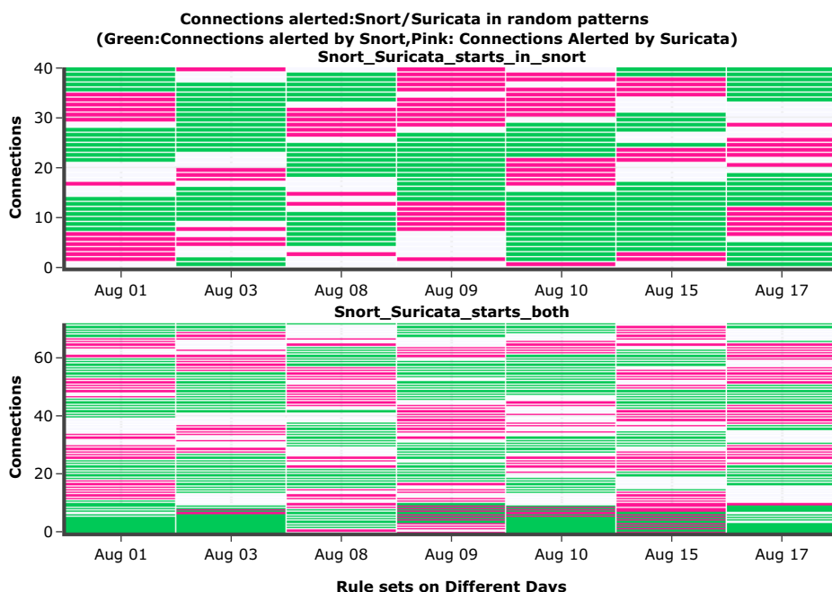
Fig. 15 Distribution of connection alerted by both in different patterns. Green: Snort; Pink: Suricata Patterns, experiment 1
