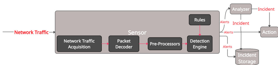
Fig. 1 Snort IDS architecture
