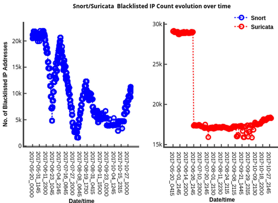
Fig. 3 Count of Blacklisted IPs in Snort and Suricata in our collection period
