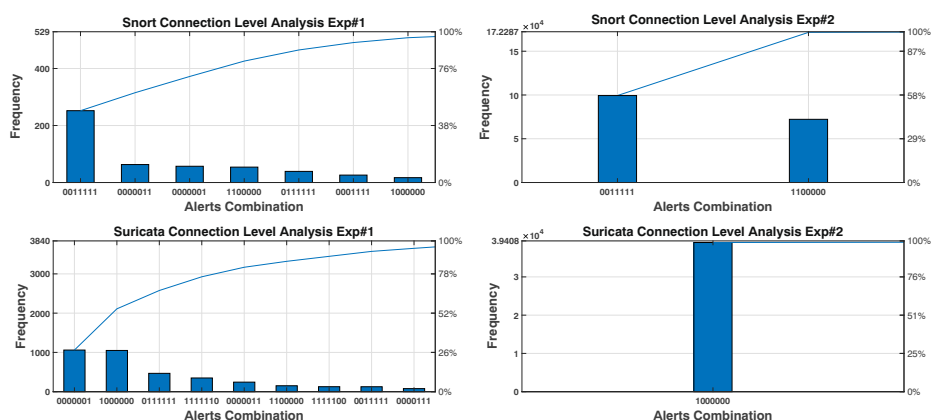
Fig. 14 Diversity in Time, Snort: Top row, Suricata: Lower row
