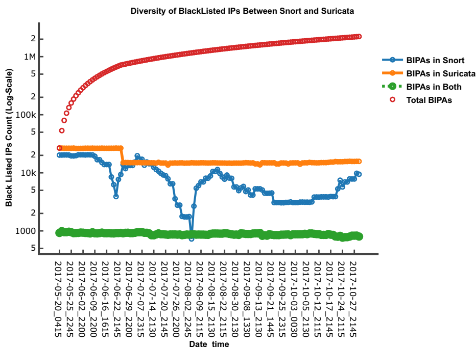
Fig. 5 Diversity in BIPAs as collected from Snort and Suricata sources
