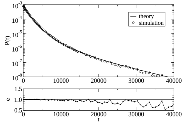
FIG. 5: First passage time distribution - Average on all target nodes s : The distribution of the FPT obtained is shown (ER graph: N = 10^3 , \langle k \rangle = 6 ). At each run both the target node s and the starting node of the random walker are randomly chosen. This means that in this distribution the degree of the target nodes is no more fixed. The non exponential curve is the result of the convolution of several exponential curves obtained for fixed k(s) . The theoretical curve, obtained according to eq.(8), is in excellent agreement with data from simulation performed on a single graph. The fractional error e , defined as the ratio between simulated and calculated data, is also plotted. For large times poor statistics causes bigger fluctuations of e .
