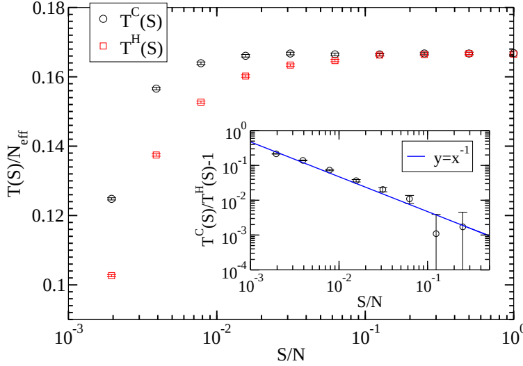
Figure 5. Consensus time T(S)/N_{\text{eff}} as a function of the number of initial states S on a d = 1 lattice with N = 10^3 nodes with a correlated initial configuration made of blocks of voters in the same state, of initial length N/S , T^C(S) , compared with the consensus time obtained with random homogeneous initial conditions T^H(S) . In the inset we show that the quantity T^C(S)/T^H(S) - 1 goes to zero with a power law behavior with exponent -1 . Error bars are obtained as in Figure 3. Each point is averaged over 10^5 runs.
