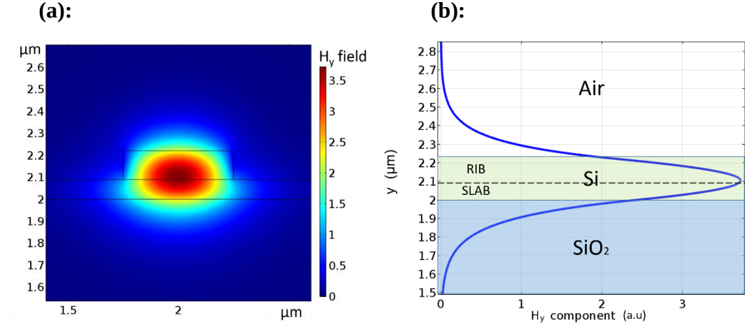
Fig. 4.4 (a) H_y field profile, (b) H_y variation along the vertical direction, for input Si rib waveguide with W = 500 \text{ nm} , H = 220 \text{ nm} , and S = 90 \text{ nm} .
