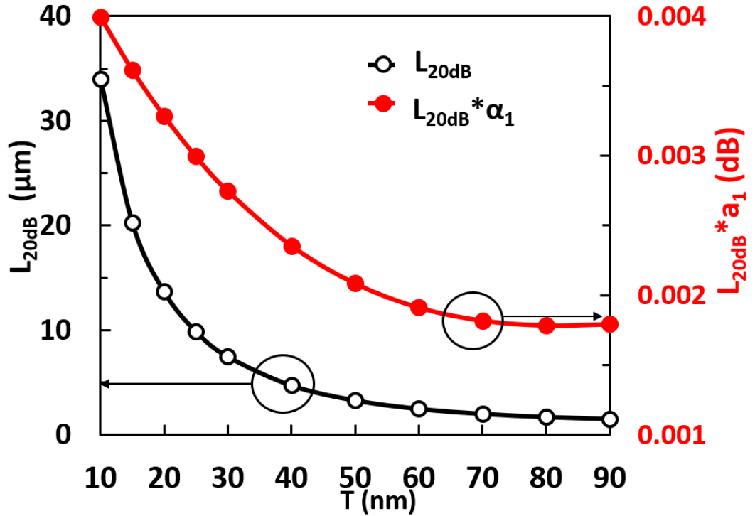
Fig. 6.8. L_{20\text{dB}} and total modal loss of CW in amorphous state with varying GSST thickness, T .
