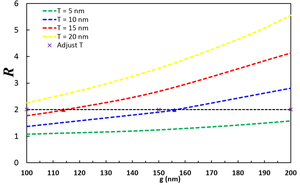
Fig. 7.16. The ratio of the coupling length, R as a function of the waveguide gap, g for GSST layer thickness, T = 5 -20 nm.
