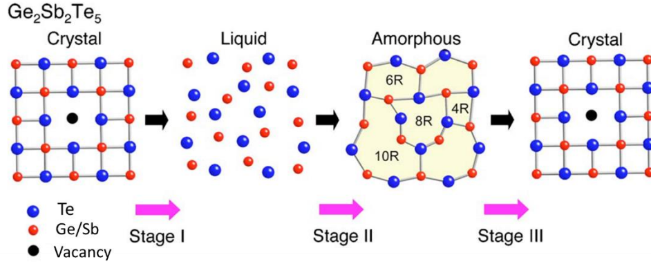
Fig. 2.4. Schematic presentation for the possible ring size transformation in Re-amorphization and crystallization process in \text{Ge}_2\text{Sb}_2\text{Te}_5 . [54]
