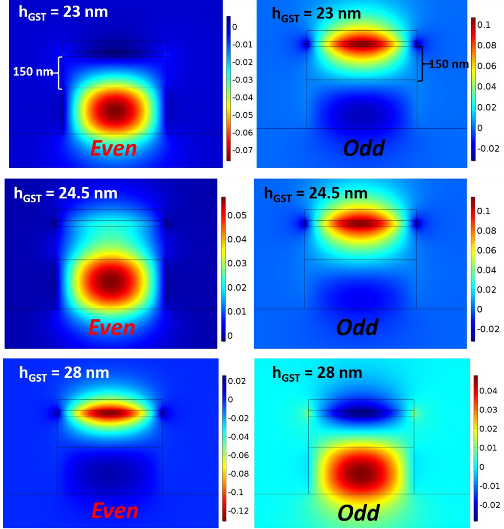
Fig. 5.4. H_y field profiles of the H_y^{11} even and odd supermodes in crystalline state for S_{ITO} = 150 nm and h_{GST} = 23, 24.5 and 28 nm.
