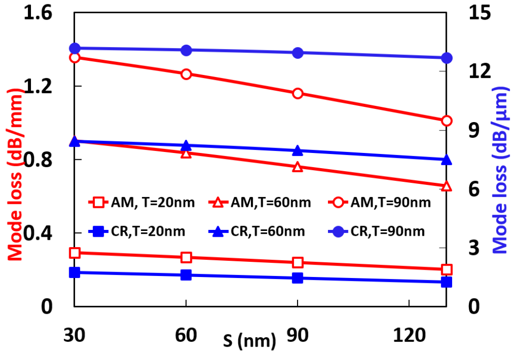
Fig. 6.6. Variations of mode loss of CW in amorphous and crystalline states with Si slab thickness, S of three different values of T ( W = 500 nm, H = 220 nm).
