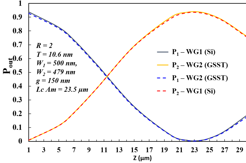
Fig. 7.21. Power transfer, P_{out} with the power launching at I_1 and I_2 for the case R = 2 ( T = 10.6 \text{ nm} , g = 150 \text{ nm} ) along the propagation direction Z .
