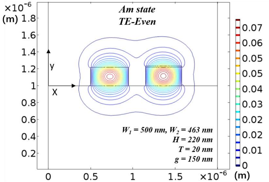
Fig. 7.6. 2D contour plot of the H_y field of the quasi-TE even-like supermode with W_1 = 500 \text{ nm} , W_2 = 463 \text{ nm} , H = 220 \text{ nm} , T = 20 \text{ nm} and g = 150 \text{ nm} (GSST-AM).
