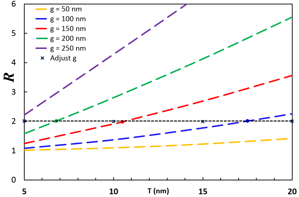
Fig. 7.15. The ratio of the coupling length, R as a function of the GSST thickness, T for waveguide gap, g = 50 - 250 nm.
