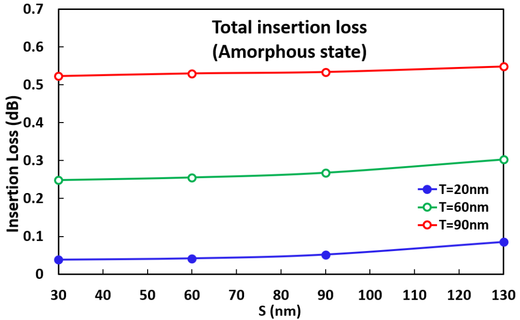
Fig. 6.12. Variations of total insertion loss of CW in amorphous state with Si slab layer S .
