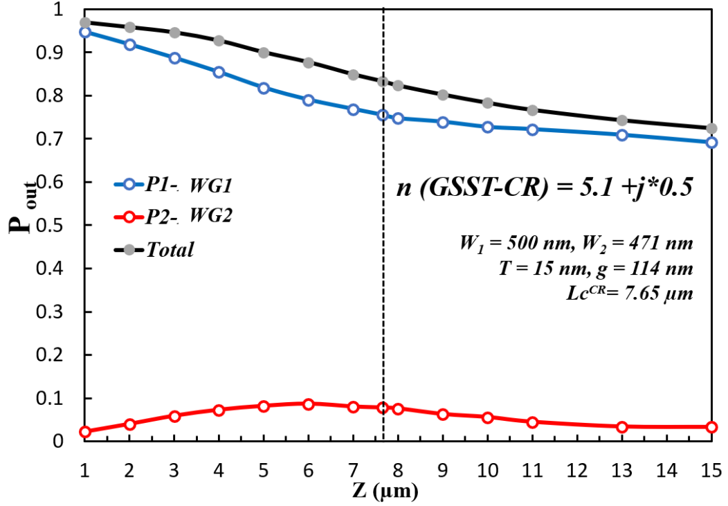
Fig. 7.29. Power transfer, P_{out} at WG1 and WG2 with the desired R = 2 case ( T = 15 nm, g = 114 nm) when GSST in CR state ( n = 5.1 + 0.5*j ) along the propagation direction Z .
