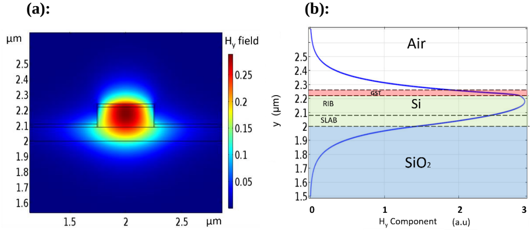
Fig. 4.6.(a) H_y field profiles, (b) H_y variation along the vertical direction, for WG1 in crystalline state with W = 500 \text{ nm} , H = 220 \text{ nm} , S = 90 \text{ nm} , T = 20 \text{ nm} .
