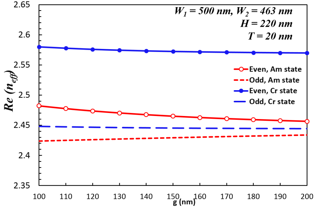
Fig. 7.11. Variations of the real part of the effective index of the even and odd supermodes as a function of the gap, g for phase matched waveguides ( W_1 = 500 nm, W_2 = 463 nm, H = 220 nm and T = 20 nm) at GSST AM and CR state.
