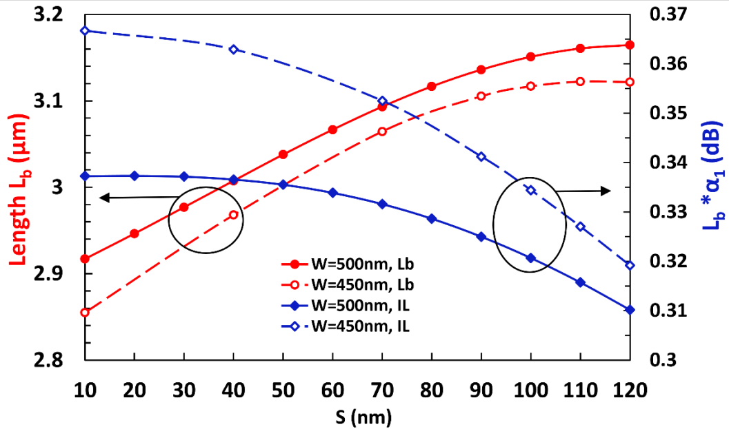
Fig. 4.14. L_b and total modal loss in amorphous state with varying S for two different widths.
