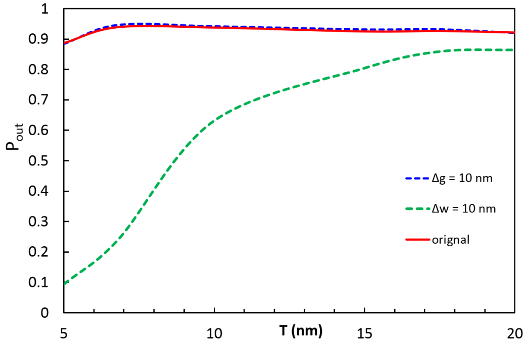
Fig. 7.31. Power transfer, P_{out} of the GSST-loaded Si waveguide at the coupling length position Z = L_c^{AM} with the case: (g + 10 \text{ nm}) , (W_2 + 10 \text{ nm}) and the desire R = 2 as a function of the GSST thickness, T at GSST AM state.
