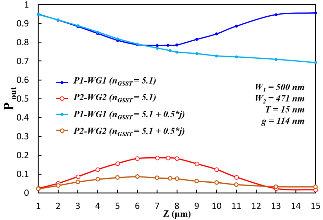
Fig. 7.30. Power transfer, P_{out} at WG1 and WG2 for the desired R = 2 case ( T = 15 \text{ nm} , g = 114 \text{ nm} ) when GSST in CR state with refractive index ( n = 5.1 ) and ( n = 5.1 + 0.5*j ) along the propagation direction Z .
