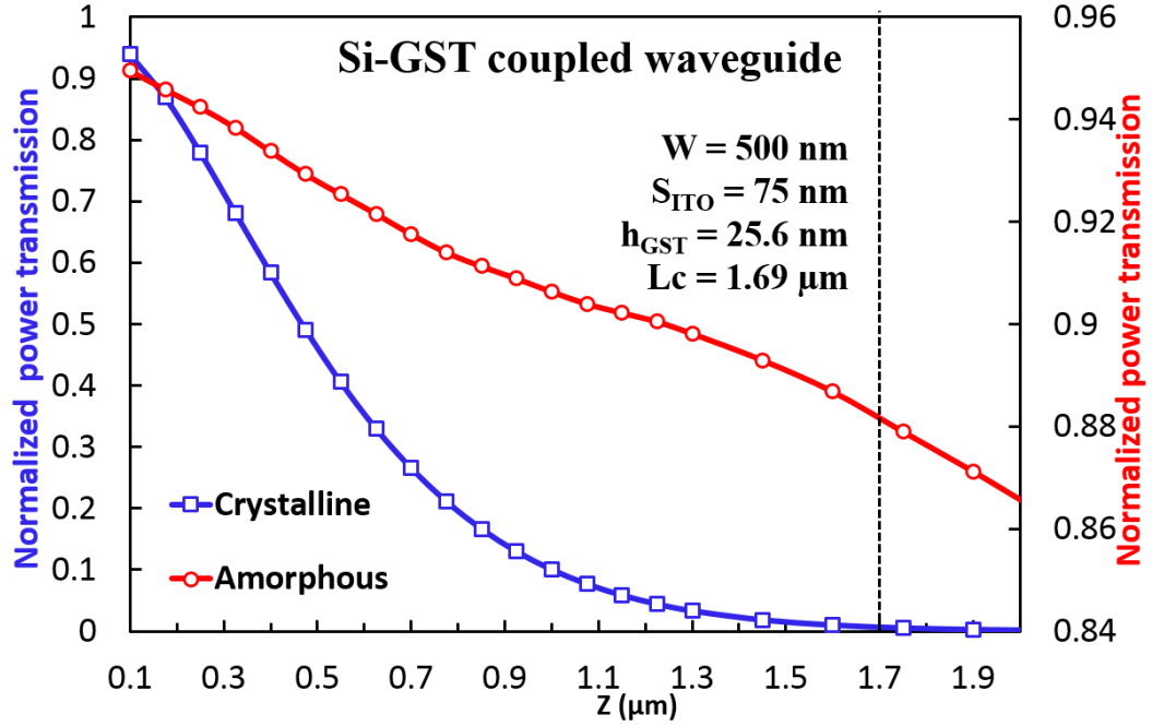
Fig. 5.13. Normalized power transmission in “ON” and “OFF” state of the switch when GST in crystalline state with S_{ITO} = 75 nm, h_{GST} = 25.6 nm and L_c = 1.7 \mu m by the FDTD simulation.
