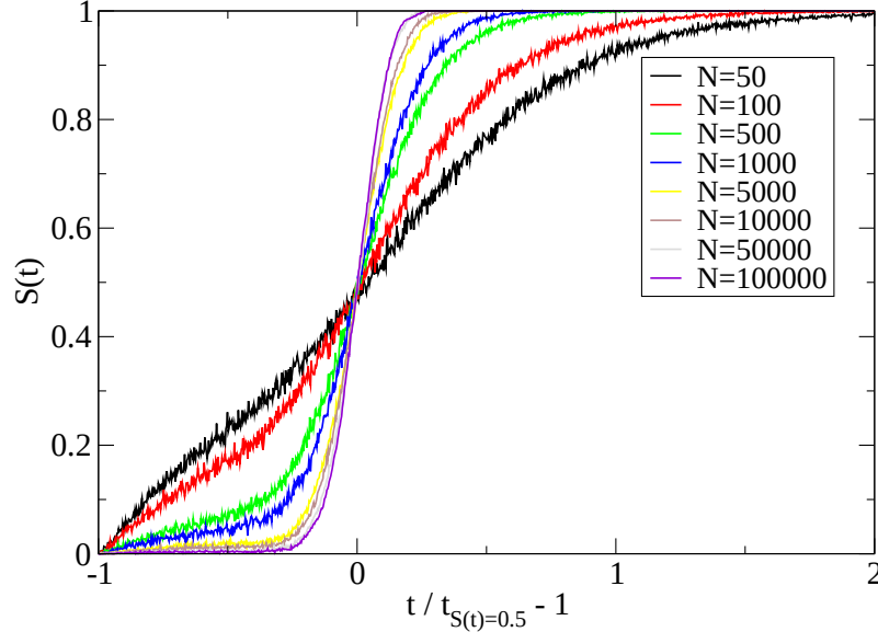
Fig. 6. Rescaling of the success rate curves. Curves relative to different system sizes show different qualitative behavior if time is rescaled as t \rightarrow t/t_{S(t)=0.5} - 1 , where t_{S(t)=0.5} \sim N^{3/2} . Indeed, on this timescale, the transition between the initial disordered state and the final ordered one where S(t) \approx 1 (i.e., the disorder-order transition) becomes steeper and steeper as N grows.
