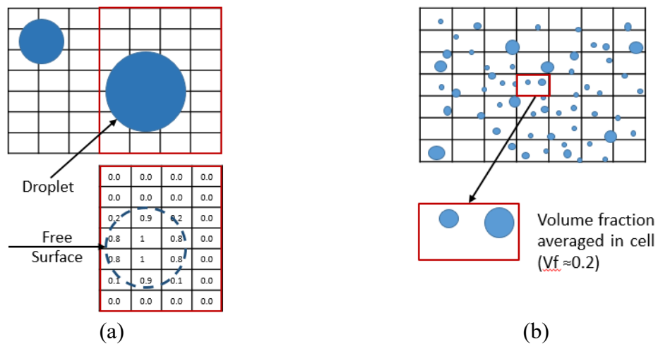
Figure 89. Droplets bigger than grid scale- VOF model and (b) droplets smaller than grid scale - Mixture and Eulerian-Eulerian model.
