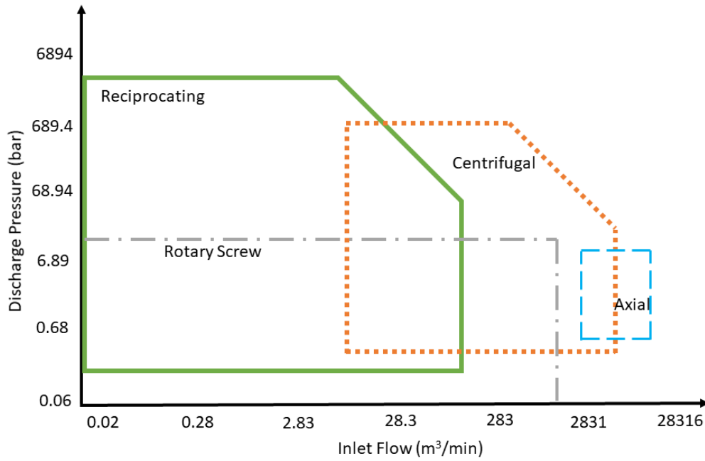
Figure 3. Application range for various types of compressors (reproduced from reference [7]).
