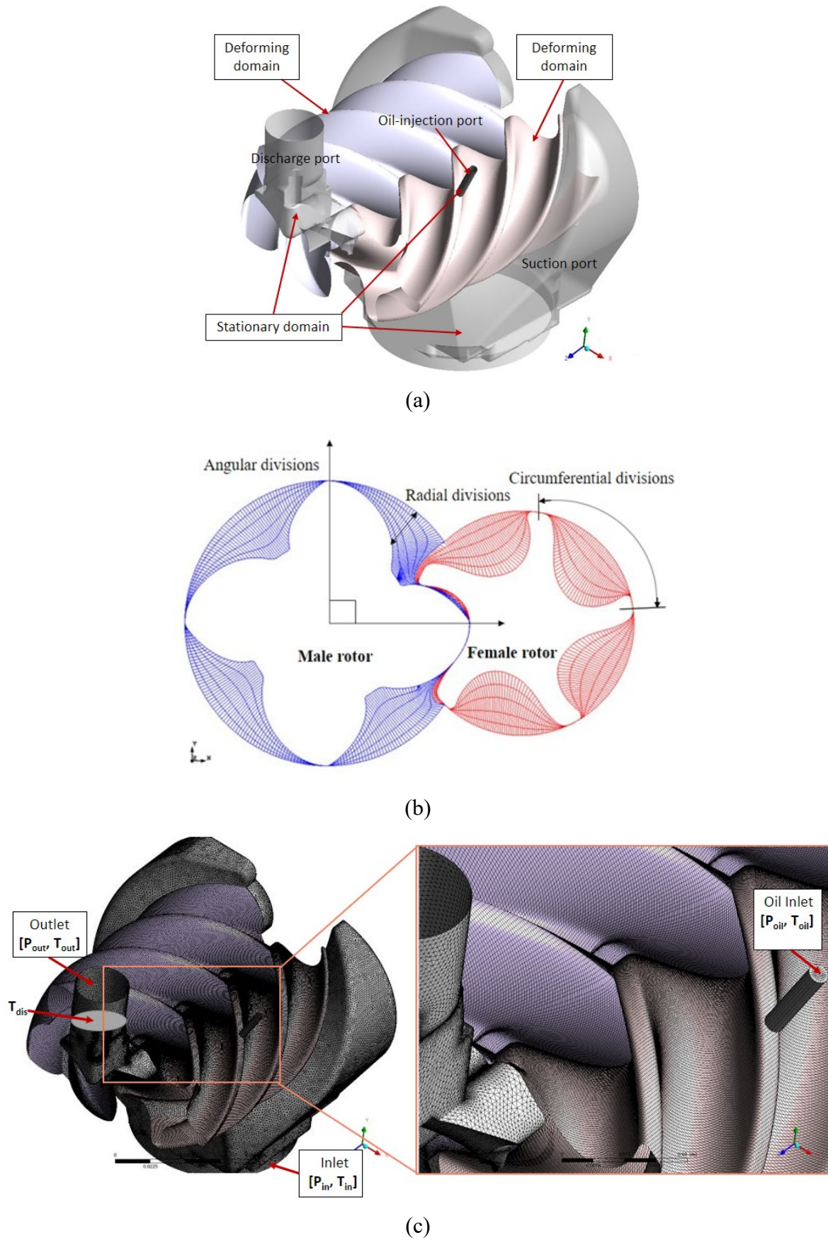
Figure 38. (a) Computational domain of the compressor, (b) rotor mesh in the transverse plane at 0° male rotor rotation and (c) grid structure of the screw compressor.
