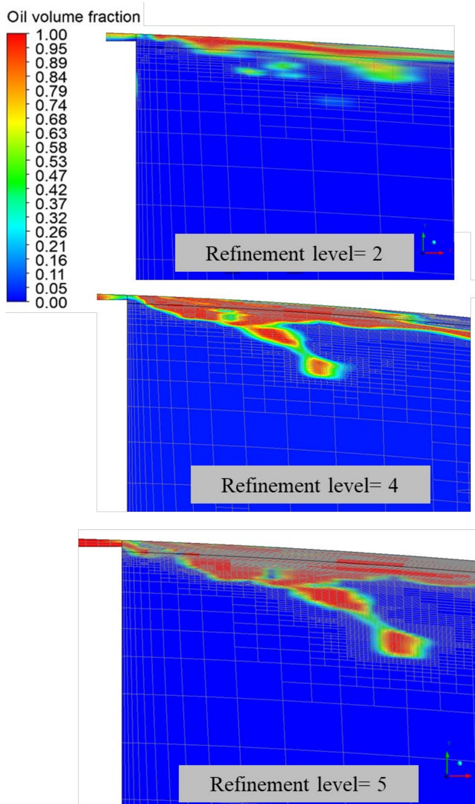
Figure 68. Oil volume fraction contour for x-y plane with refinement levels= 2,4 and 5 at time= 0.005 s.
