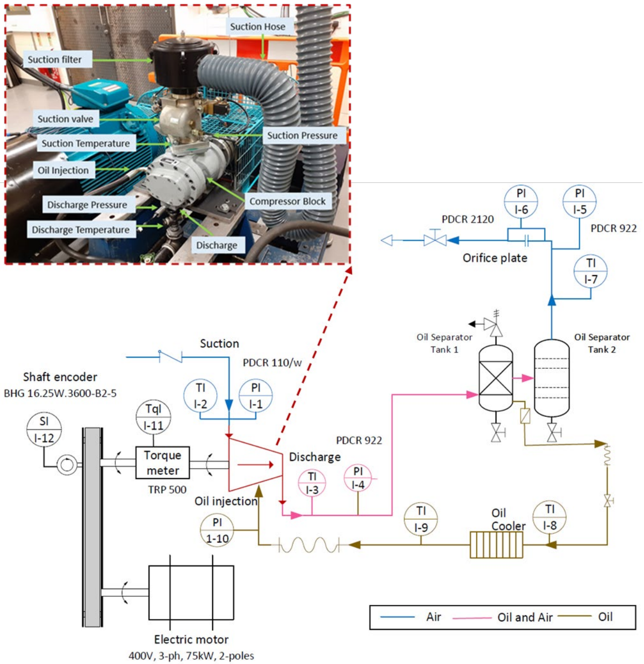
Figure 39. Layout and instrumentation of the compressor test rig.
