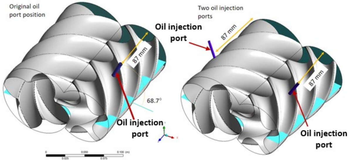
Figure 46. Positions of single and two oil injection ports.
