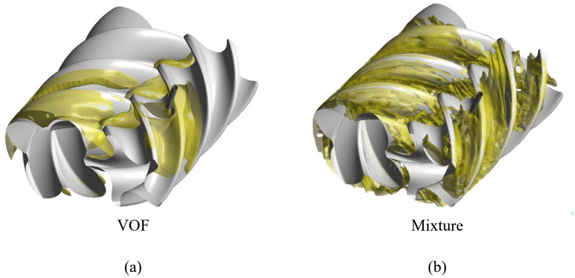
Figure 42. Oil volume fraction iso-surface of 0.035 for (a) VOF model and (b) Mixture model.
