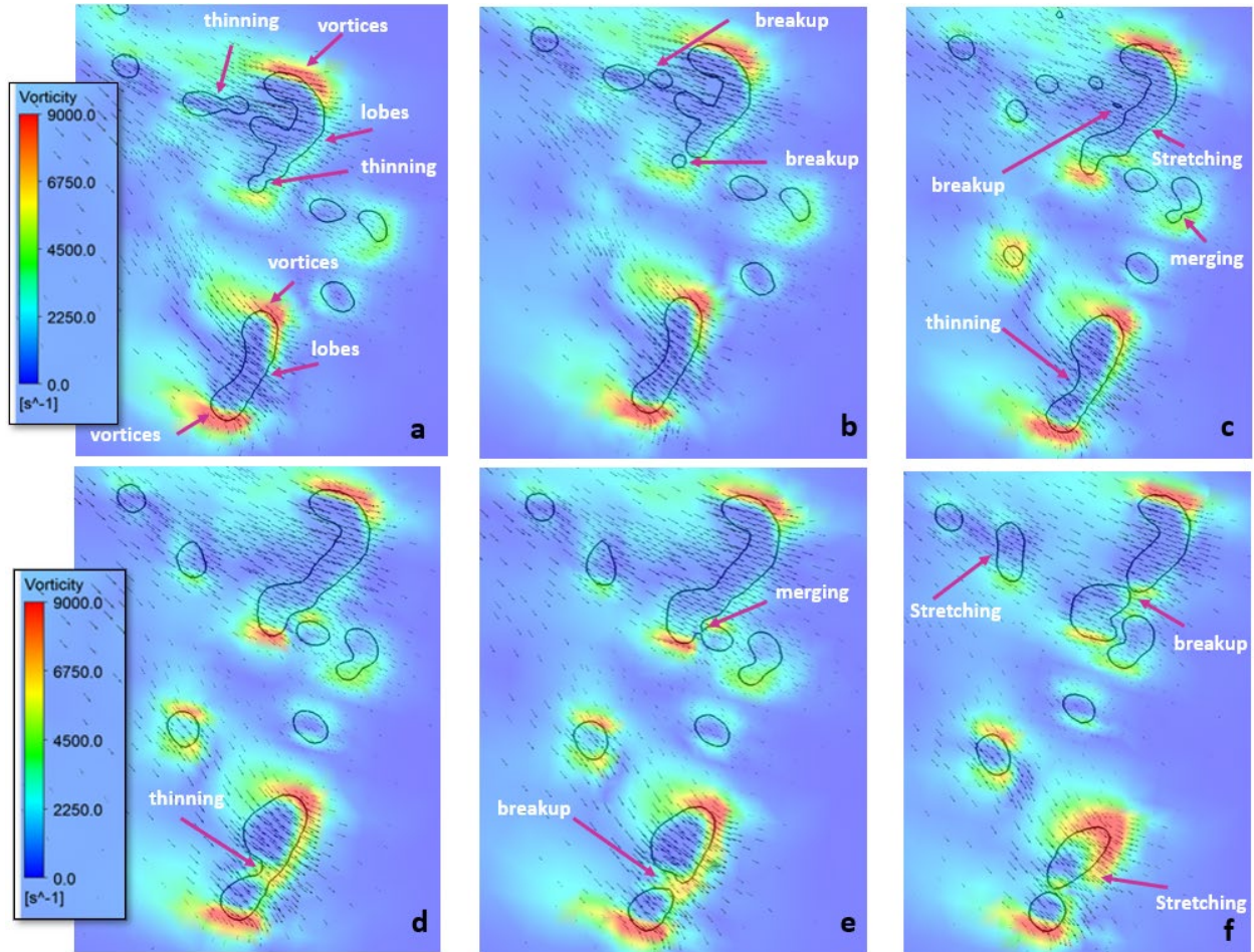
Figure 73. Breakup of secondary oil structures with vorticity contour and overlapping velocity vector.
