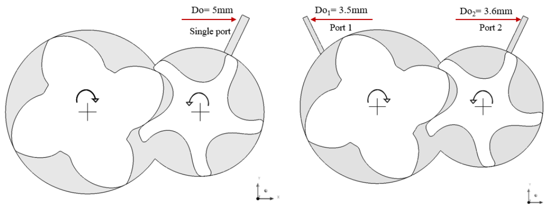
Figure 55. Oil-injection port on the rotor (cross-section at z = 0.1\text{m} ) Left: single port on the female rotor side and Right: dual port on the male and female rotor side.
