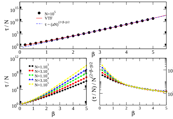
FIG. 3: MFPT for scale-free uncorrelated random networks. Here E_0 = 1 . Top: \gamma = 2.2 , N = 10^5 ; both Eq.(13) and a VTF fit (with T_0 \approx 0.023 ) are shown. Bottom: \gamma = 3 and various network sizes. For \beta < \beta_c = 1 , \tau \propto N , while \tau \propto N^{2+(\beta E_0 - \gamma)/2} for \beta > \beta_c .
