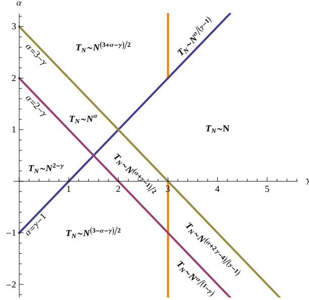
Fig. 1. Phase diagram of the heterogeneous voter model with variable opinion strengths, in which the strength of the opinion of an agent (its willingness to change opinion) is related to its degree by the relation f(k) = k^\alpha .
