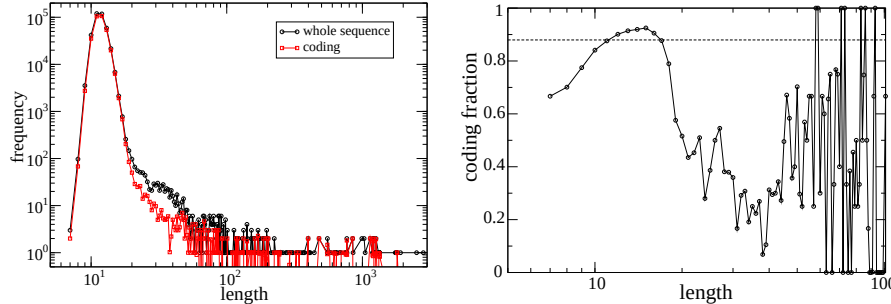
Fig. 2. Fraction of words extracted from coding regions ( Escherichia coli ). This dictionaries were extracted giving LZ77 the possibility of finding repeated sequences in the whole string. Words of lengths between 20 and 90 characters are found to belong mainly to non-coding regions.
