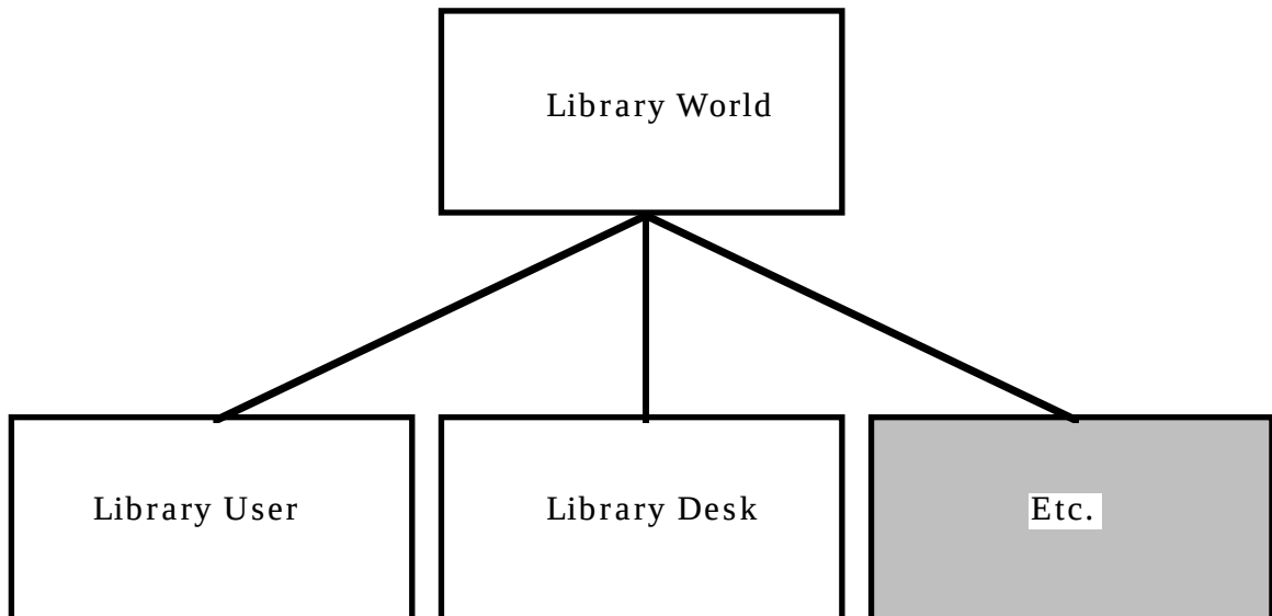
Figure 1: Simple library
