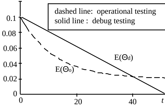
Figure 4. Subdomain testing: evolution of E(\Theta_o) and E(\Theta_d) as t increases.
