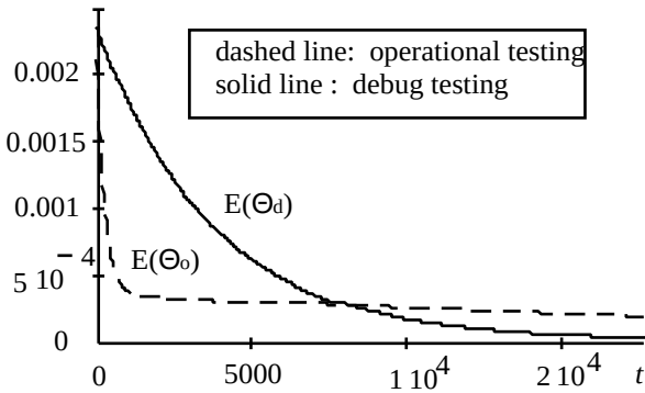
Figure 2. Evolution of E(\Theta_d) and E(\Theta_o) .
