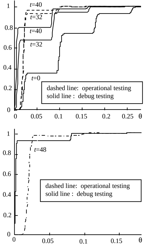
Figure 5. Cumulative distribution functions of the failure rate \Theta , before testing and then at three stages in the testing: before, at, and (lower figure) after the crossover point of the mean values (cf. Fig 4).
