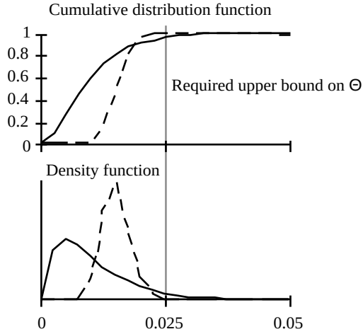
Fig. 1: Trade-off between average results and consistency of results in two hypothetical statistical distributions of the failure rates ( \Theta ) obtained after testing.
