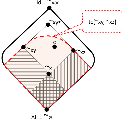
Fig. 6. Visualisation of some elements of QoI(Sto)
