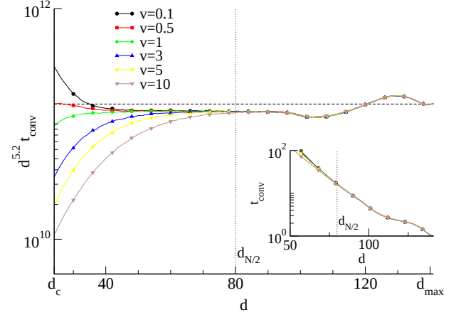
FIG. 5: (Color online) Rescaling of the consensus time, d > d_c . For large \eta > 1 and large d curves for different values of v behave as t_{conv} \sim 1/d^{5.2} as far as d (and hence \langle k \rangle ) is not too large. The behavior is better observed for smaller velocities, since large values of v reduce the value of \eta . As d > d_{N/2} the different curves collapse, and v becomes an irrelevant parameter, as shown also in the inset with non-rescaled abscissas. Horizontal dashed lines represent a constant behavior, and serve as a guide for the eye.
