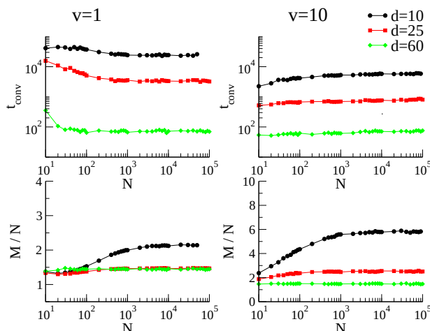
FIG. 6: (Color online) Memory usage. The average maximum memory used by each agent is plotted for different values of the velocity v . While for large mobility the individual storage capacity monotonously increases as d is reduced, small velocity induces a more complex behavior. In this case, the curves exhibit a minimum for d \simeq d_1 and a maximum for d \simeq 60 , for the usual choice of the parameters. For d > d_{N/2} curves for different velocities collapse (see Inset).
