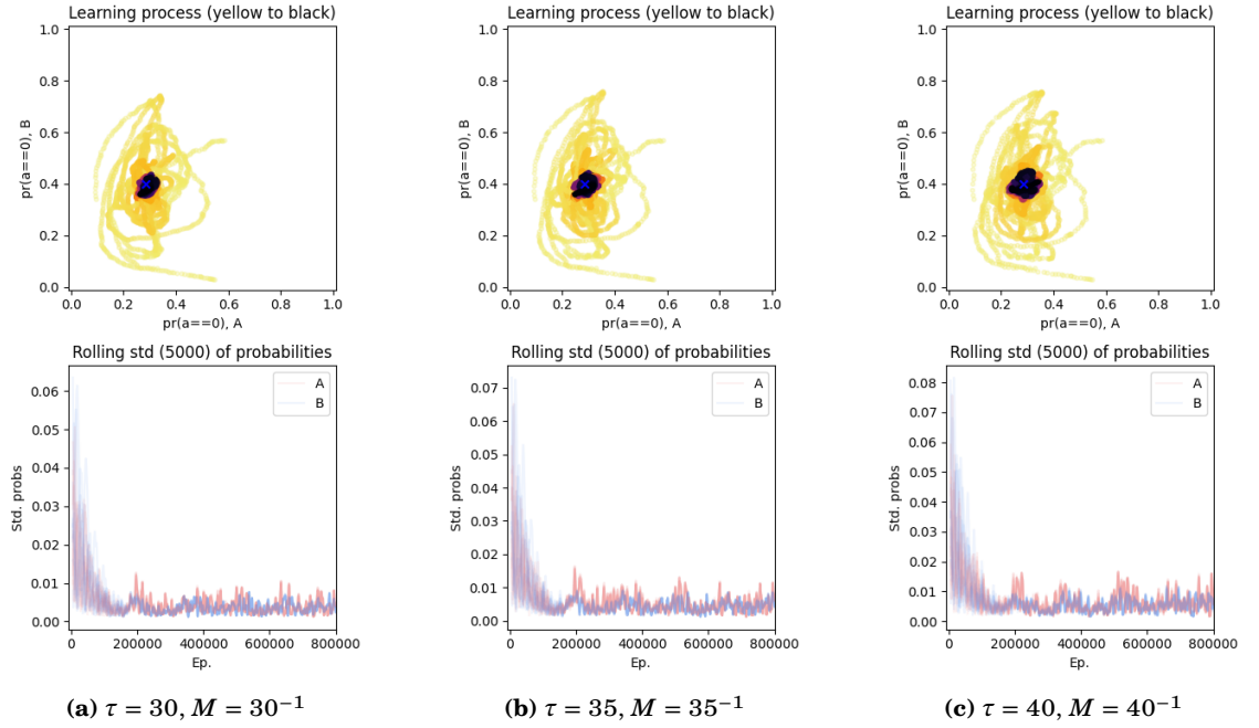
Figure 6.20: FAQ in self-play on the RPS-3 game with different values for \tau (30, 35, 40) or M ( 30^{-1} , 35^{-1} , 40^{-1} ) equivalently; \vartheta = 5 \cdot 10^{-3} ; for 10 different initialisations.
