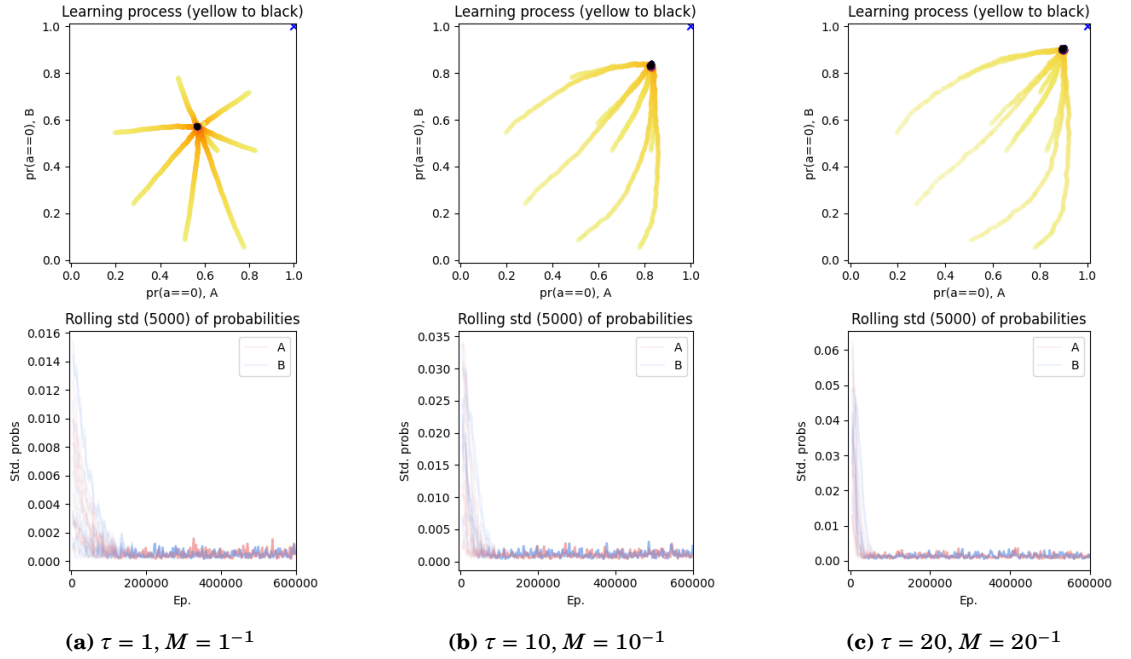
Figure 6.3: MBL-LC in self-play on the PD game with different values for \tau (1, 10, 20) or M ( 1 , 10^{-1} , 20^{-1} ) equivalently; \vartheta = 5 \cdot 10^{-3} ; for 10 different initialisations. (See figure 6.1 for a detailed explanation of the graphs.)
