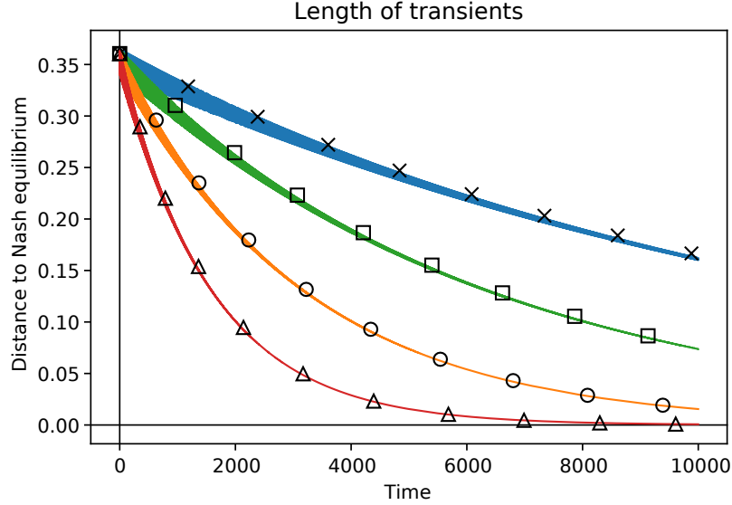
Figure 5.1: Four solutions of (5.2.1) for the matching pennies game in example 5.2.5 with different mutation strengths M_X = M_Y = M . The coloured lines show the distance of the solution to the Nash equilibrium (1/2, 1/2) , with red, orange, green and blue lines corresponding to solutions for M -values of 2^{-4} \cdot 10^{-2} , 2^{-5} \cdot 10^{-2} , 2^{-6} \cdot 10^{-2} and 2^{-7} \cdot 10^{-2} , respectively. Lines appear thicker at the start as the distance fluctuates stronger. The shapes ‘ \Delta ’, ‘ \circ ’, ‘ \square ’ and ‘ \times ’ show the values of the exponential decay function C_0 \cdot e^{-M \cdot t} with appropriate scaling constant C_0 for corresponding M -values of 2^{-4} \cdot 10^{-2} , 2^{-5} \cdot 10^{-2} , 2^{-6} \cdot 10^{-2} and 2^{-7} \cdot 10^{-2} , respectively.
