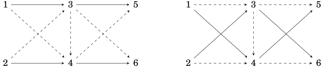
Figure 3.5: Expected interaction graphs for |I| = |J| = 2 , |P| = 2 , where dashed edges have weights close to zero.
