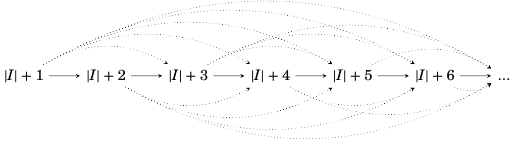
Figure 3.1: Schematic illustration of the induced subgraph of agents in P .
