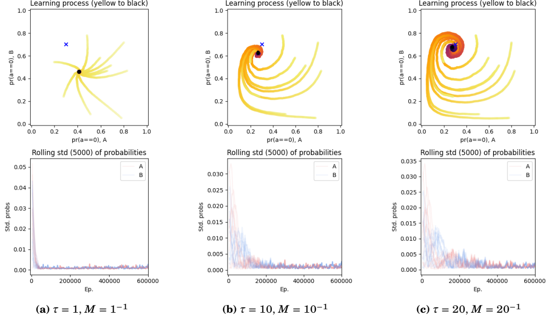
Figure 6.8: MBL-DPU in self-play on the MP game with different values for \tau (1, 10, 20) or M ( 10^{-1} , 20^{-1} ) equivalently; \vartheta = 10^{-4} ; for 10 different initialisations. (See figure 6.1 for a detailed explanation of the graphs.)
