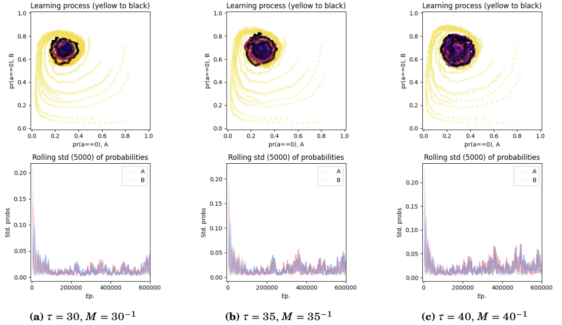
Figure 6.11: MBL-LC in self-play on the MP game with different values for \tau (30, 35, 40) or M ( 30^{-1} , 35^{-1} , 40^{-1} ) equivalently; \vartheta = 5 \cdot 10^{-3} ; for 10 different initialisations. (See figure 6.1 for a detailed explanation of the graphs.)
