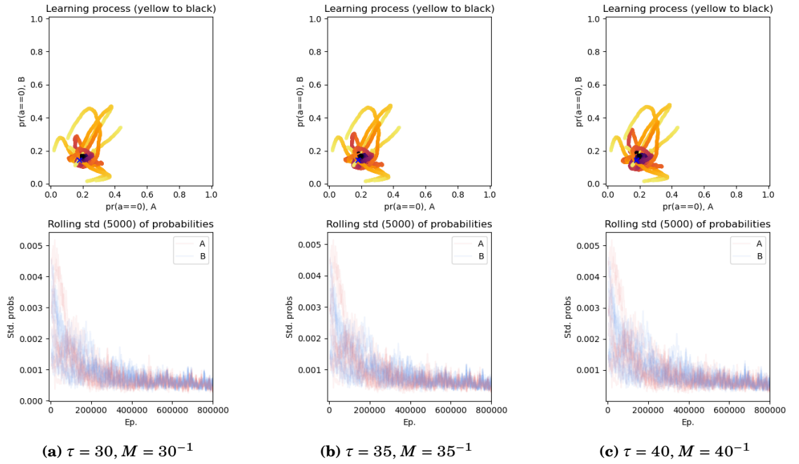
Figure 6.23: MBL-DPU in self-play on the RPS-5 game with different values for \tau (30, 35, 40) or M ( 30^{-1} , 35^{-1} , 40^{-1} ) equivalently; \vartheta = 10^{-4} ; for 10 different initialisations.
