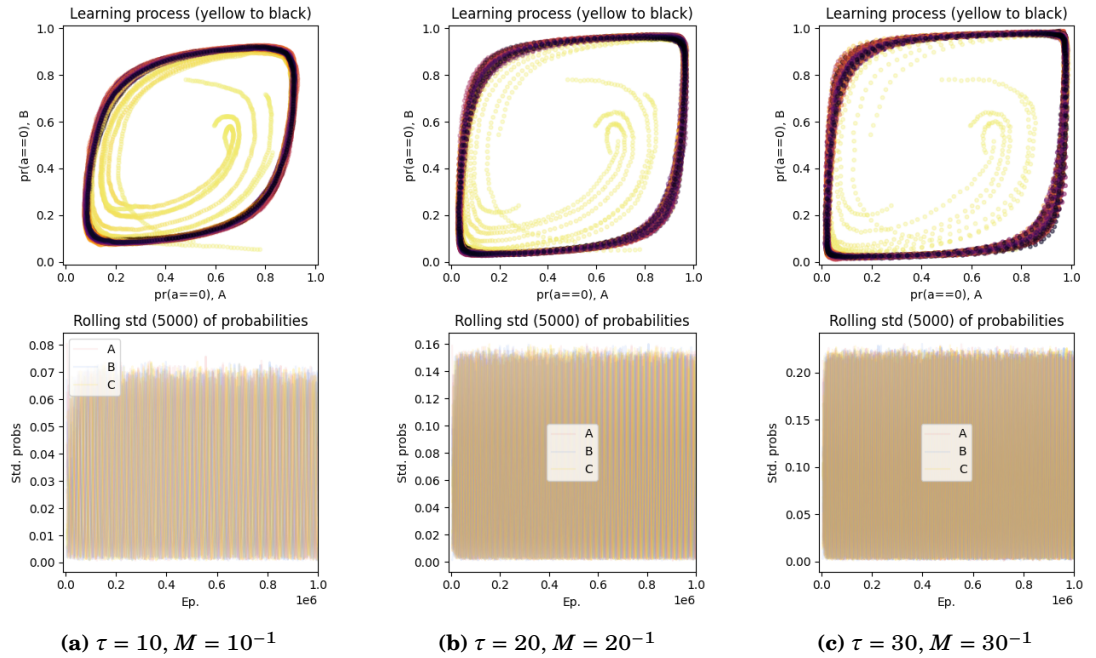
Figure 6.37: MBL-LC in self-play on the 3MP game with different values for \tau (10, 20, 30) or M ( 10^{-1} , 20^{-1} , 30^{-1} ) equivalently; \vartheta = 10^{-4} ; for 10 different initialisations. (See figure 6.1 for a detailed explanation of the graphs.)
