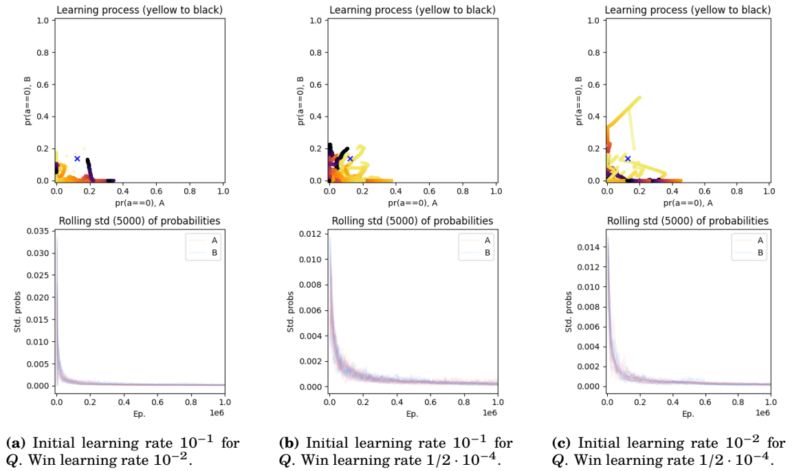
Figure 6.35: WoLF-PHC in self-play on the RPS-9 game with different learning schedules; for 10 different initialisations. (See figure 6.1 for a detailed explanation of the graphs.)
