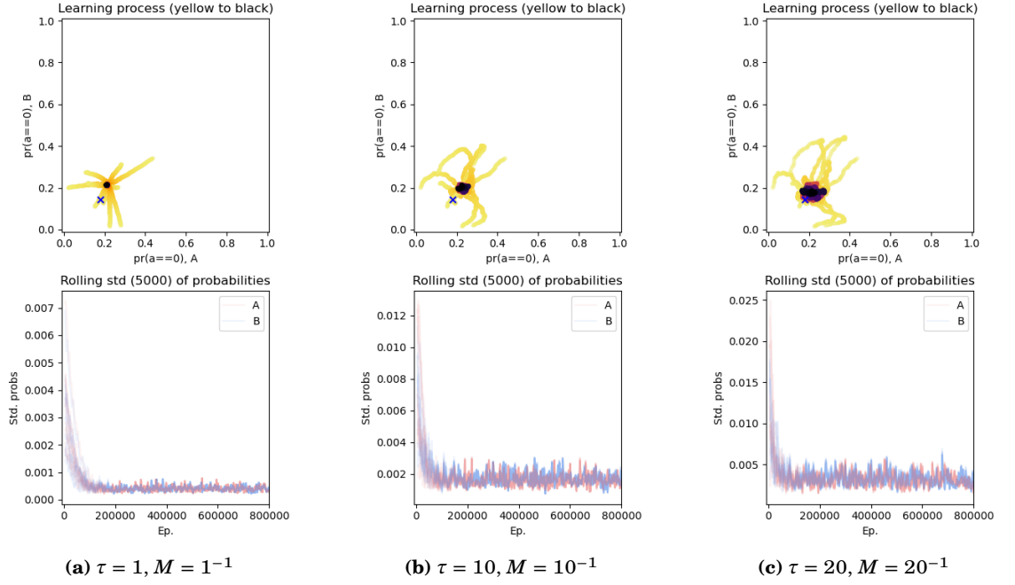
Figure 6.24: MBL-LC in self-play on the RPS-5 game with different values for \tau (1, 10, 20) or M ( 1 , 10^{-1} , 20^{-1} ) equivalently; \vartheta = 5 \cdot 10^{-3} ; for 10 different initialisations. (See figure 6.1 for a detailed explanation of the graphs.)
