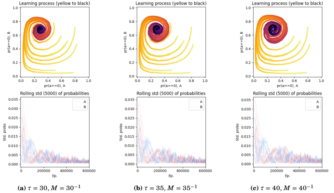
Figure 6.9: MBL-DPU in self-play on the MP game with different values for \tau (30, 35, 40) or M ( 30^{-1} , 35^{-1} , 40^{-1} ) equivalently; \vartheta = 10^{-4} ; for 10 different initialisations. (See figure 6.1 for a detailed explanation of the graphs.)
