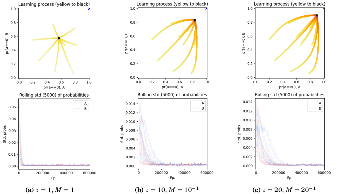
Figure 6.1: MBL-DPU in self-play on the PD game with different values for \tau (1, 10, 20) or M (1, 10^{-1} , 20^{-1} ) equivalently; \vartheta = 10^{-4} ; for 10 different initial conditions. In each subfigure, the upper graph shows the ten trajectories in the projection on the first components of the players' strategies, in this case the 'defect' strategy, with the first player given on the horizontal axis and the second player on the vertical axis. Points coloured yellow correspond to earlier points in time, changing over orange and violet to black for later points in time. The position of the game's Nash equilibrium is marked with a blue cross in the projection plane. The lower graph shows the standard deviation of all components of the players' strategies for each point in time over the past 5000 time steps, for each of the ten initial conditions, coloured red and blue for the two players. Time is given on the horizontal axis. The standard deviation is computed with the usual Euclidean metric.
