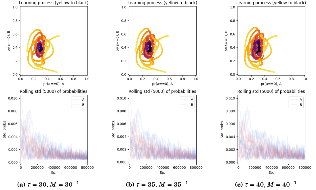
Figure 6.16: MBL-DPU in self-play on the RPS-3 game with different values for \tau (30, 35, 40) or M ( 30^{-1} , 35^{-1} , 40^{-1} ) equivalently; \vartheta = 10^{-4} ; for 10 different initialisations. (See figure 6.1 for a detailed explanation of the graphs.)
