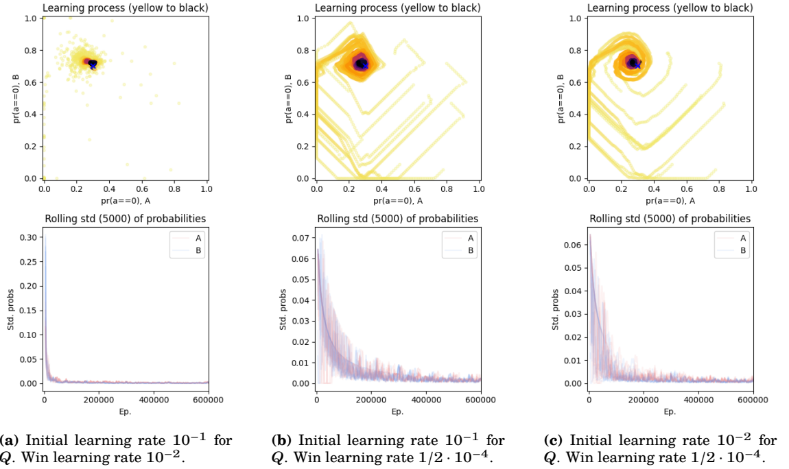
Figure 6.14: WoLF-PHC in self-play on the MP game with different learning schedules; for 10 different initialisations. (See figure 6.1 for a detailed explanation of the graphs.)
