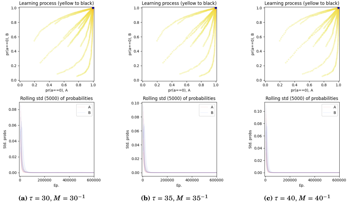
Figure 6.6: FAQ in self-play on the PD game with different values for \tau (30, 35, 40) or M ( 30^{-1} , 35^{-1} , 40^{-1} ) equivalently; \vartheta = 5 \cdot 10^{-3} ; for 10 different initialisations. (See figure 6.1 for a detailed explanation of the graphs.)
