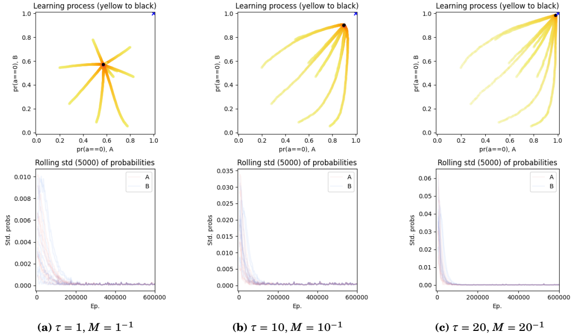
Figure 6.5: FAQ in self-play on the PD game with different values for \tau (1, 10, 20) or M ( 1, 10^{-1}, 20^{-1} ) equivalently; \vartheta = 5 \cdot 10^{-3} ; for 10 different initialisations. (See figure 6.1 for a detailed explanation of the graphs.)
