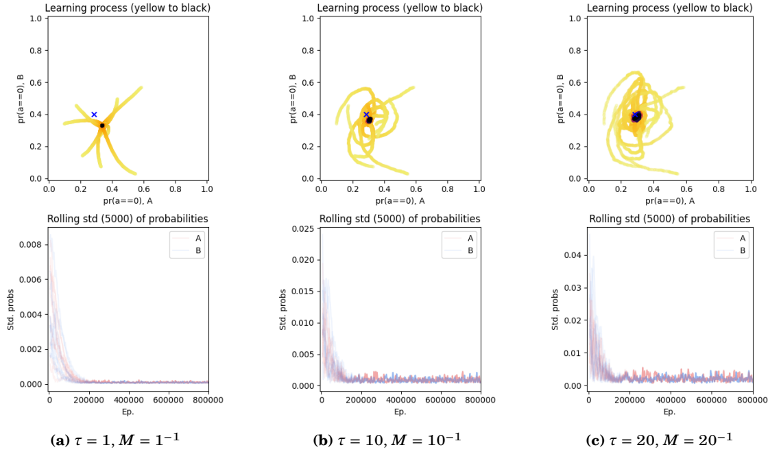
Figure 6.19: FAQ in self-play on the RPS-3 game with different values for \tau (1, 10, 20) or M ( 1 , 10^{-1} , 20^{-1} ) equivalently; \vartheta = 5 \cdot 10^{-3} ; for 10 different initialisations. (See figure 6.1 for a detailed explanation of the graphs.)
