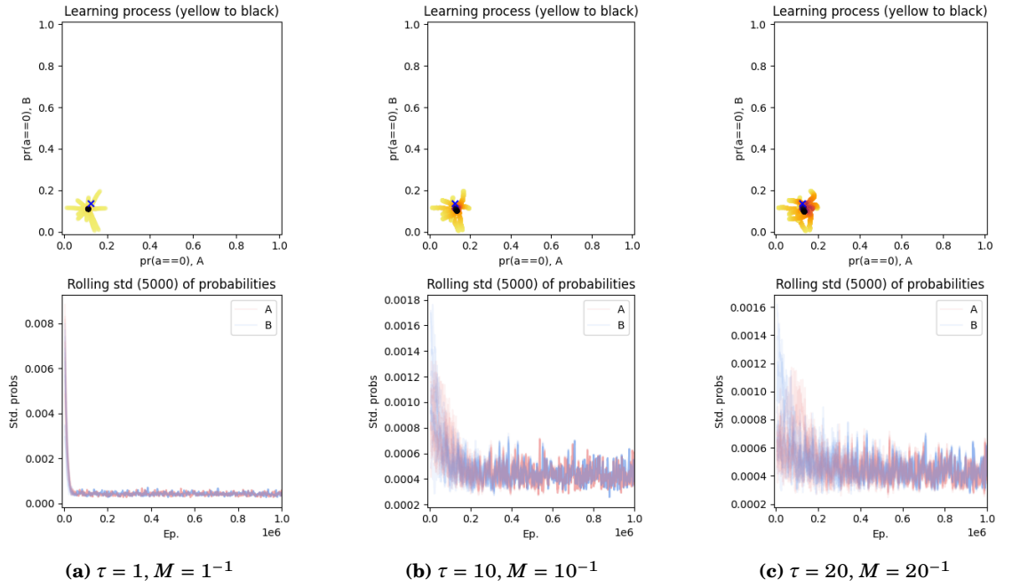
Figure 6.29: MBL-DPU in self-play on the RPS-9 game with different values for \tau (1, 10, 20) or M (1, 10^{-1} , 20^{-1} ) equivalently; \vartheta = 10^{-4} ; for 10 different initialisations. (See figure 6.1 for a detailed explanation of the graphs.)
