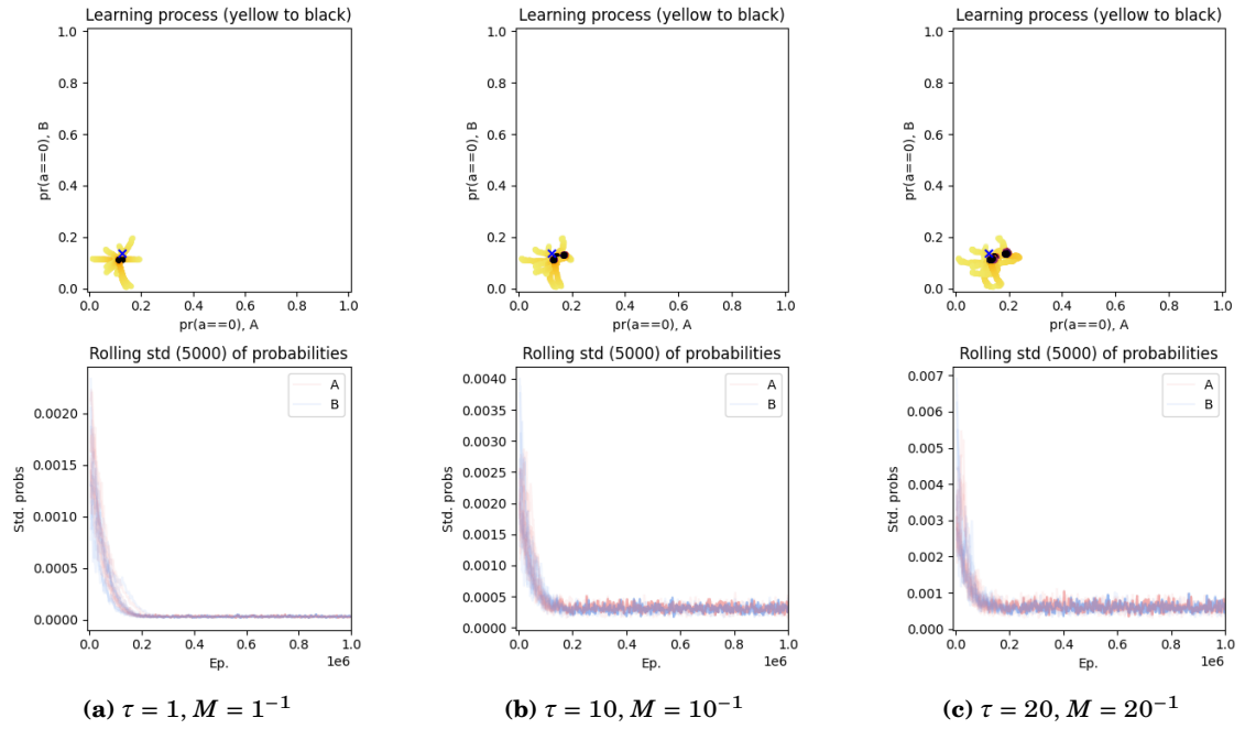
Figure 6.33: FAQ in self-play on the RPS-9 game with different values for \tau (1, 10, 20) or M (1, 10^{-1} , 20^{-1} ) equivalently; \vartheta = 5 \cdot 10^{-3} ; for 10 different initialisations. (See figure 6.1 for a detailed explanation of the graphs.)
