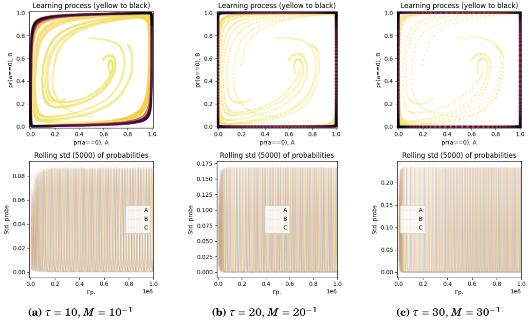
Figure 6.38: FAQ in self-play on the 3MP game with different values for \tau (10, 20, 30) or M ( 10^{-1} , 20^{-1} , 30^{-1} ) equivalently; \vartheta = 10^{-4} ; for 10 different initialisations.
