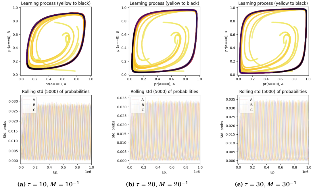
Figure 6.36: MBL-DPU in self-play on the 3MP game with different values for \tau (10, 20, 30) or M ( 10^{-1} , 20^{-1} , 30^{-1} ) equivalently; \vartheta = 10^{-4} ; for 10 different initialisations. (See figure 6.1 for a detailed explanation of the graphs.)
