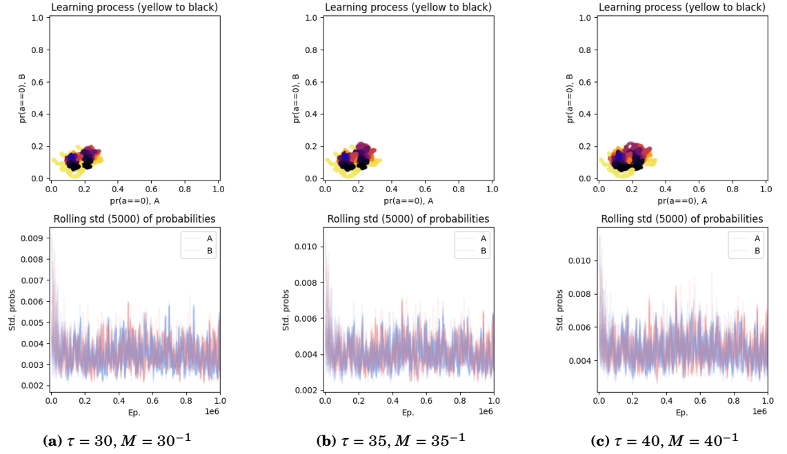
Figure 6.32: MBL-LC in self-play on the RPS-9 game with different values for \tau (30, 35, 40) or M ( 30^{-1} , 35^{-1} , 40^{-1} ) equivalently; \vartheta = 5 \cdot 10^{-3} ; for 10 different initialisations.
