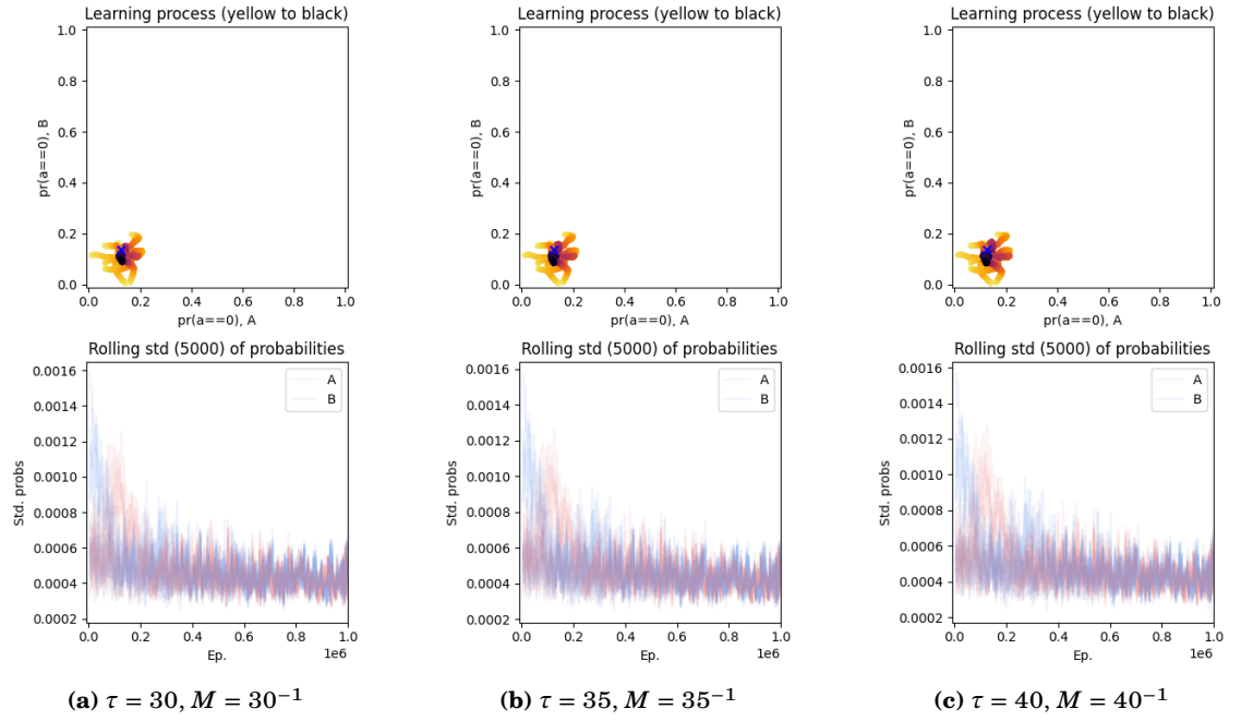
Figure 6.30: MBL-DPU in self-play on the RPS-9 game with different values for \tau (30, 35, 40) or M ( 30^{-1} , 35^{-1} , 40^{-1} ) equivalently; \vartheta = 10^{-4} ; for 10 different initialisations.
