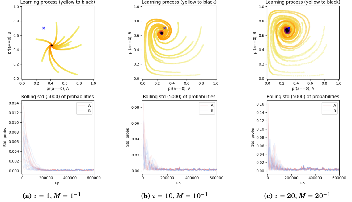
Figure 6.12: FAQ in self-play on the MP game with different values for \tau (1, 10, 20) or M ( 10^{-1} , 20^{-1} ) equivalently; \vartheta = 5 \cdot 10^{-3} ; for 10 different initialisations. (See figure 6.1 for a detailed explanation of the graphs.)
