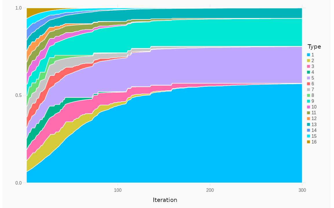
Figure 3.6: Evolution of population composition (abscissa) over time for first 300 generations, where the vertical distance along the ordinate between type boundaries gives the proportion in the population.
