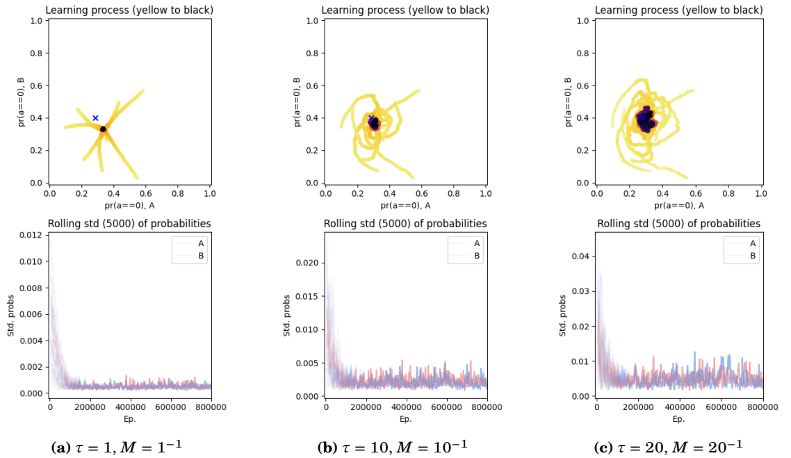
Figure 6.17: MBL-LC in self-play on the RPS-3 game with different values for \tau (1, 10, 20) or M ( 1, 10^{-1}, 20^{-1} ) equivalently; \vartheta = 5 \cdot 10^{-3} ; for 10 different initialisations. (See figure 6.1 for a detailed explanation of the graphs.)
