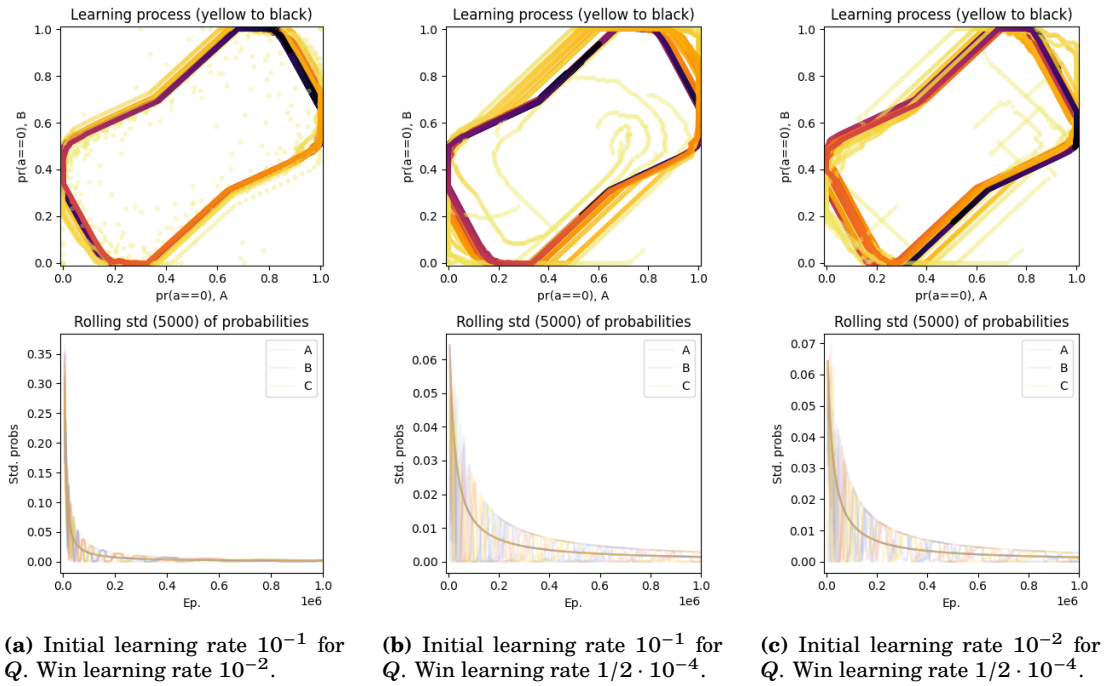
Figure 6.39: WoLF-PHC in self-play on the 3MP game with different learning schedules; for 10 different initialisations. (See figure 6.1 for a detailed explanation of the graphs.)
