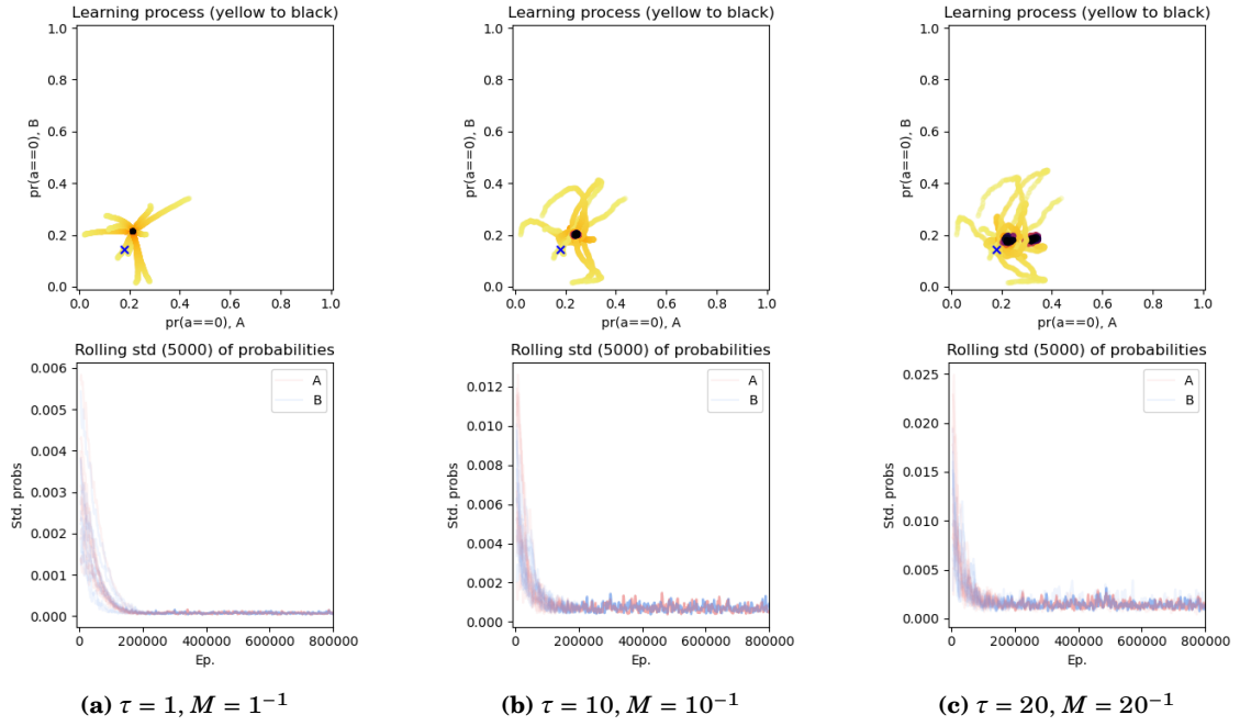
Figure 6.26: FAQ in self-play on the RPS-5 game with different values for \tau (1, 10, 20) or M ( 10^{-1} , 20^{-1} ) equivalently; \vartheta = 5 \cdot 10^{-3} ; for 10 different initialisations.
