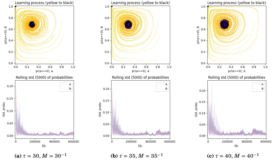
Figure 6.13: FAQ in self-play on the MP game with different values for \tau (30, 35, 40) or M ( 30^{-1} , 35^{-1} , 40^{-1} ) equivalently; \vartheta = 5 \cdot 10^{-3} ; for 10 different initialisations. (See figure 6.1 for a detailed explanation of the graphs.)
