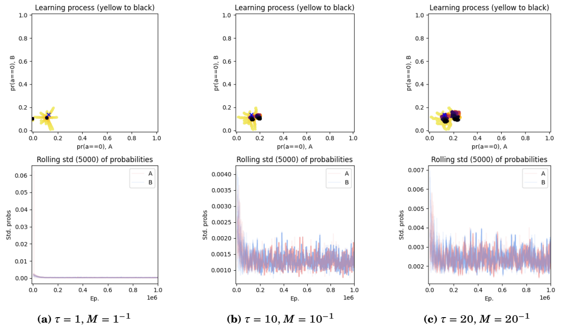
Figure 6.31: MBL-LC in self-play on the RPS-9 game with different values for \tau (1, 10, 20) or M (1, 10^{-1} , 20^{-1} ) equivalently; \vartheta = 5 \cdot 10^{-3} ; for 10 different initialisations. (See figure 6.1 for a detailed explanation of the graphs.)
