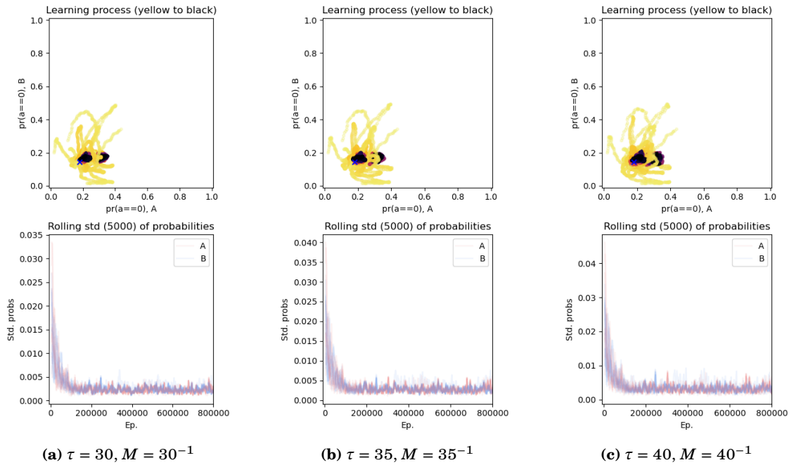
Figure 6.27: FAQ in self-play on the RPS-5 game with different values for \tau (30, 35, 40) or M ( 30^{-1} , 35^{-1} , 40^{-1} ) equivalently; \vartheta = 5 \cdot 10^{-3} ; for 10 different initialisations. (See figure 6.1 for a detailed explanation of the graphs.)
