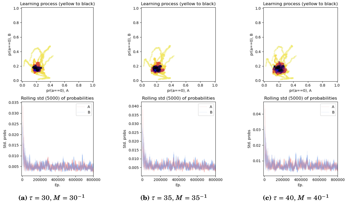
Figure 6.25: MBL-LC in self-play on the RPS-5 game with different values for \tau (30, 35, 40) or M ( 30^{-1} , 35^{-1} , 40^{-1} ) equivalently; \vartheta = 5 \cdot 10^{-3} ; for 10 different initialisations. (See figure 6.1 for a detailed explanation of the graphs.)
