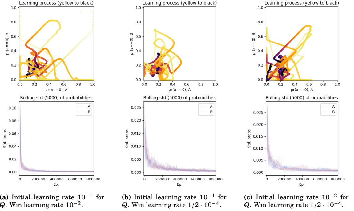
Figure 6.28: WoLF-PHC in self-play on the RPS-5 game with different learning schedules; for 10 different initialisations.
