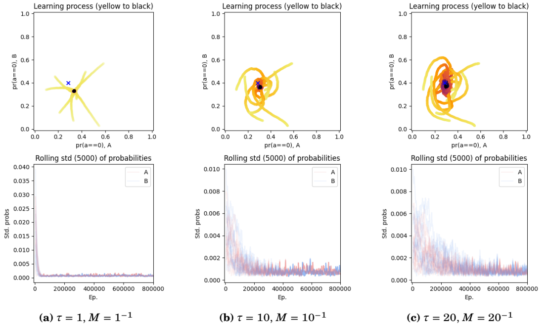
Figure 6.15: MBL-DPU in self-play on the RPS-3 game with different values for \tau (1, 10, 20) or M ( 1, 10^{-1}, 20^{-1} ) equivalently; \vartheta = 10^{-4} ; for 10 different initialisations. (See figure 6.1 for a detailed explanation of the graphs.)
