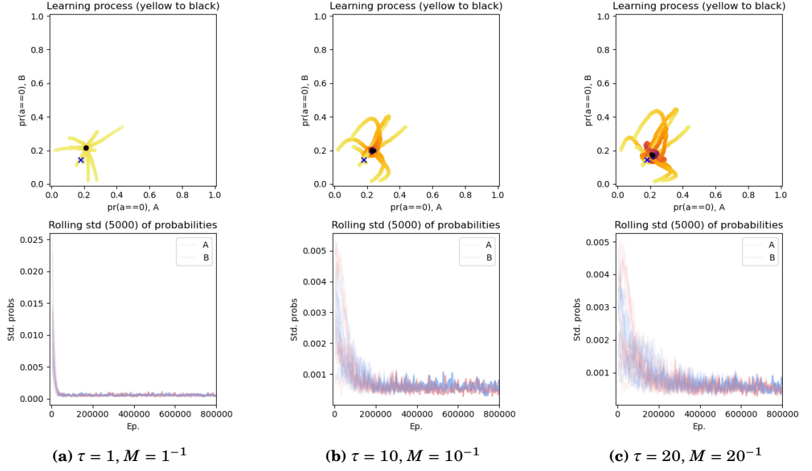
Figure 6.22: MBL-DPU in self-play on the RPS-5 game with different values for \tau (1, 10, 20) or M (1, 10^{-1} , 20^{-1} ) equivalently; \vartheta = 10^{-4} ; for 10 different initialisations. (See figure 6.1 for a detailed explanation of the graphs.)
