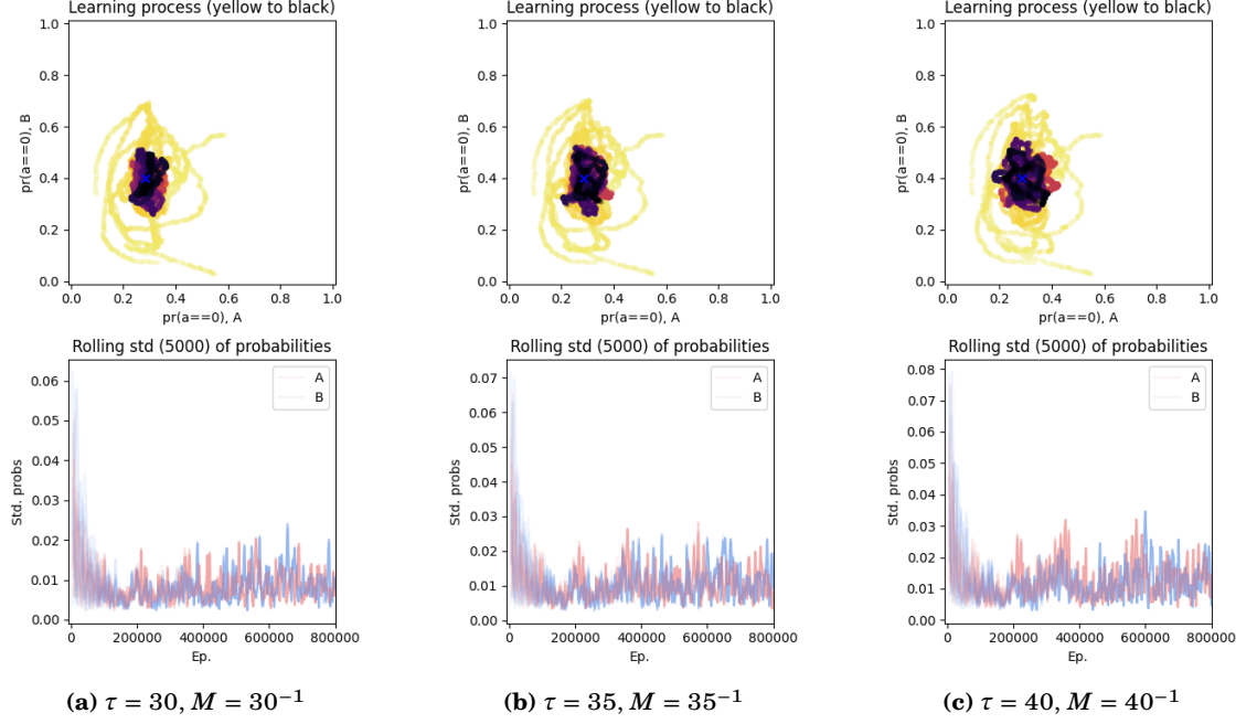
Figure 6.18: MBL-LC in self-play on the RPS-3 game with different values for \tau (30, 35, 40) or M ( 30^{-1} , 35^{-1} , 40^{-1} ) equivalently; \vartheta = 5 \cdot 10^{-3} ; for 10 different initialisations. (See figure 6.1 for a detailed explanation of the graphs.)
