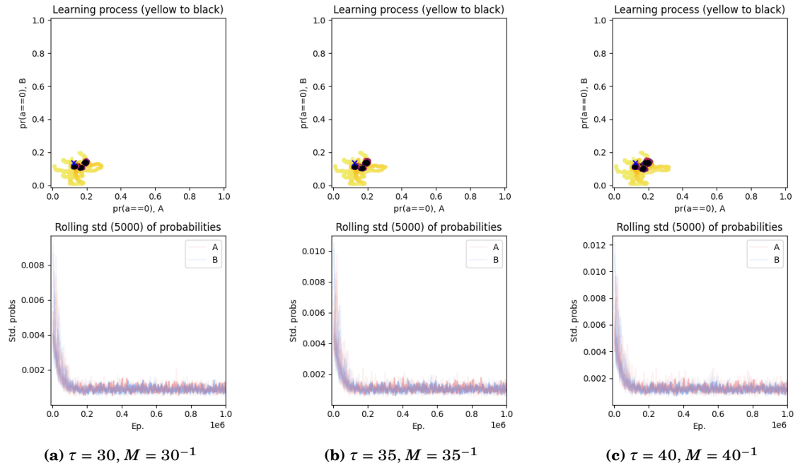
Figure 6.34: FAQ in self-play on the RPS-9 game with different values for \tau (30, 35, 40) or M ( 30^{-1} , 35^{-1} , 40^{-1} ) equivalently; \vartheta = 5 \cdot 10^{-3} ; for 10 different initialisations.
