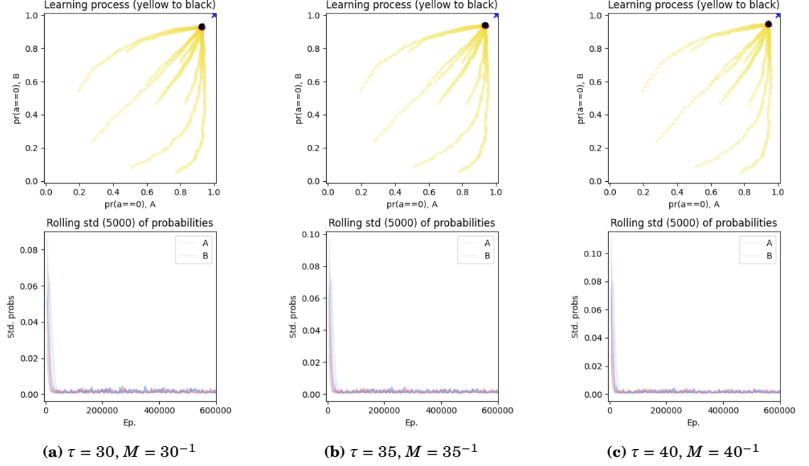
Figure 6.4: MBL-LC in self-play on the PD game with different values for \tau (30, 35, 40) or M ( 30^{-1} , 35^{-1} , 40^{-1} ) equivalently; \vartheta = 5 \cdot 10^{-3} ; for 10 different initialisations. (See figure 6.1 for a detailed explanation of the graphs.)
