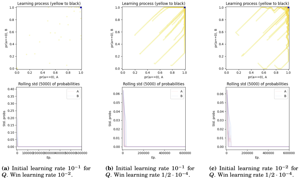
Figure 6.7: WoLF-PHC in self-play on the PD game with different learning schedules; for 10 different initialisations. Subgraph (a) has a high convergence speed such that only disconnected points can be seen. (See figure 6.1 for a detailed explanation of the graphs.)
