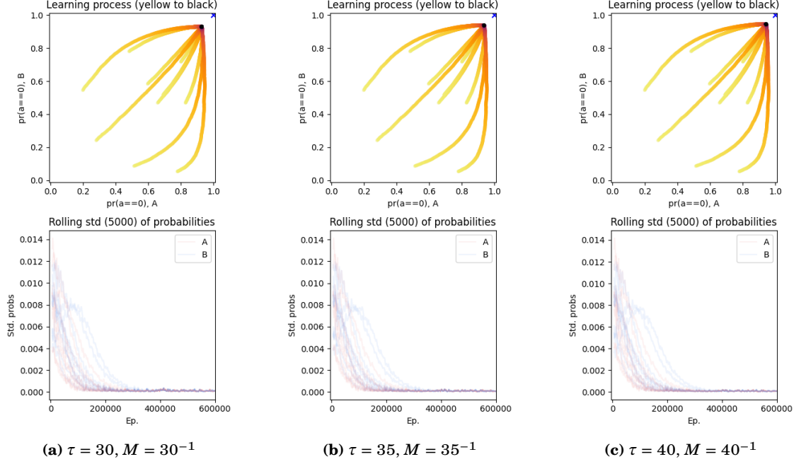
Figure 6.2: MBL-DPU in self-play on the PD game with different values for \tau (30, 35, 40) or M ( 30^{-1} , 35^{-1} , 40^{-1} ) equivalently; \vartheta = 10^{-4} ; for 10 different initialisations. (See figure 6.1 for a detailed explanation of the graphs.)
