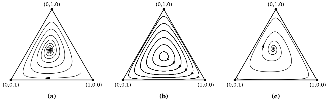
Figure 2.1: Three possible situations resulting from the continuous single-population replicator dynamics with different payoffs in the Rock-Paper-Scissors game. (a) An asymptotically stable and globally attracting stationary point results from payoff matrix A_1 . (b) For the conventional choice for payoffs A_2 , a Lyapunov stable but not asymptotically stable stationary point with closed orbits results. (c) For A_3 , an unstable and globally repelling stationary point results.
