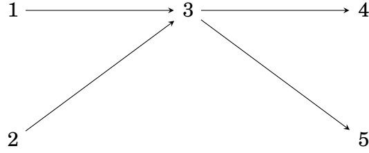
Figure 3.3: Interaction graph in the case of |I| = |J| = 2 and |P| = 1 .
