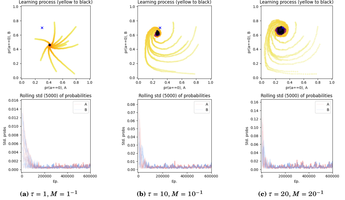
Figure 6.10: MBL-LC in self-play on the MP game with different values for \tau (1, 10, 20) or M ( 10^{-1} , 20^{-1} ) equivalently; \vartheta = 5 \cdot 10^{-3} ; for 10 different initialisations. (See figure 6.1 for a detailed explanation of the graphs.)
