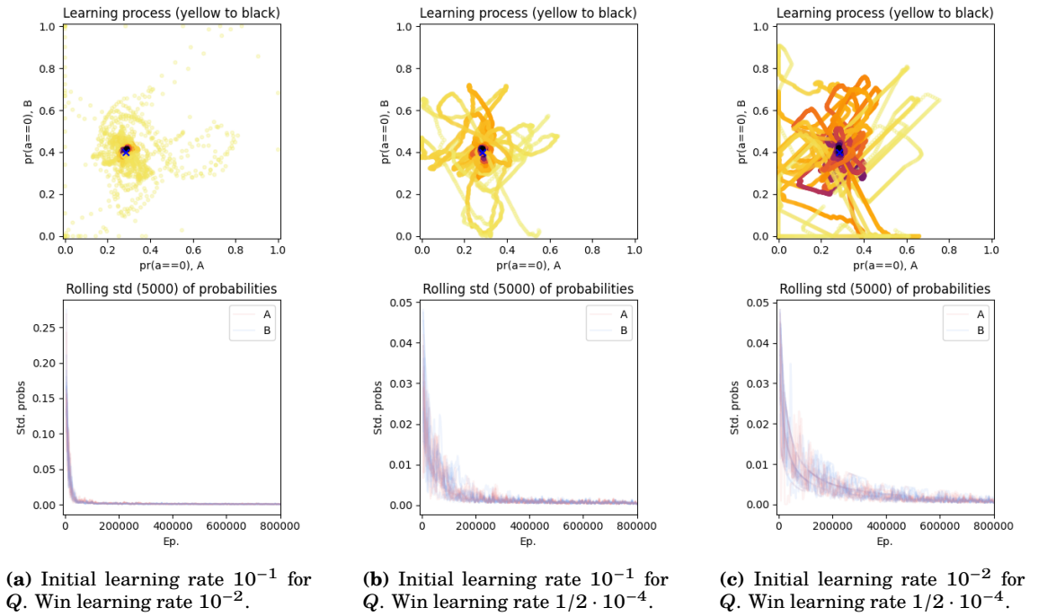
Figure 6.21: WoLF-PHC in self-play on the RPS-3 game with different learning schedules; for 10 different initialisations. (See figure 6.1 for a detailed explanation of the graphs.)
