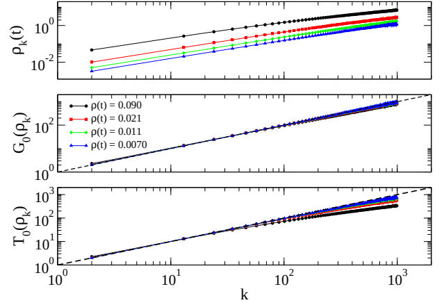
FIG. 5: Density spectra of the bosonic RD process 2A \rightarrow \emptyset on uncorrelated UCM networks with \gamma = 2.5 . Network size N = 10^6 . Top: Density spectra as a function of the degree k at different times (densities) from measures performed with fixed parameter \lambda = 0.1 . The curves show a bending in the large k region for short times (large densities). Center: Data collapse of the density spectra at different times as predicted by Eq. (82). Bottom: Check of the Taylor expansion of the density spectra, as given by Eq. (83). The poor collapse at large k confirms the presence of strong nonlinear terms at short times.
