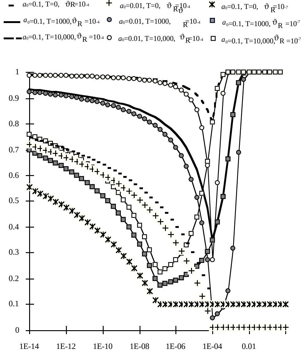
Figure 4 Probability P_{\text{succ}}(T) that the failure intensity \Theta of the program under test is lower than \vartheta_R , as a function of the lower bound on the failure intensity, \vartheta_1 . The probability of correctness, a_0 , is kept constant, and the logarithm of \Theta is uniformly distributed between \log(\vartheta_1) and 0. Notice that the curves to the right of the point \vartheta_1 = \vartheta_R are just the curves of b_0 = P(\Theta = 0) , since \vartheta_1 > \vartheta_R means that all acceptable, non-zero failure intensities have zero probability.
