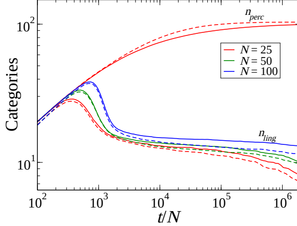
Fig. 2. Perceptual and linguistic categories obtained from the old and the new algorithm for N = 25, 50 and 100 . Solid lines show results obtained from the old algorithm while broken lines indicate results obtained from the new algorithm. All the results are averaged over 30 samples.
