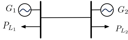
FIGURE 10 One-line diagram of a two-generator and two-load power system
