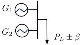
FIGURE 7 One-line diagram of a two-generator and one-load power system
