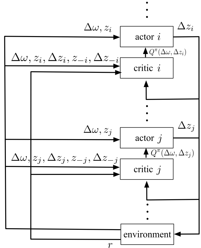
FIGURE 2 MADDPG schema in a frequency control scenario
