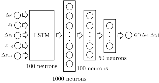
FIGURE 4 Architecture of the MADDPG critic
