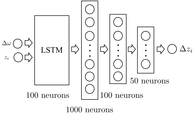
FIGURE 3 Architecture of the MADDPG actor
