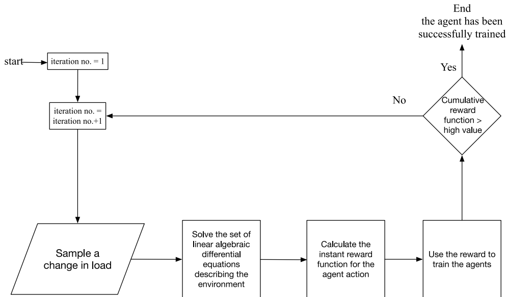
FIGURE 5 Diagram of the training process for developing the proposed load frequency control scheme
