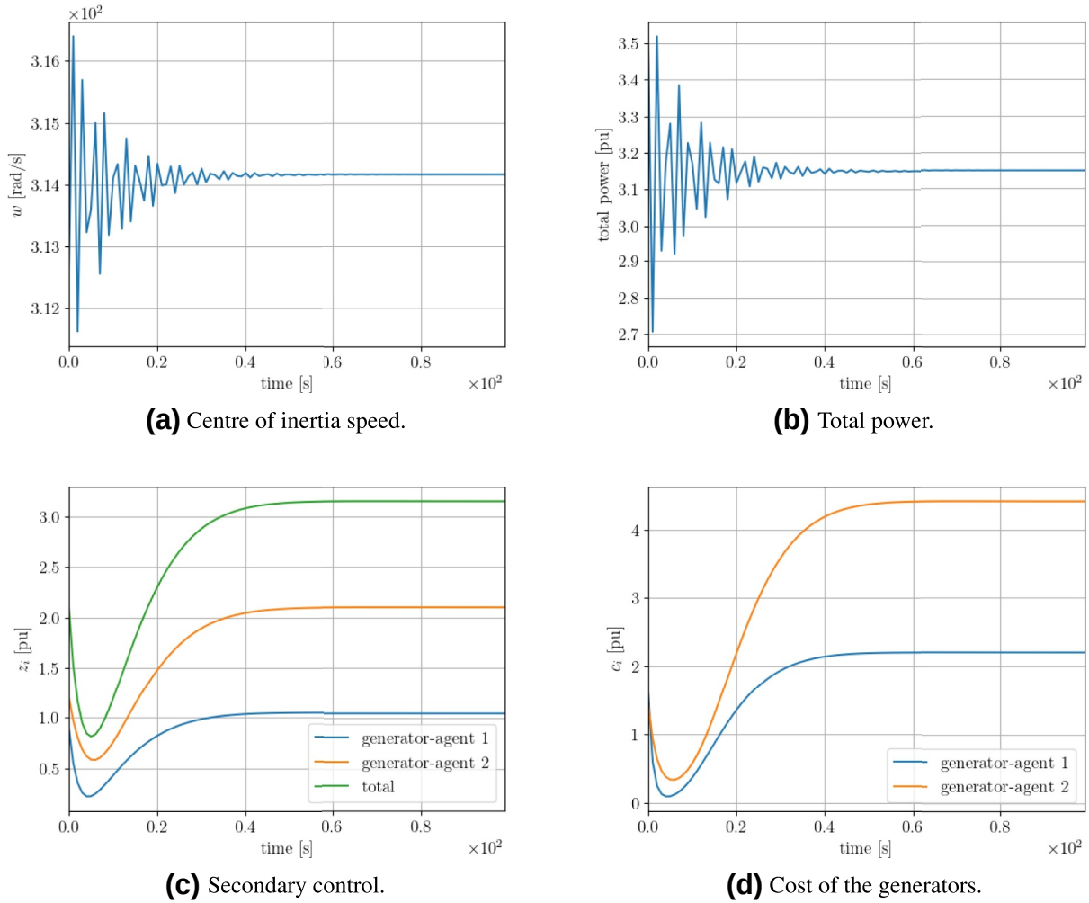
FIGURE 13 Change in load by 0.15 pu using the benchmark algorithm
