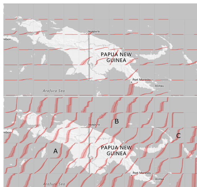
Figure 5: Local species accumulation curves, with a common y-axis (top) and a locally-scaled y-axis (bottom), indicating large differences in species richness.
