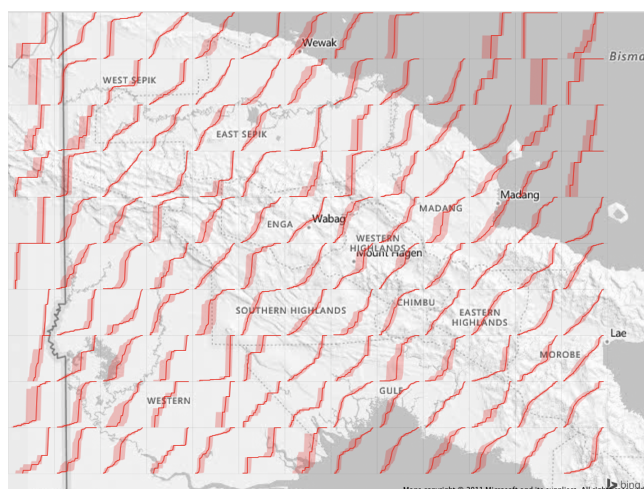
Figure 3: Design 2 is a regular array of spatially-local species accumulation curves indicating variation in species richness at different scales and across geographical space.
