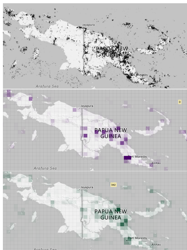
Figure 1: New Guinea: Top: Observations. Middle: Density of observations. Bottom: Density of species. There are more observations and more species diversity for Papua New Guinea (Eastern half) than Western New Guinea, but how does this relate to collection effort?
