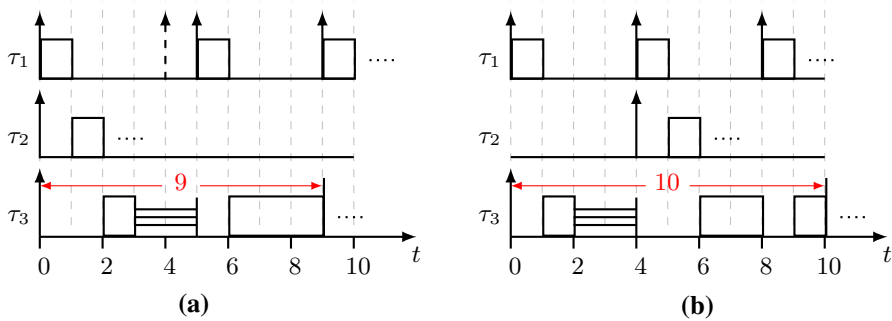
Fig. 5 A counterexample to demonstrate the misconception of the synchronous release of all tasks in Sect. 5.3 based on the task set in Table 9. a Release jobs synchronously. b Do not release jobs synchronously
