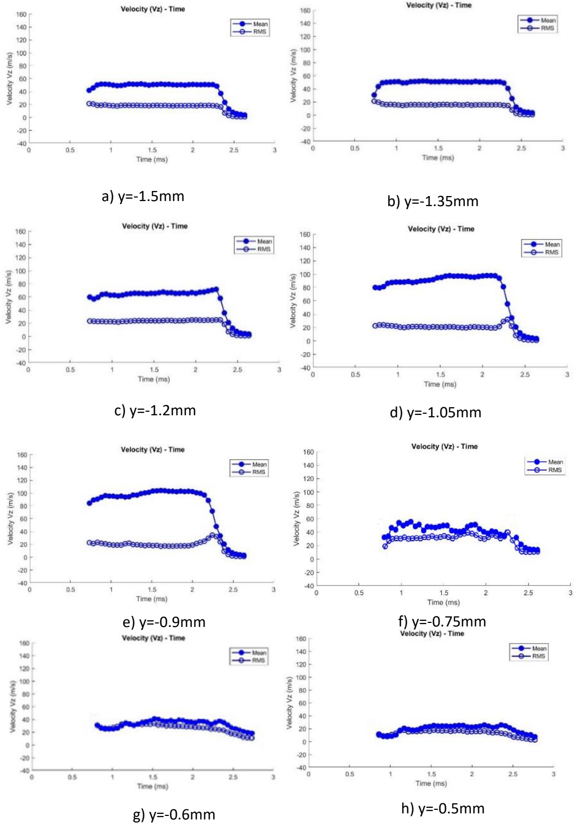
Figure 7-8 Temporal variation of average axial velocity over a time window of 0.05ms at z = 1\text{mm} , x=-0.2\text{mm} and at different y locations for 100 bar injection pressure and 2ms injection duration.
