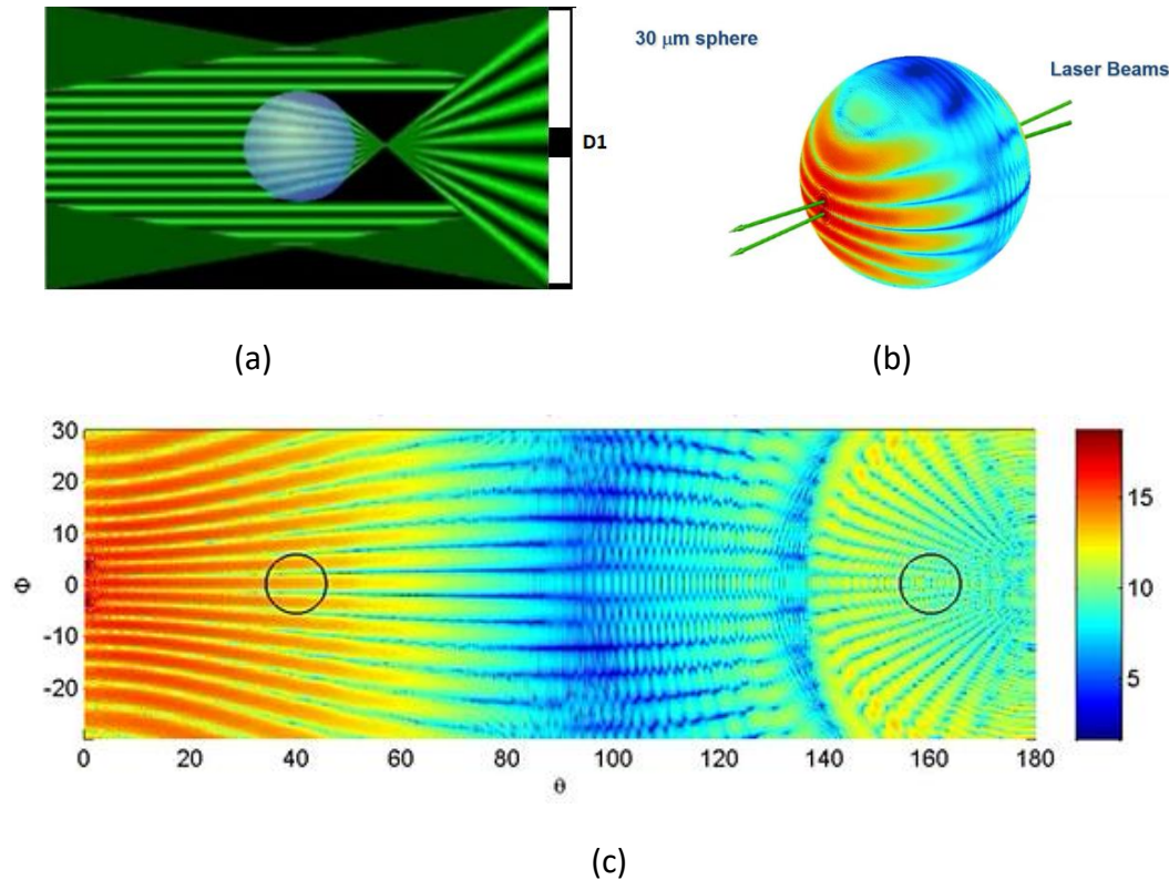
Figure 3-16 (a): A spherical droplet passing through the probing volume and the reflected light pattern from its surface on the receiver detector (LDA1 signal). (b): A 3D droplet with 30 \mu\text{m} diameter and the 3D light intensity contour plots shown on the surface of the droplet. (c) : The 2D contour plot of light intensity on the droplet surface with 100 \mu\text{m} diameter while moving through the probing volume [81]
