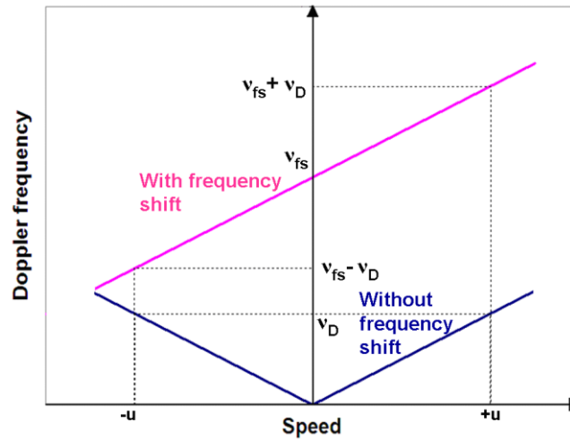
Figure 3-18 Schematic representation of frequency shift [82]
