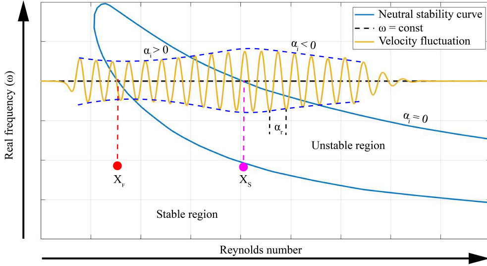
Figure 1.3: Stability curve for flow over flat plate with zero pressure gradient. Blue line - neutral stability curve, yellow line - velocity fluctuations, dotted blue line - envelope of velocity fluctuations.
