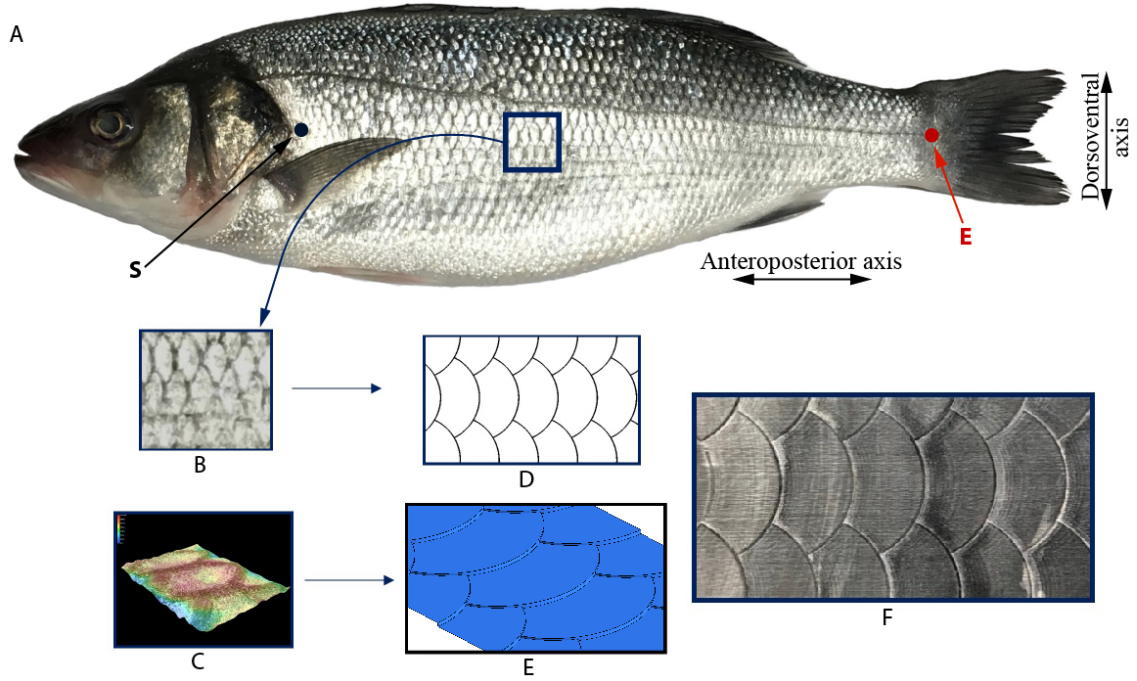
Figure 2.1: Microscope images and CAD replication of Sea bass fish scales (A) Picture of a Sea bass. Point S and E show the regions where measurements were taken. (B) Top view of the scales. (C) Topographical view from scanning with the Digital Microscope. (D) Top view of replicated CAD model. (E) Isometric view of CAD model (F) Photograph of 3-D printed model from top.
