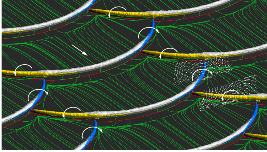
Figure 2.8: Surface streamline plot with direction of vortices. Vector plots at the overlap region for two consecutive scale rows. Helicity coloured in yellow for positive (Vortex direction CCW) and blue for negative (Vortex direction CW). Other rotational vectors are based on the colouring of vortices. Vortices are identified with 'Q' criterion. White straight arrow represents the mean flow direction.
