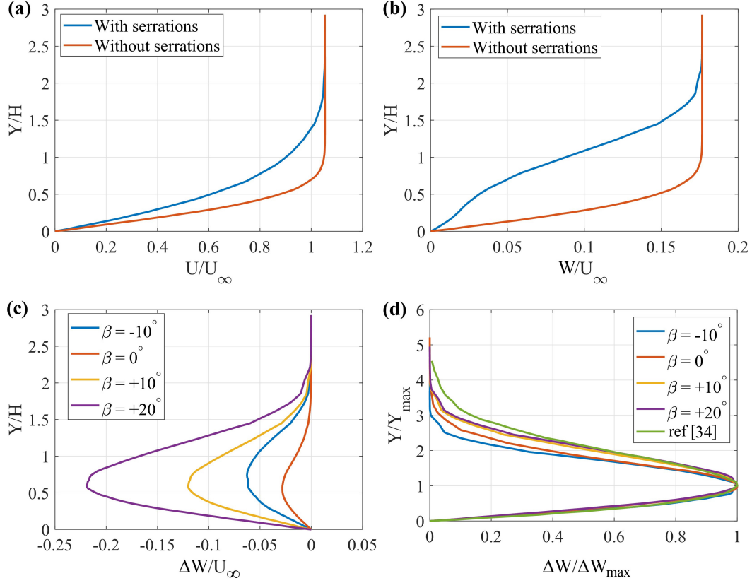
Figure 4.9: Velocity profiles from CFD simulations at X/L = 6 downstream of the leading edge. (a) Chordwise velocity for \beta = +10^\circ . (b) Spanwise velocity for \beta = +10^\circ . Net-effect of crossflow profile (c) For all sweep angles. (d) Normalised crossflow velocity profile with comparison to Ustinov and Ivanov (2018)
