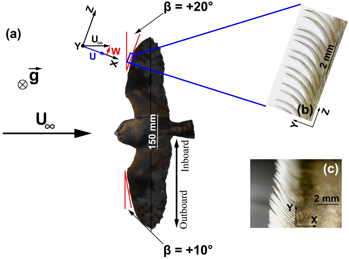
Figure 4.1: Gliding owl and leading edge serrations. a) Top view of an owl in gliding flight, illustrating the backward sweep of the wing. The situation is shown in a body-fixed observer situation with wind coming from left at a velocity ( U_\infty ). The wing portion at mid span has an effective positive sweep angle of \beta \approx 10^\circ , increasing to \beta \approx 20^\circ further towards 3/4 span. The picture of the owl is reproduced/adapted from the video published in (Durstion et al., 2019) with permission from Journal of Experimental Biology, reference (Durstion et al., 2019) with DOI: 10.1242/jeb.185488. Inset b) pointed picture of leading edge comb in back view with flow coming out of the paper plane; inset c) pointed picture of side view of the serrations with flow coming from left .
