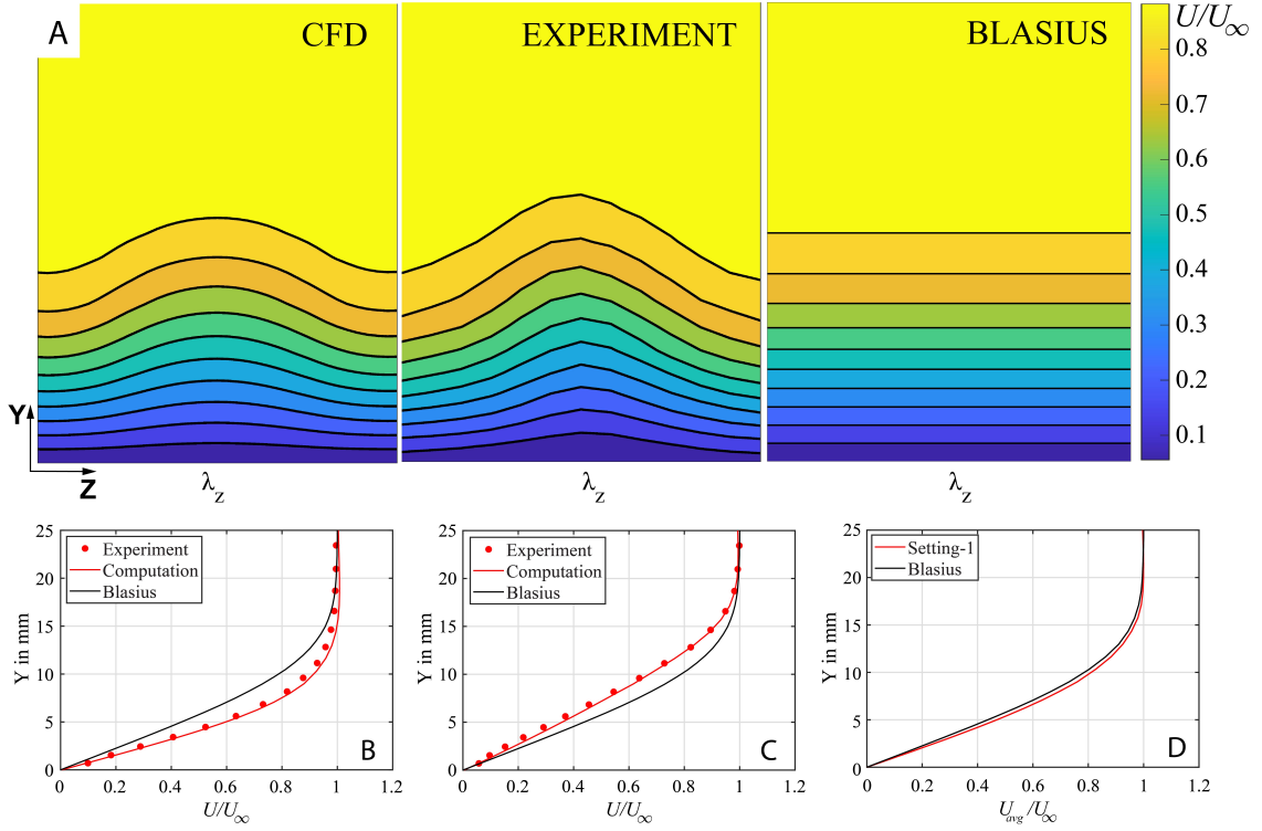
Figure 3.3: Comparison of CFD with experimental results (A) Velocity variation of streaky base flow in Z - Y plane at a distance of 1.2m from the leading edge (Left - CFD result, Middle - Hot-film result, Right - Blasius). Normalised velocity profile at (B) the overlap region (high-velocity region) behind the scale array Z = 0.025\text{m} . (C) at the central region (low-velocity region) behind the scale array Z = 0\text{m} . (D) Spanwise averaged streamwise velocity profile for Setting-1. Black line - Reference Blasius velocity profile
