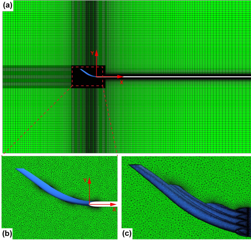
Figure 4.12: Computational domain with serrations. (a) Unstructured mesh near serrations (shown inside red rectangle) and structured mesh in all other regions. (b) and (c) Enlarged view around the serrations.
