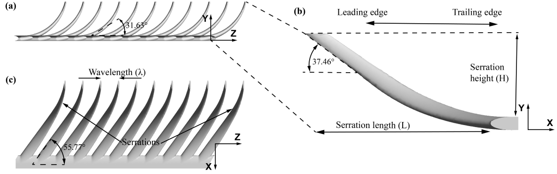
Figure 4.2: Orientation of the reconstructed serrated leading edge. a) back-view of the comb, looking from the back over the feather onto the outstanding barbs of the right wing, compare also Fig. 1b. b) Side view on a single barb in enlarged scale showing the tilt angle ( 37.5^\circ ) c) top-view of the comb in the feather plane, showing the inclination angle ( 55.8^\circ ) of serrations along the spanwise direction.
