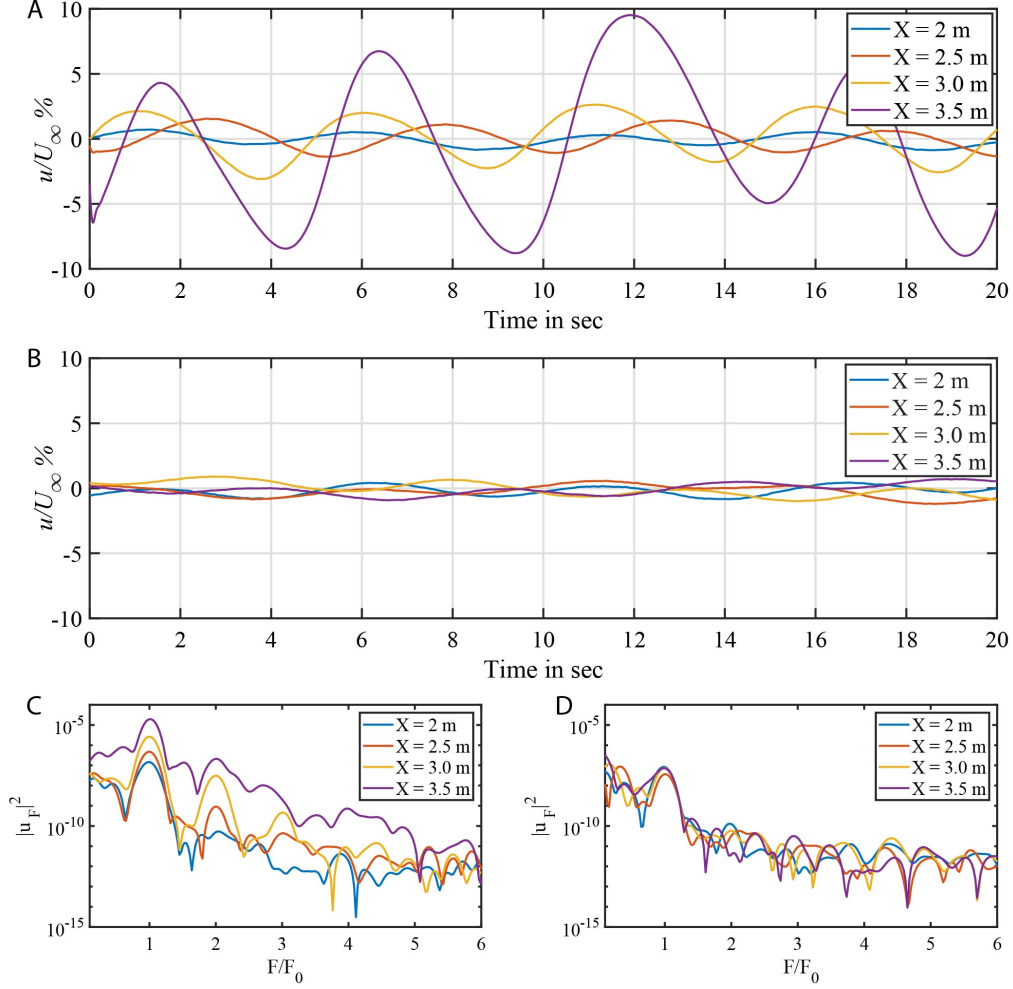
Figure 3.5: Instantaneous velocity and spectrum for reference flat plate and fish scale array case (A) Instantaneous velocity at four locations for reference flat plate case. (B) Instantaneous velocity at four locations for fish scale array case (Setting-1). (C) Spectrum for the velocity signals for reference flat plate case. (D) Spectrum for the velocity signals for fish scale array case (Setting-1).
