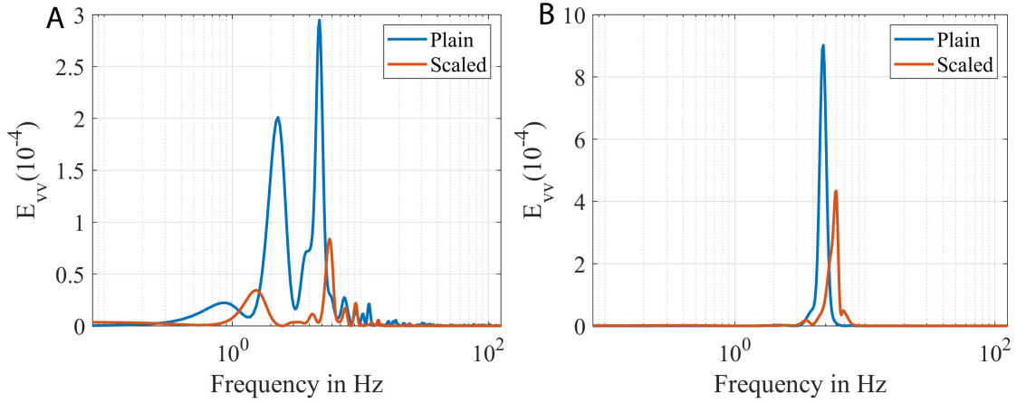
Figure 3.18: Power spectrum for plain and scaled hydrofoil at U_\infty = 30\text{cm/s} (A) spectrum from cross velocity behind trailing edge of hydrofoil. (B) spectrum for POD mode-1.
