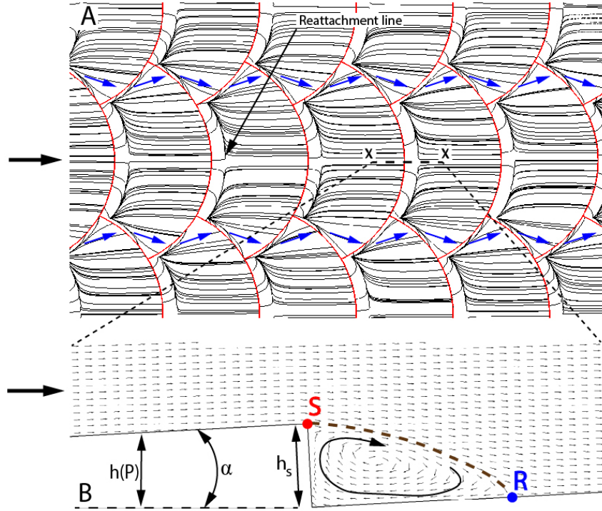
Figure 2.7: Surface streamline and vector plots from CFD simulation. (A) Top view of surface streamline over the scales. Note the zig-zag motion along the overlap region compared to the parallel flow at the central regions of the scales. (B) Vector field in the x-z cross sectional plane along the central region of the scale at line X-X (vectors indicate only direction and not magnitude). h_s = 1mm and \alpha = 3 degrees. S and R represents the separation and reattachment of the flow streamlines. Thick dashed line indicates the region of recirculating flow with an arrow indicating the direction of rotation. In both drawings the black arrow indicates the mean flow direction.
