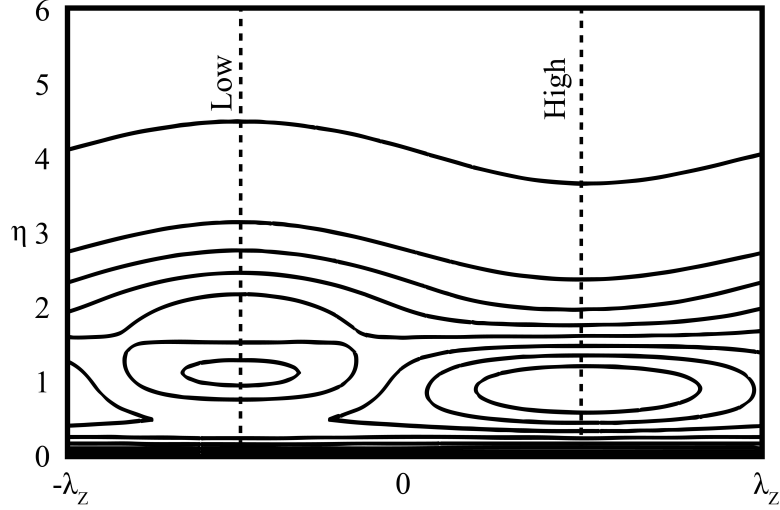
Figure 3.11: Contours of constant velocity fluctuation amplitude (streamwise component) in a cross-section at X = 2.5\text{m} for Setting-2 at f = 0.2\text{ Hz} .
