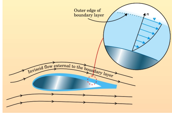
Figure 1.1: Viscous flow over an airfoil. The blue coloured border depicts the thin boundary layer region. Inset shows the velocity profile inside the boundary layer. Source: Prandtl's boundary layer by John D. Anderson (Anderson, 2005).
