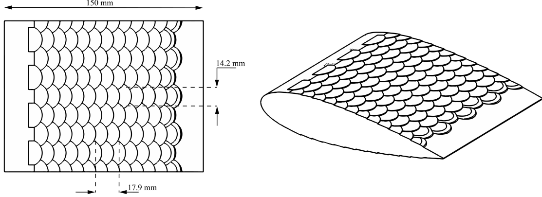
Figure 3.14: CAD drawing of hydrofoil
