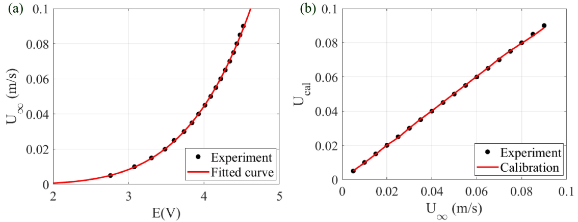
Figure 4.19: Hot-film calibration curves. (a) Voltage vs velocity. (b) Experimental velocity vs calibrated velocity from the hot-film probe.
