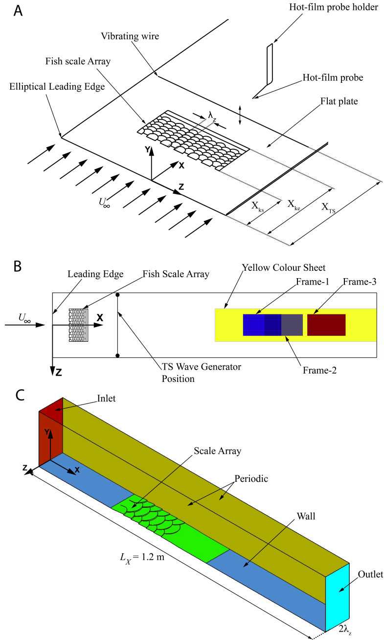
Figure 3.2: Experimental flow set-up, details of flow visualisation set-up and computational domain (A) Experimental Set-up in the Laminar Water channel with a biomimetic scale array. (B) Experimental arrangement from top view, Yellow area is the region in which a yellow sheet was glued on the flat plate. All three frames where videos were recorded are shown by rectangles. Note that Frame-1 and Frame-2 have some overlap. (C) CFD domain with periodic conditions. Setting-1 is shown in this figure and for Setting-2 all conditions remain the same except the fish scale array geometry. The inlet was provided with velocity parallel to X-axis with a value of U_\infty = 0.086\text{m/sec} .
