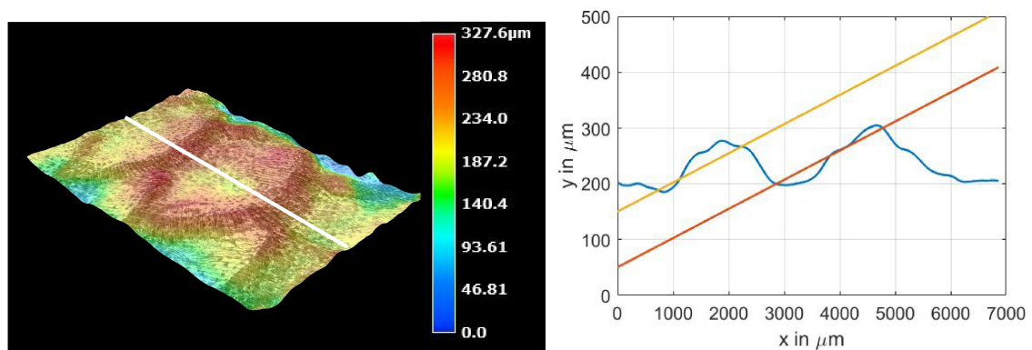
Figure 2.11: 3D topography obtained with a digital microscope. White colour line - Profile variation was measured (left). Profile height along the centreline of the fish scale. The lines indicate the average tilt of scales from the horizontal axis (Approximately 3 degrees) (right).
