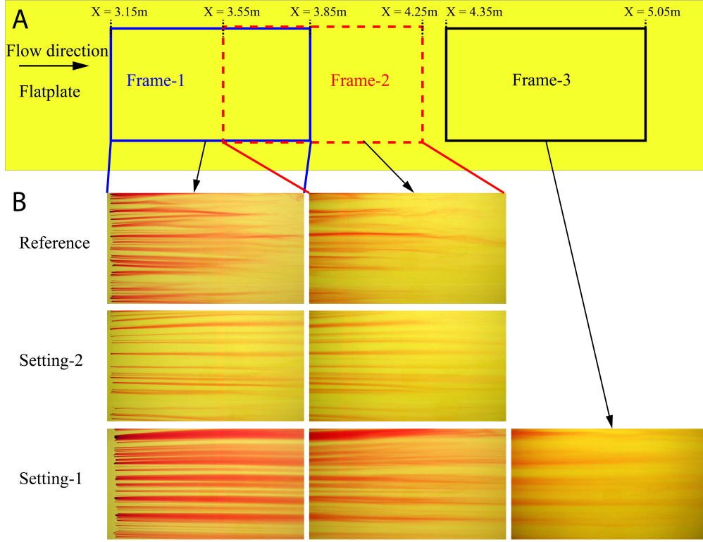
Figure 3.6: Flow visualisation results (A) Flow visualisation setting, Frame-1: 3.15 to 3.85m (Blue rectangle), Frame-2: 3.55 to 4.25m (Dotted red rectangle), Frame-3: 4.35 to 5.05m (Black rectangle). Blue line pair mark Frame-1 and Red line pair mark Frame-2 regions. (B) Flow visualisation pictures for reference, Setting-2 and Setting-1 cases.
