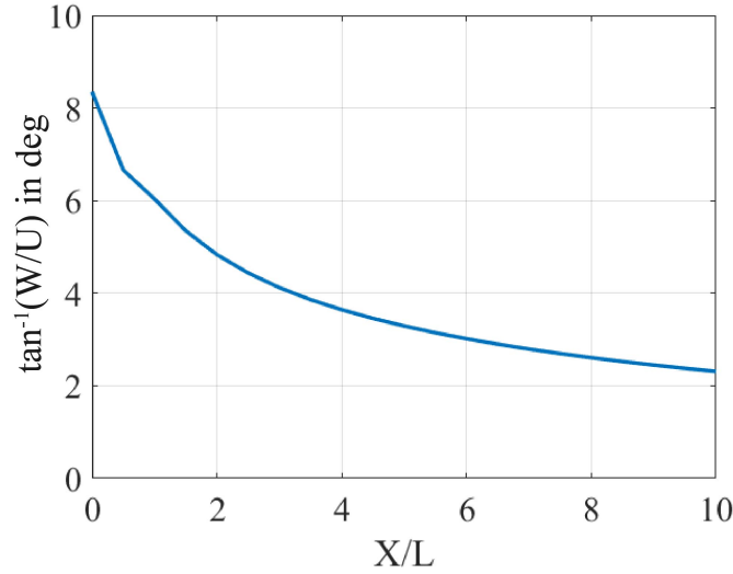
Figure 4.15: Maximum flow turning angle specified in degrees over downstream distance normalised by the serration length (L).
