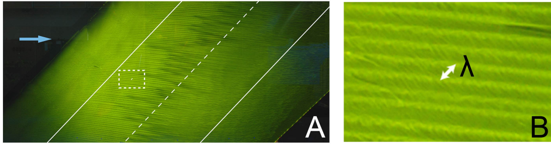
Figure 1.6: Flow visualisation picture over a 45 deg swept wing. (A) Cross-flow vortices on a NACA 66018 aerofoil at Re = 2.15 \cdot 10^6 (flow is from left to right). (B) Enlarged picture from frame 'A' which shows the wavelength ( \lambda ) of the crossflow vortices. From Serpieri (Serpieri and Kotsonis, 2015).
