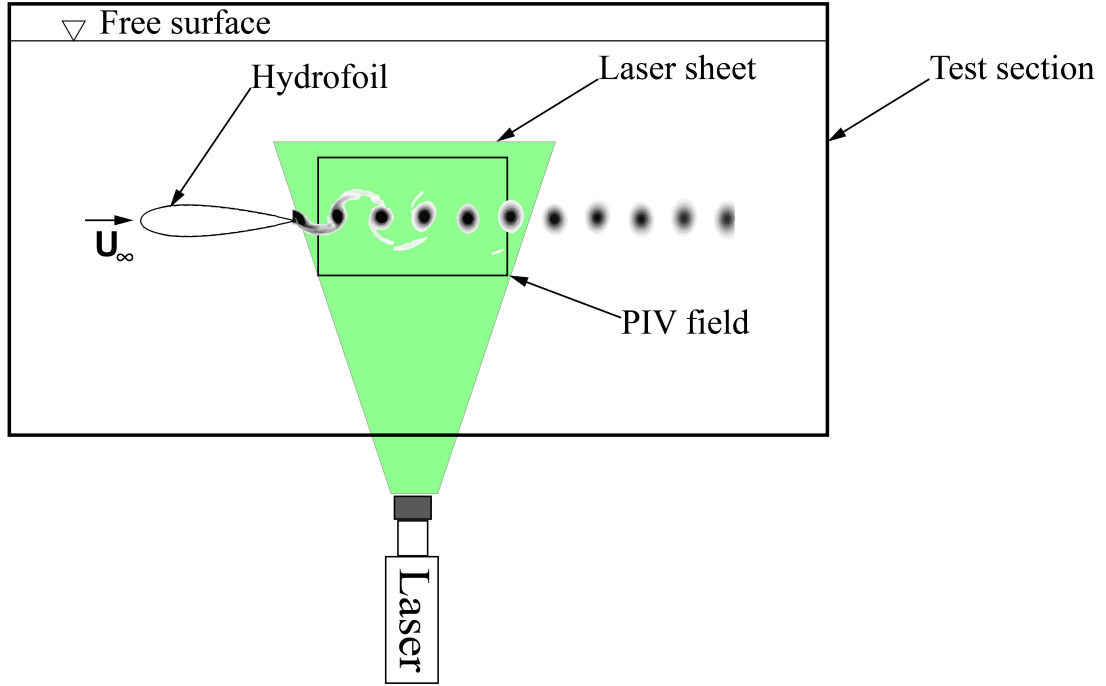
Figure 3.15: Schematic diagram of the experimental set-up. Circular End plates were used to avoid spanwise leakage flows (not shown here).
