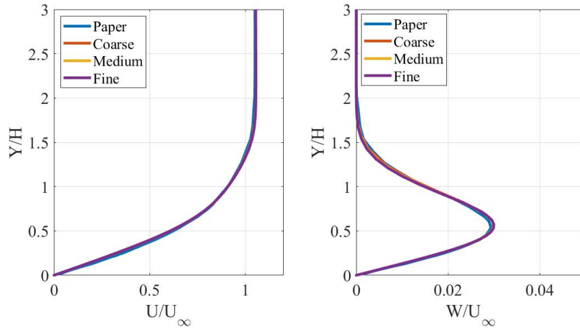
Figure 4.13: Mesh dependency result for all grids. Normalised velocity profiles behind five times the serration length. Streamwise velocity ( U/U_\infty ) (Left) and Crosswise velocity ( W/U_\infty ) (Right).
