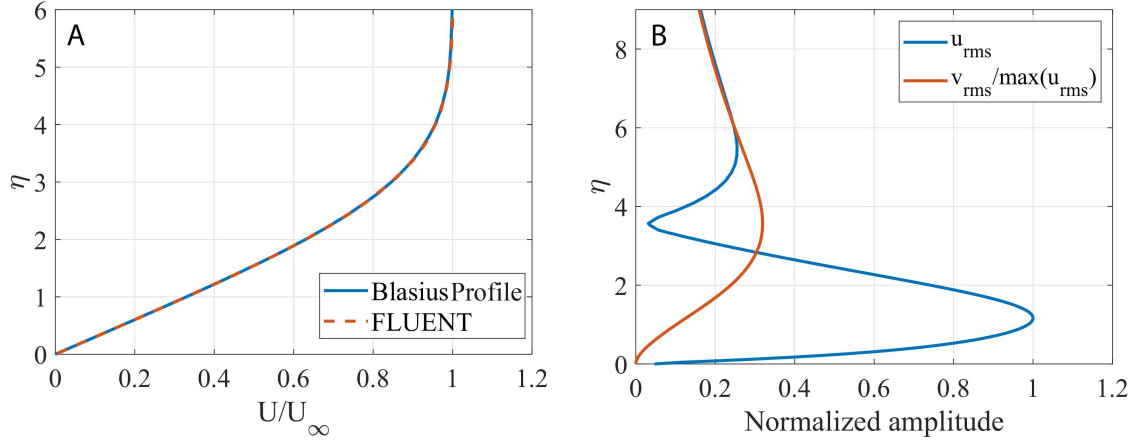
Figure 3.9: Boundary layer and fluctuation profiles at X = 1.2\text{m} : (A) Comparison streamwise velocity profile from computation with Blasius profile. (B) Streamwise and wall normal fluctuation velocity profiles for f = 0.2\text{ Hz} .
