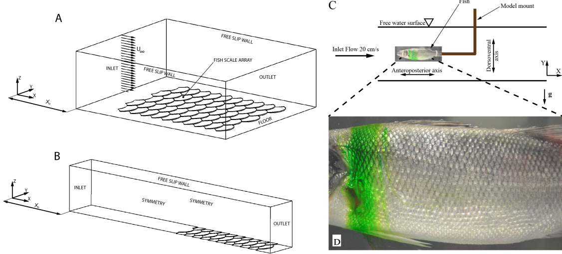
Figure 2.2: Computational domain and Experimental set-up (A) Configuration of the fish-scale array in CFD similar to the condition of the physical model of the scale array at the bottom wall of the wind tunnel. Note that the velocity vector represents the inlet profile with free-stream velocity parallel to the 'x' axis in positive direction (Anteroposterior direction). 'y' axis represents the spanwise (Dorsoventral direction) and 'z' axis represents wall normal direction. (B) CFD domain with symmetry conditions to simulate the drag variation with no end effects. In both the figures ' x_o ' is the imaginary length from the leading edge of the plate to the inlet of the domain. (C) Schematic diagram of the experimental set-up. (D) Dye coating on the surface of the fish.
