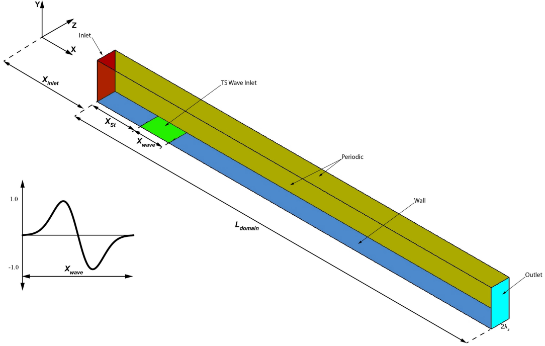
Figure 3.8: Domain for TS-wave CFD simulation Inlet to the domain is X_{inlet} = 0.8m from the leading of the flat plate. L_{domain} = 4.2m which starts from 0.8m and ends at 5m in X-direction. The typical profile of the TS-wave velocity is shown on the left.
