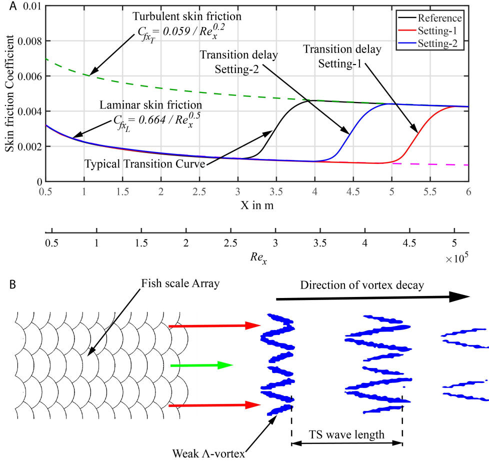
Figure 3.7: Typical skin friction plot and proposed flow manipulation mechanism (A) Skin friction coefficient curve: Dashed green line - Turbulent flow, Dashed pink line - laminar flow. (B) Flow behind fish scale array with modulated TS wave. Red arrow - High-velocity region, Green arrow - Low-velocity region.
