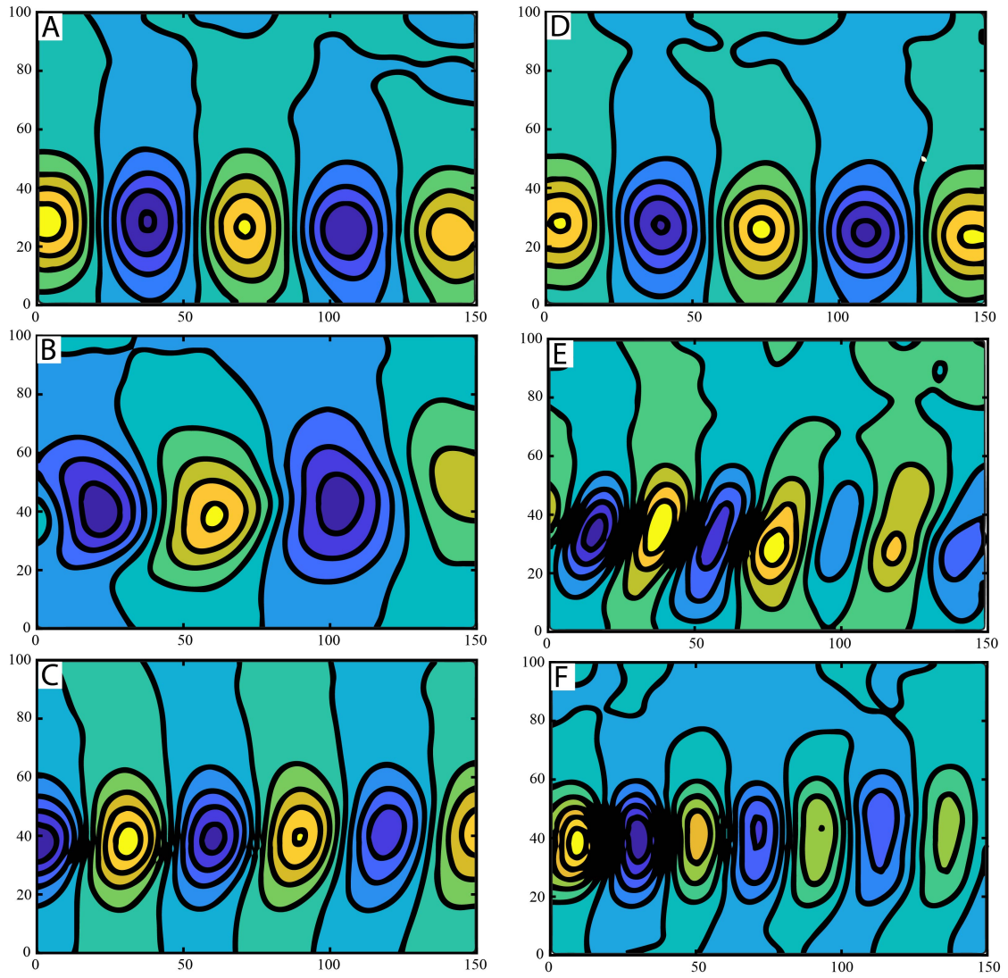
Figure 3.17: Mode-1 from cross velocity. Plain hydrofoil (A) 10 cm/s (B) 20 cm/s (C) 30 cm/s, Scaled hydrofoil (D) 10 cm/s (E) 20 cm/s (F) 30 cm/s.
