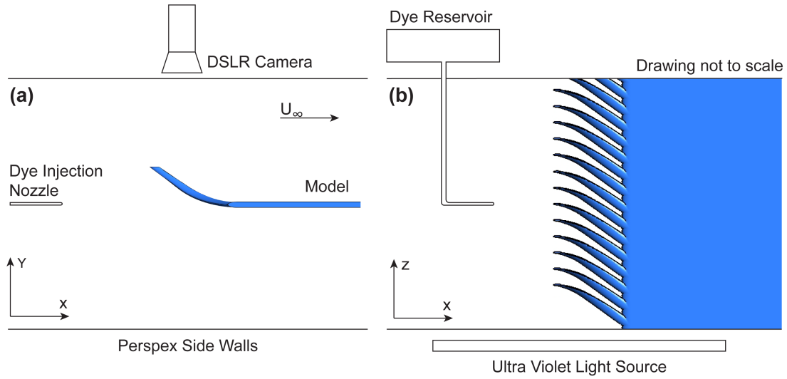
Figure 4.5: Sketches of the experimental set-up for the dye flow visualizations carried out in the CHB Water Tunnel at City, University of London. (a) plan view of the set-up in the horizontal cross-section. (b) Side view on the vertically mounted flat plate.
