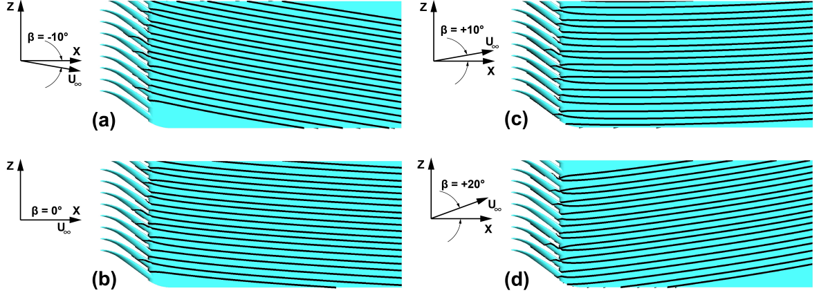
Figure 4.7: Surface streamlines from CFD simulations. (a) Negative sweep angle \beta = -10^\circ . (b) Zero Sweep angle \beta = 0^\circ . Positive sweep angle (c) \beta = +10^\circ . (d) \beta = +20^\circ
