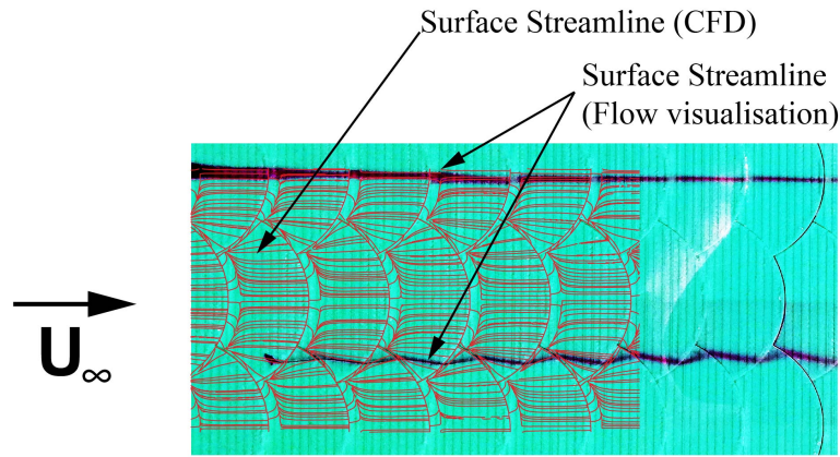
Figure 2.14: Surface flow visualisation pictures overlaid with CFD result.
