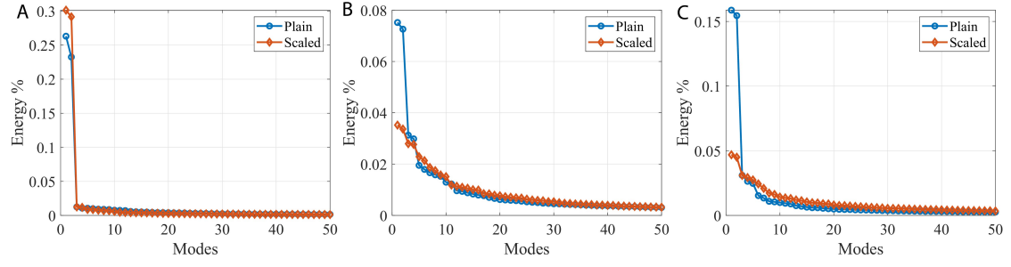
Figure 3.16: Comparison of Energy for plain and scaled hydrofoil. (A) 10 cm/s (B) 20 cm/s (C) 30 cm/s.
