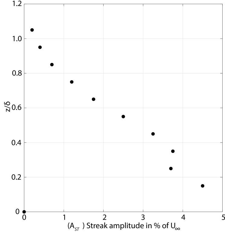
Figure 2.4: Variation of streak amplitude along wall-normal direction for model fish scales. Measurements were made 190 mm from water inlet (along black line shown in Fig. 2.3b)
