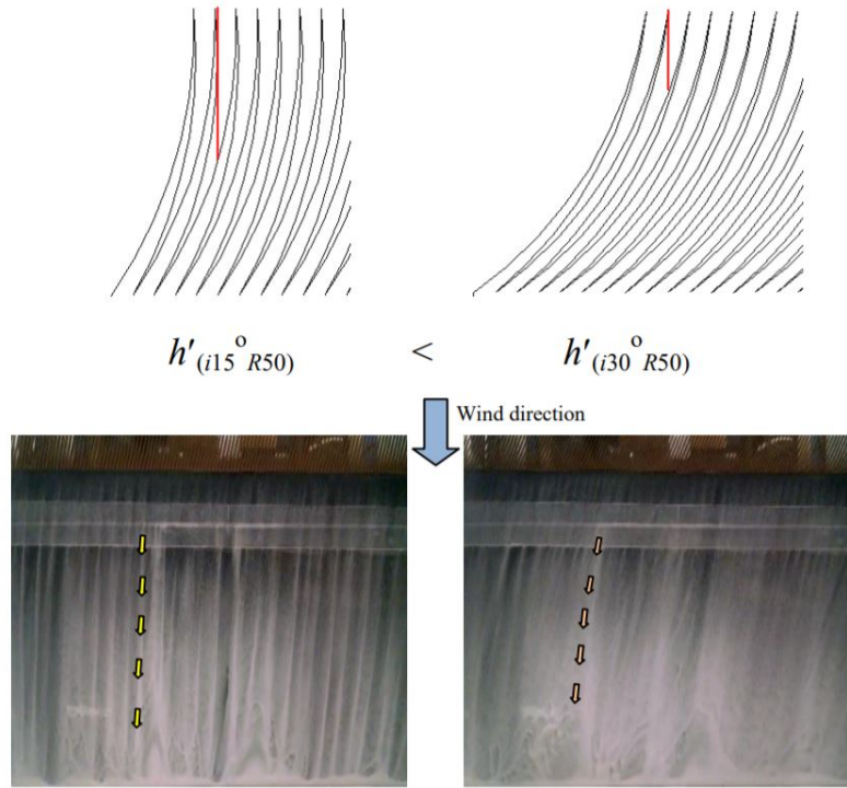
Figure 4.17: Flow deflection picture behind 2D curved serrations. Reproduced from (Juknevičius et al., 2017).
