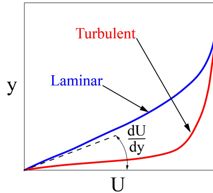
Figure 1.2: Boundary layer velocity profile. Blue curve - laminar, Red curve-turbulent and dashed line represents velocity gradient \frac{dU}{dy} at wall.
