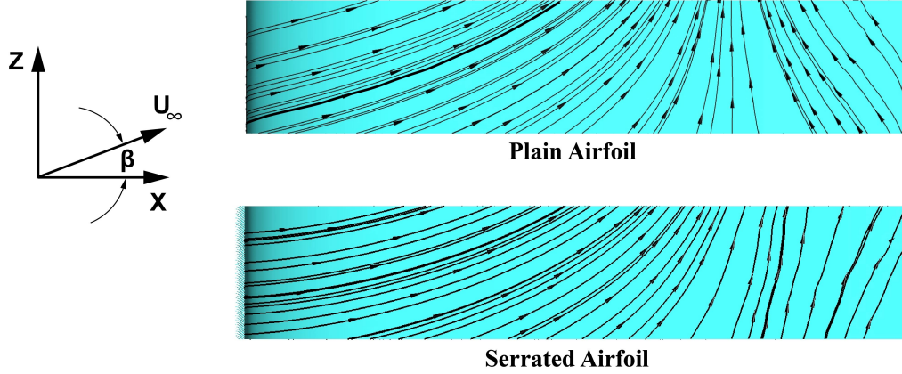
Figure 4.10: Time averaged surface streamline for Plain airfoil (top), Serrated airfoil (bottom).
