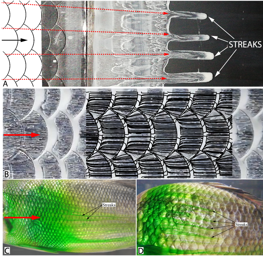
Figure 2.5: Surface flow visualisation on the scales. (A) Black arrow represents mean flow direction. Note that the oil-mixture was painted in the region downstream of the scales to highlight the generation of the streaks. 2-D top view of the CAD model is merged to get the impression of the arrangement of the scales. The red arrows were added to illustrate the trace of the streaks relative to the arrangement of the scales. (B) Red arrow represents the mean flow direction. Herein, the oil-mixture was painted directly onto the scales. Surface streamlines from CFD simulation are overlaid to compare the results. Note that the regions of accumulated oil-patches match with the regions of flow reversals from CFD simulation. (C and D) Oil-flow visualisation on sea bass ( Dicentrarchus labrax ) and common carp ( Cyprinus carpio ).
