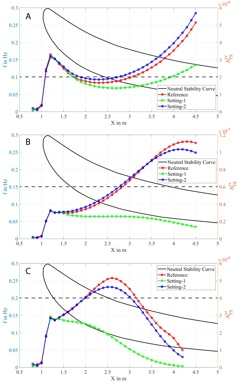
Figure 3.13: Integral streamwise fluctuation profiles for different cases. Red curve - Reference Blasius case, Green curve - Setting-1, Blue curve - Setting-2, (A) f = 0.1 Hz. (B) f = 0.15 Hz. (C) f = 0.2 Hz
