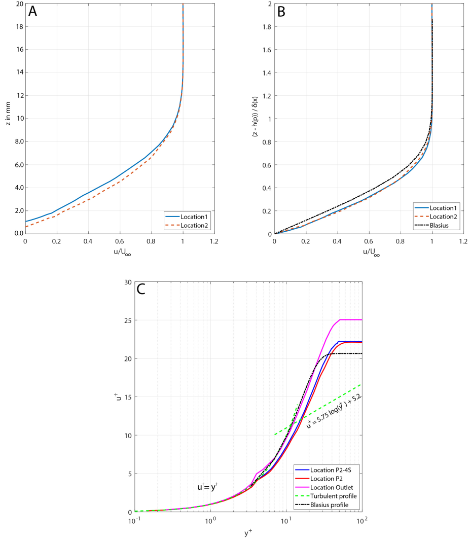
Figure 2.6: Boundary layer profiles at Location 1 and Location 2 (probe points P1 and P2 in Fig. 2.3B). (A) Normalised velocity profiles in the absolute coordinate system. Note that the shift in velocity profiles along 'z' direction is because of the change in scale height h(P) for the different probe points P (B) Normalised velocity in the body coordinate system with Blasius laminar boundary layer profile along a smooth flat plate. (C) Dimensionless velocity profile at three locations: Location P2, four scales upstream from Location P2 (P2-4S) and at outlet.
