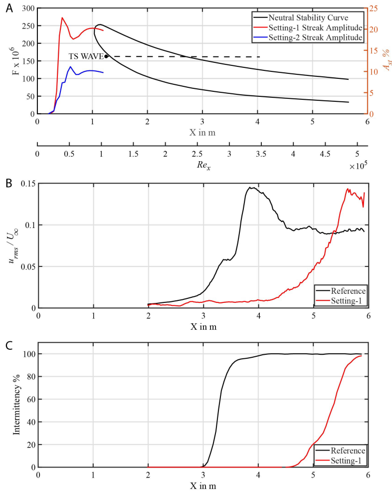
Figure 3.4: Neutral stability curve, root mean square of velocity fluctuations and intermittency variation (A) Neutral stability curve and streak amplitude for two settings. (Normalised frequency F given in left 'y' coordinate and streak amplitude A_{st} given in right 'y' coordinate, Black dot marks the TS wave generator position and dotted line indicates the frequency value). (B) u_{rms} plot normalised by free stream velocity ( U_\infty ) for reference flat plate and Setting-1. (C) Intermittency plot for reference flat plate and Setting-1
