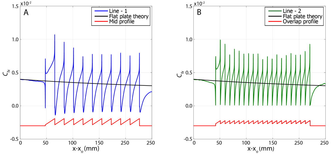
Figure 2.9: Variation of skin friction coefficient ( C_{fx} ) along 'x' direction at two locations. (A) Blue line represents the C_{fx} variation along (Line-1) (refer Blue line in Fig. 2.3B) (B) Green line represents the C_{fx} variation along (Line-2) (refer Green line in Fig. 2.3B). Red lines represents variation of 'z' coordinate in 'x' direction along corresponding locations (not to scale). Black line represents the variation of C_{fx theory} for flat plate boundary layer by Eqn.2.5. x_o (333mm) is the imaginary length before the inlet of the domain.
