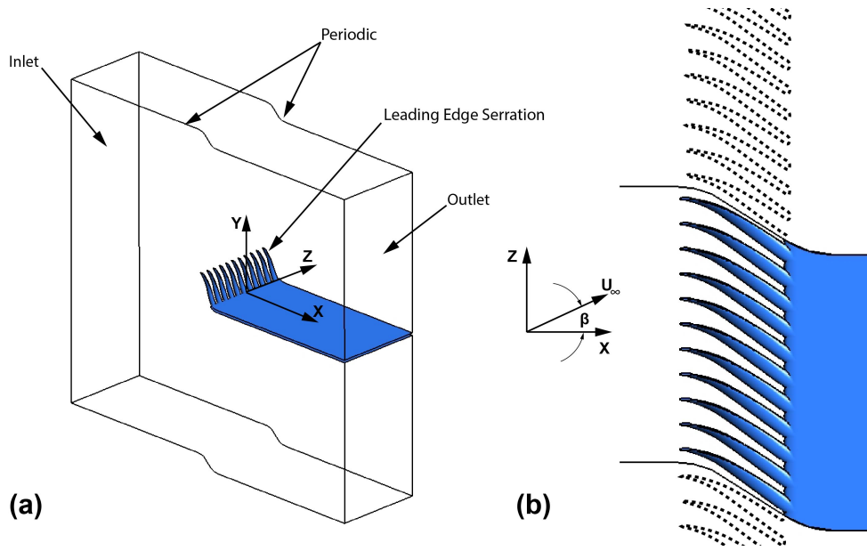
Figure 4.4: Sketches of the CFD domain and the flow configuration with respect to the comb. (a) Isometric view of the CFD domain with periodic conditions in Z-direction. Leading edge serrations attached with the flat plate is shown in blue colour surface (b) Enlarged view of leading edge serration in the X-Z plane showing the direction of the inlet flow velocity vector ( U_{\infty} ) at an angle ( \beta ) (sweep angle) with X-axis. (Hidden lines of the serration are indicating the periodic boundary condition)
