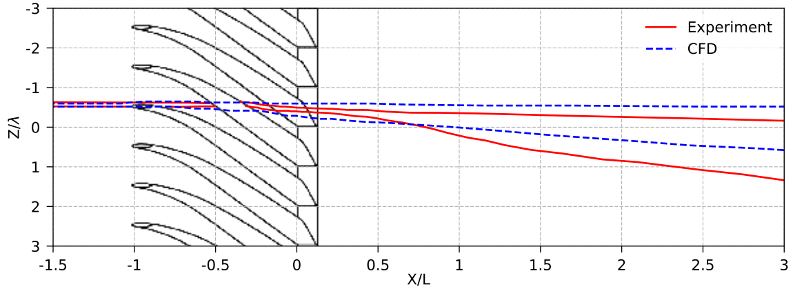
(c) Range of the most-extreme turning streamline relative to the streamline at the tip. From the CFD simulation and the dye trace from the water tunnel experiment
