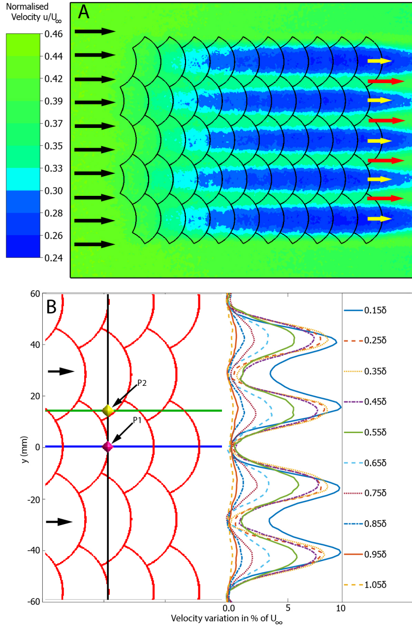
Figure 2.3: Velocity contour and velocity profiles (A) Normalised Velocity Contour at a wall-parallel plane at a distance of z = 0.25\delta from the surface. Arrows indicate flow direction. Note that the black arrows at the inlet are uniform in length, while red and yellow arrows at the outlet differ in length. (B) Velocity variation in spanwise direction at various wall-normal distances in the boundary layer. Scale array is shown in red color for better illustration. Blue line (Line-1) represents a centreline of a row of scales. Green line (Line-2) represents the overlap region between the scales. Black line represents a location in the 'x' direction at 190mm from inlet. Location1 (P1) and Location2 (P2) are probe points at 190mm from inlet on centreline region and overlap region. Black arrow indicates mean flow direction
