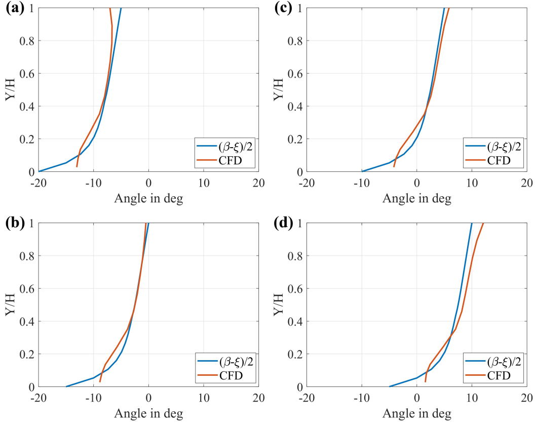
Figure 4.8: Wall-normal variation of turning angle behind serrations at X/L=0 for different sweep angles from CFD results and analytical formula. (a) \beta = -10^\circ . (b) \beta = 0^\circ . (c) \beta = 10^\circ . (d) \beta = 20^\circ .
