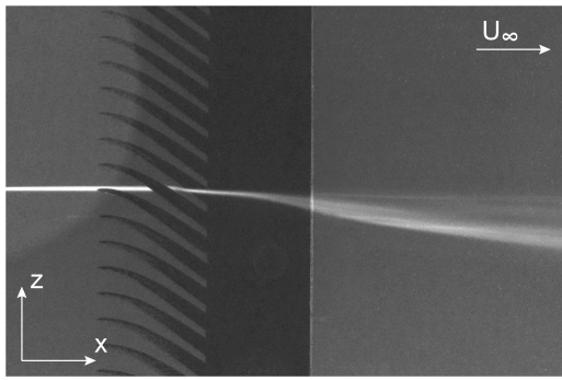
(a) Long-time exposure image of the dye flow visualisation, illuminated under ultra violet light (image has been contrast-enhanced for better clarity).
