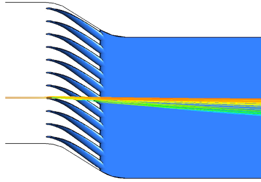
(b) Top view on streamlines with different starting points along the wall-normal axis in color (green: near-wall to red: tip of the serrations, CFD simulation at \beta = 0^\circ ).
