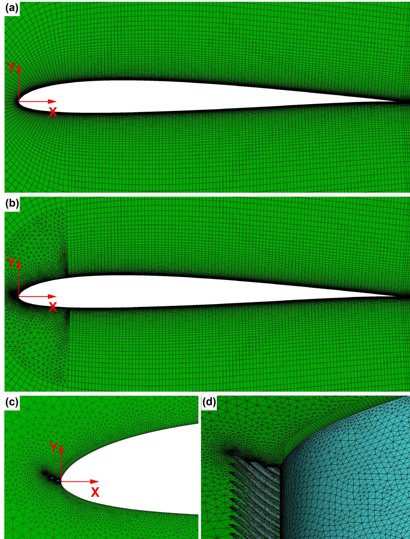
Figure 4.14: Mesh for plain airfoil with and without serrations. (a) Structured mesh around plain airfoil. (b) Mesh for airfoil with serrations (c) and (d) Enlarged view around the airfoil with serrations.
