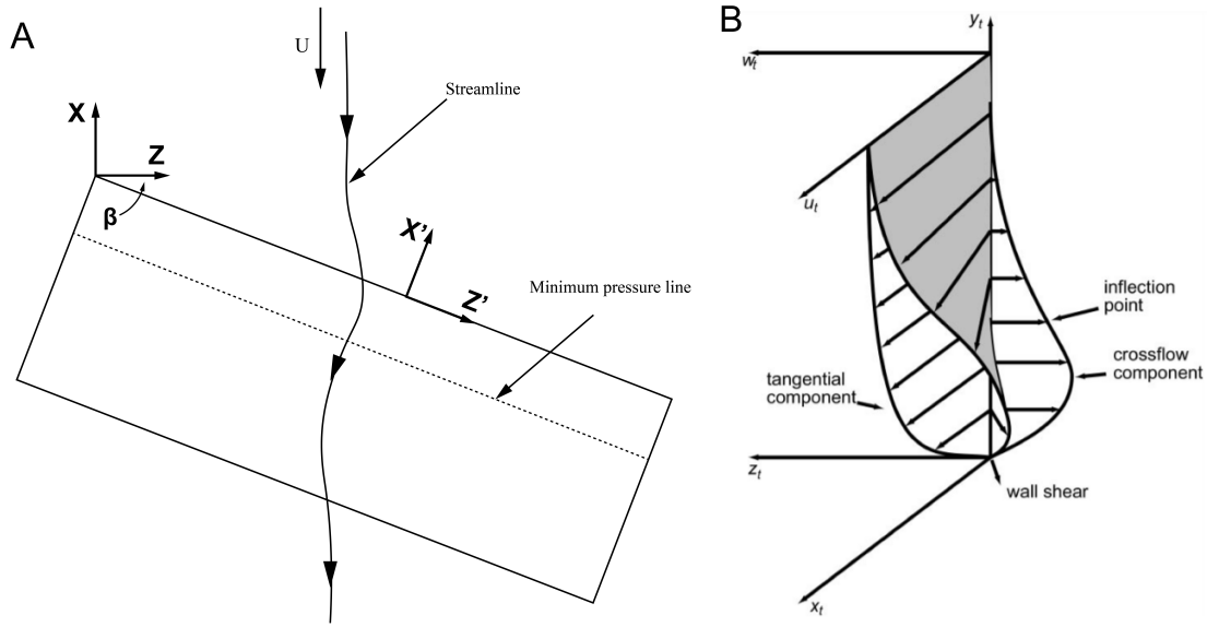
Figure 1.5: Flow over swept wing and velocity profiles. (A) Streamlines viewed from top view. Adapted from Houghton (Houghton et al., 2017). (B) Tangential and crossflow velocity profiles on a swept wing. From Saric (Saric et al., 2003).
