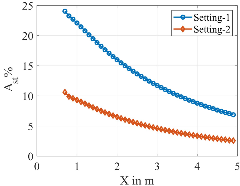
Figure 3.10: Variation of streak amplitude A_{st}\% behind the scale arrays for Setting-1 and Setting-2 from X = 0.7\text{m} to X = 5.0\text{m} .
