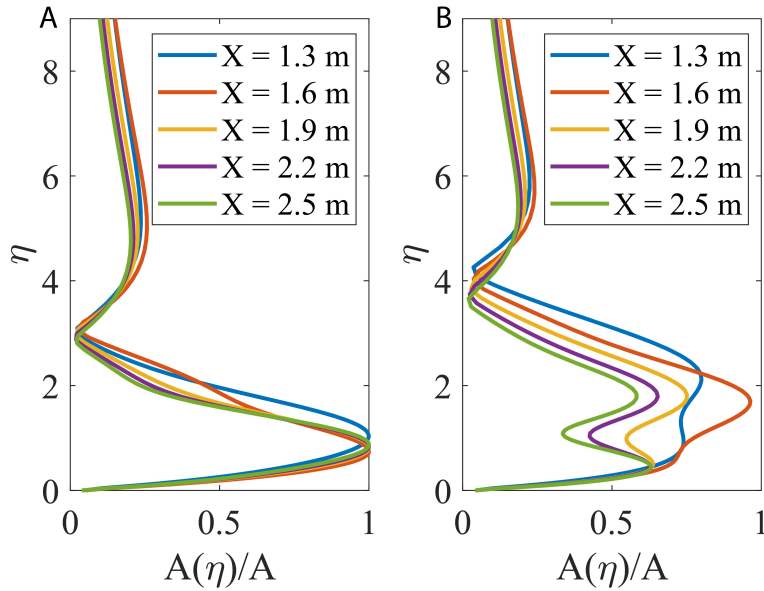
Figure 3.12: Profiles of Velocity fluctuation (streamwise component) at different locations ( X = 1.3, 1.6, 1.9, 2.2 and 2.5\text{m} ) for Setting-2 at f = 0.2\text{ Hz} . (A) y -position in the center of High-speed streak. (B) y -position in the center of Low-speed streak.
