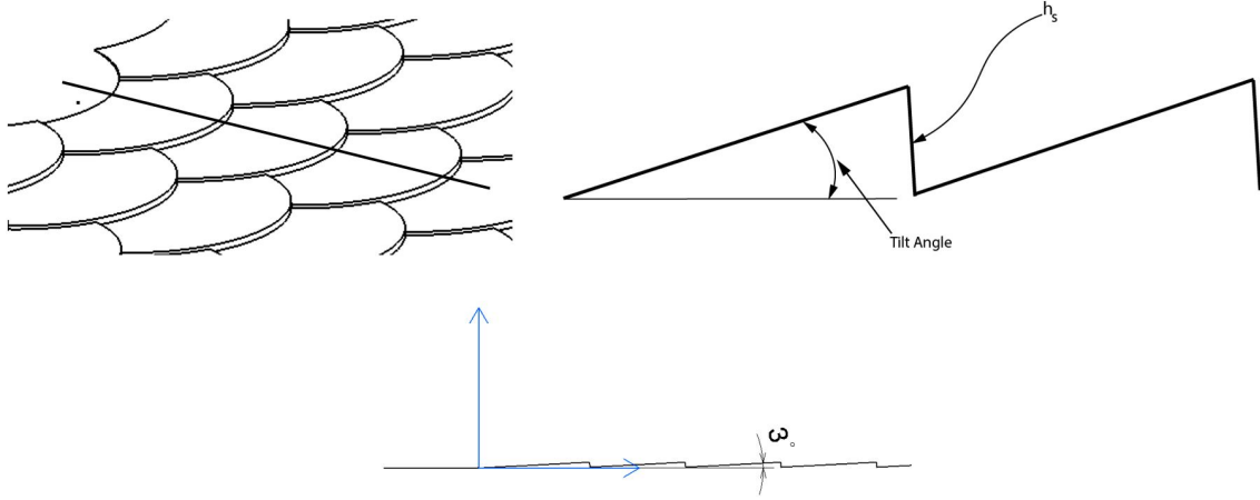
Figure 2.12: 3D view from CAD model (Left). Tilt angle of scale from horizontal axis and scale height h_s (Not to scale)(Right). Actual tilt angle of the scale (3 degrees) shown in bottom.
