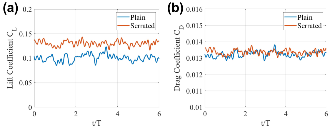
Figure 4.16: Aerodynamic characteristics of plain and serrated aerofoil. (a) Lift Coefficient. (b) Drag Coefficient.
