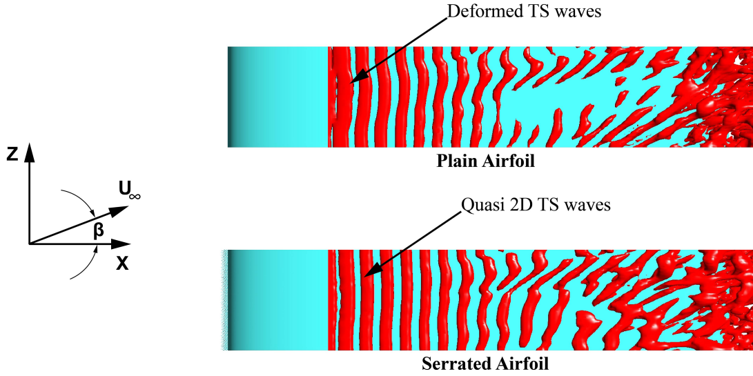
Figure 4.11: Instantaneous vortices identified with ‘Q’ criterion. Plain airfoil (top), Serrated airfoil (bottom).
