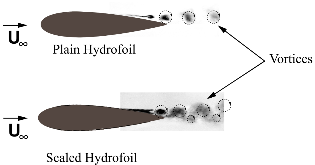
Figure 3.19: Flow visualisation results for Plain hydrofoil (top) and Scaled hydrofoil (bottom) at U_\infty = 30\text{cm/s} .
