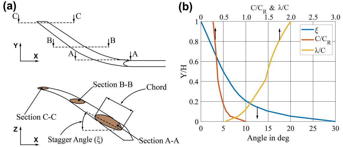
Figure 4.3: Serration drawings and plots a) Single barb with three sections showing the cross-section twist, where section A-A is the cross-section near to the root of the barb, section B-B is the cross-section at the mid-point of the barb and section C-C is the cross-section at the tip of the barb. b) Stagger angle ( \xi ), Normalised chord ( C/C_{Root} ) and spacing to chord ratio ( \lambda/C ) with normalised height of serration
