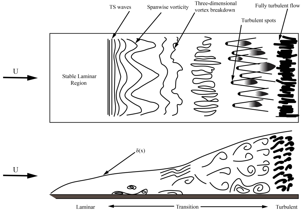
Figure 1.4: Transition to turbulence from Tollmien-Schlichting wave instability. Reproduced from White (White, 2006).
