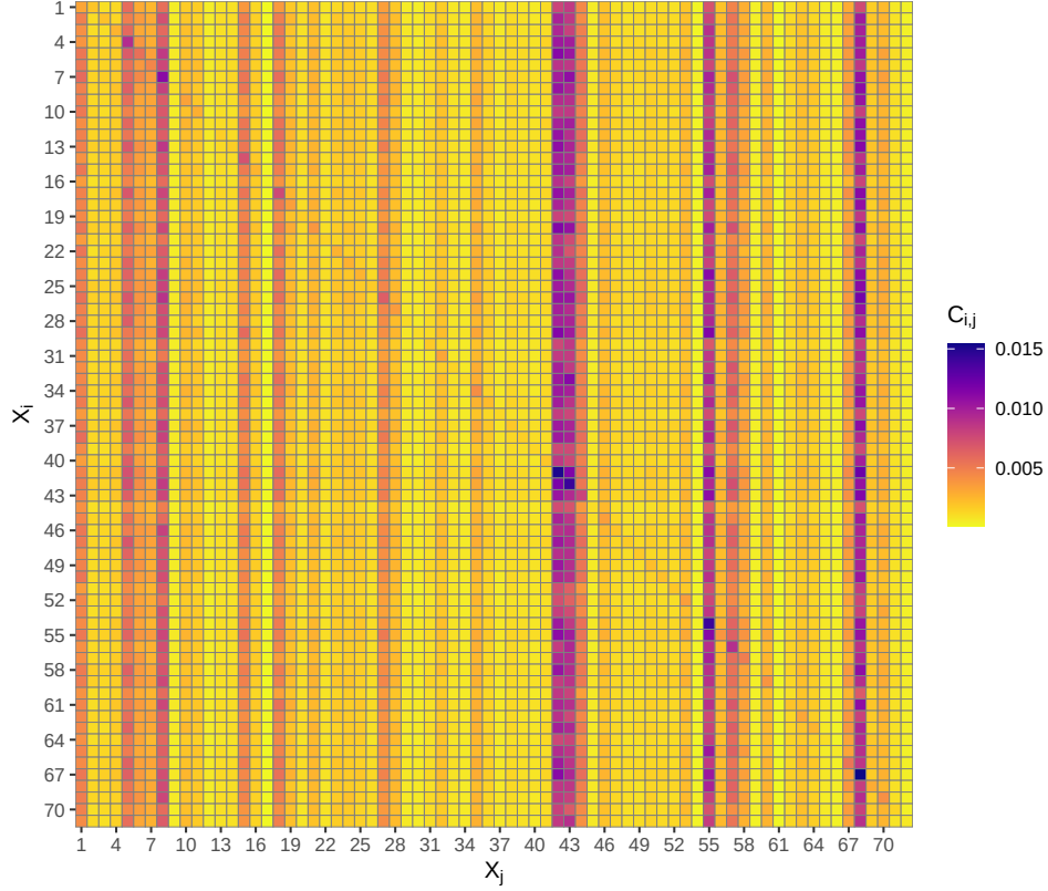
Figure 5: Heatmap of the decomposition of the cascade sensitivities \mathcal{C}_{i,j} , i, j = 1, \dots, n . Rows correspond to input factors that are stressed, while columns correspond to the (indirect) contributions of other inputs factors.
