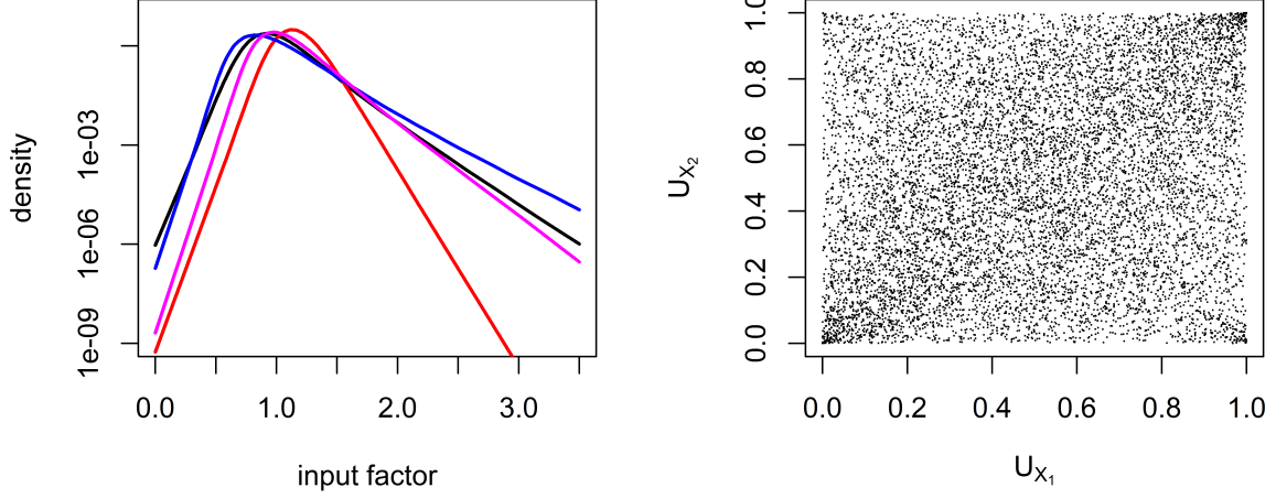
Figure 3: Left: estimated densities of input factors X_1, \dots, X_4 . Right: scatter plot of U_{X_2} against U_{X_1} .
