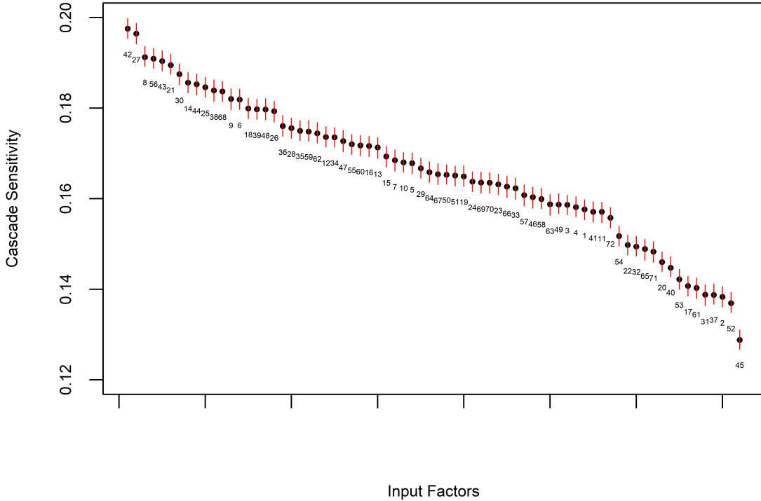
Figure 4: Importance ranking of cascade sensitivities of all 72 risk factors, with respect to a proportional stress on the t-transformed input factors. The red lines represent 90% confidence intervals.
