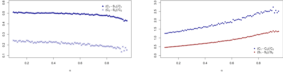
Figure 2: Sensitivities for the ES_{0.9} . Left: (C_i - S_i)/C_i , for i = 1 (triangles) and i = 2 (crosses), against different levels of tail-stresses \alpha , with t_i = F_i^{-1}(\alpha) . Right: (C_1 - C_2)/C_2 (blue) and (S_1 - S_2)/S_2 (red) against different levels of tail-stresses \alpha .
