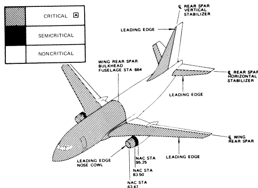
Figure 3. Aerodynamic Smoothness Critical Areas
