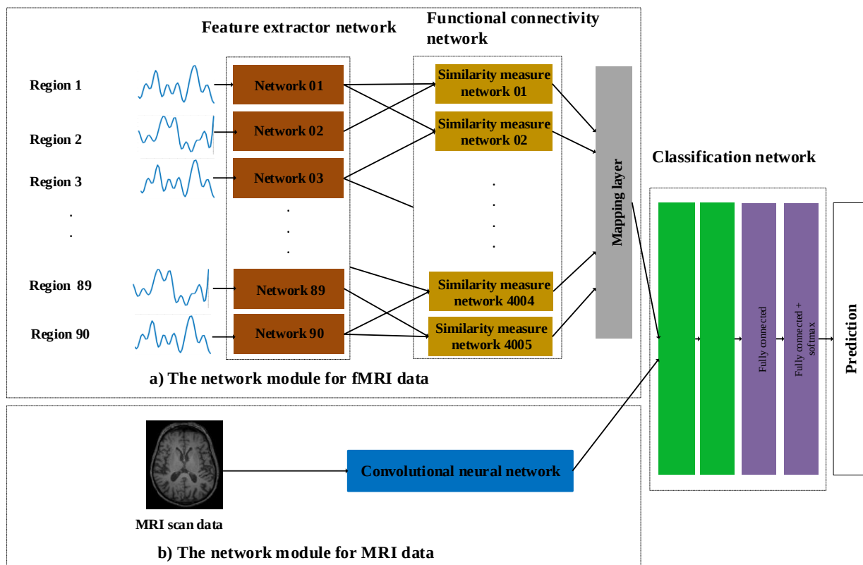
Fig. 8.1 A possible extension for fusion of multiple imaging modalities. The network (a) is for fMRI data, which is the same as proposed in this dissertation and the network (b) is for MRI data.
