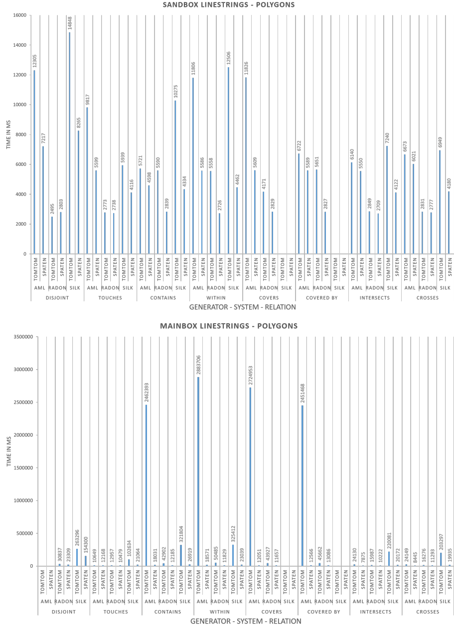
Fig. 3. Time performance for TomTom & Spaten SLP (top) and LLP (bottom) suites for AML (A), Silk (S) and RADON (R).
